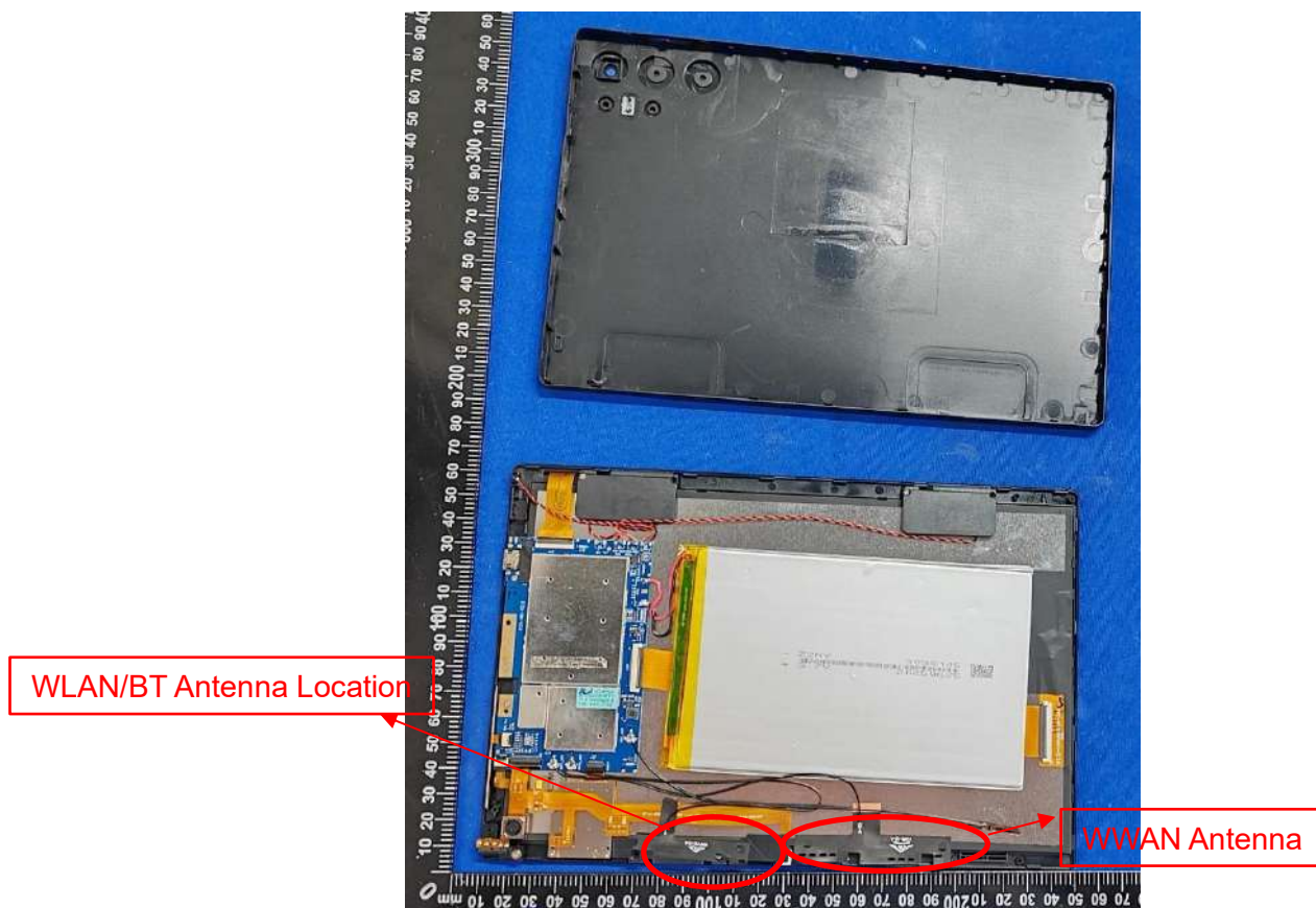
Top side (Back view)
