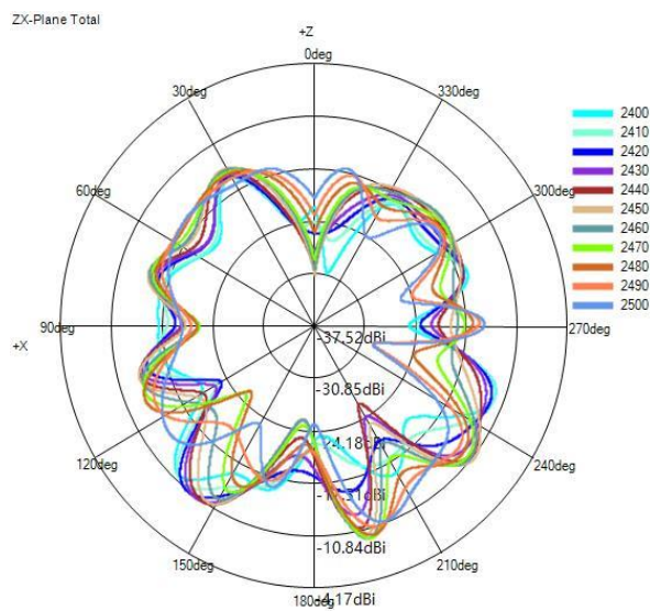
(1) X-Z Plane(unit:dBi):
