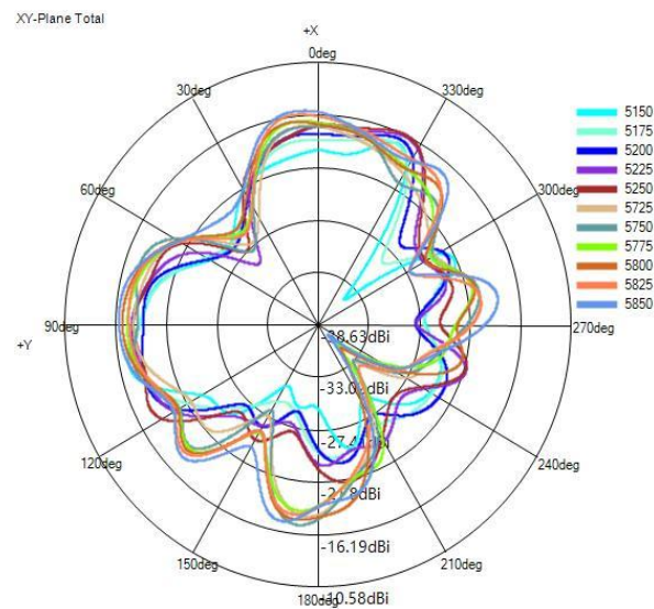
(3) X-Y Plane(unit:dBi):
