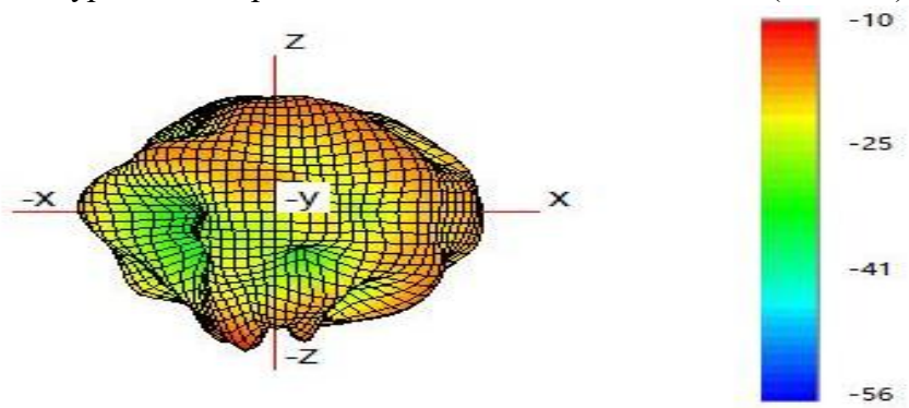
(4) Typical Free Space 3D Radiation Pattern at 5.8GHz(unit:dBi):
