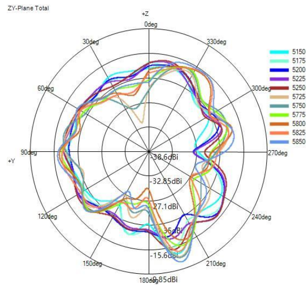
(2) Y-Z Plane(unit:dBi):
