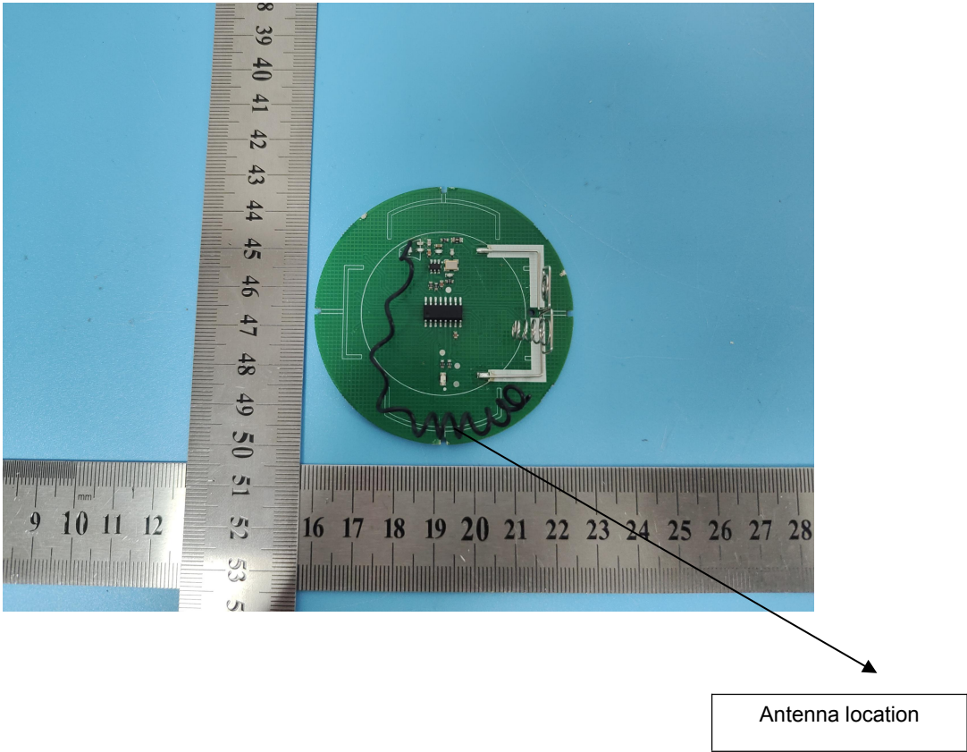
INTERNAL PHOTO OF SAMPLE PCB
