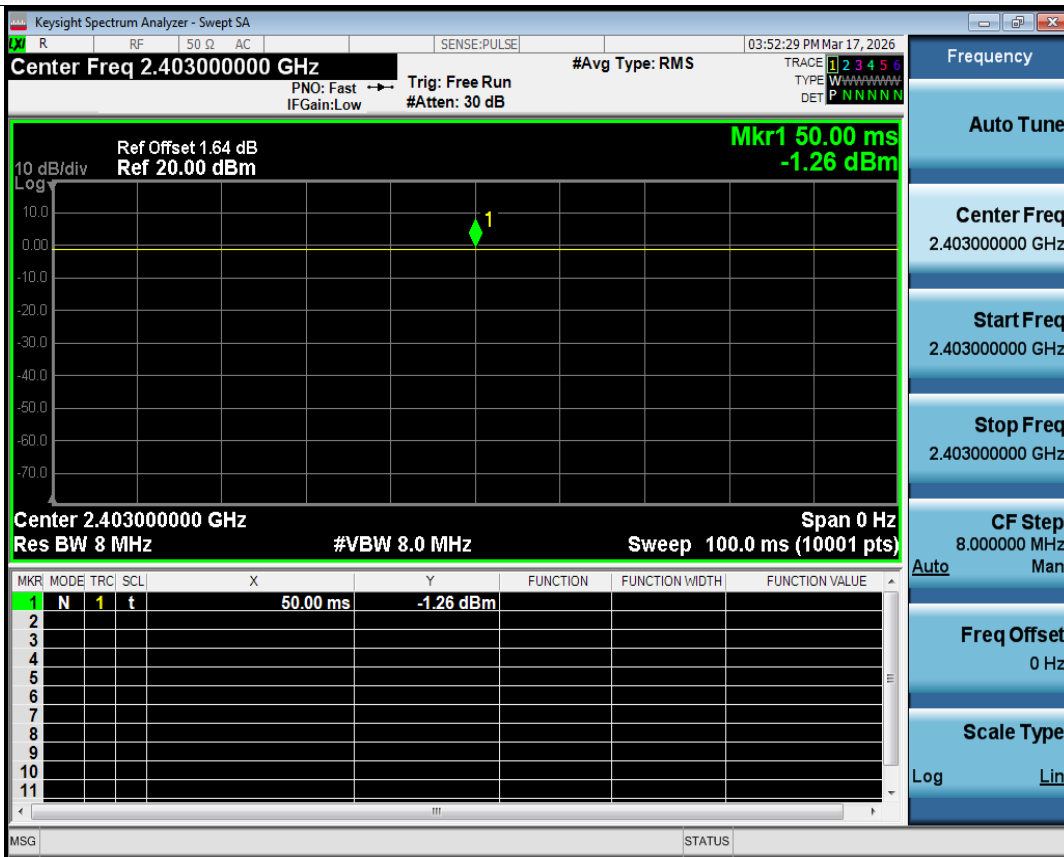
Duty Cycle NVNT 2.4G 2403MHz Ant1
