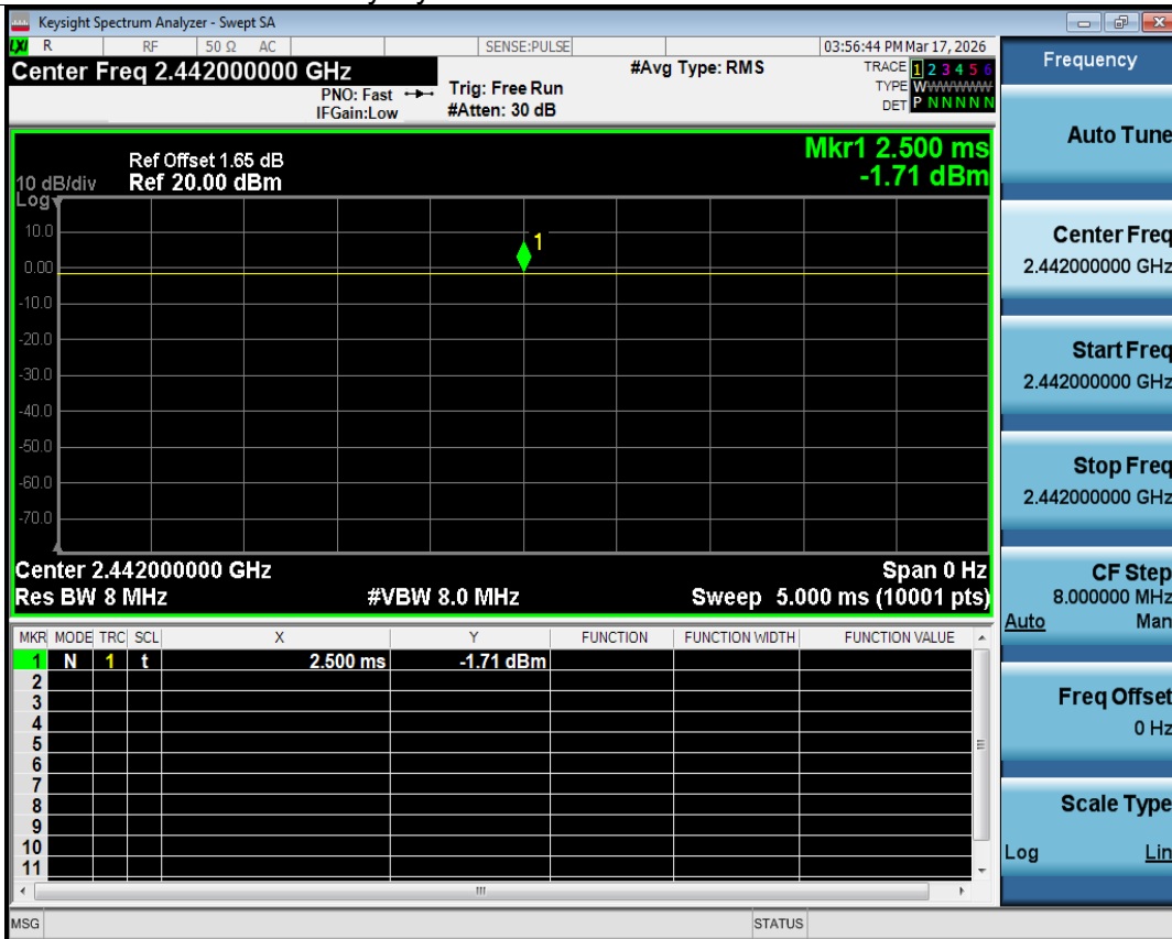
Duty Cycle NVNT 2.4G 2442MHz Ant1
