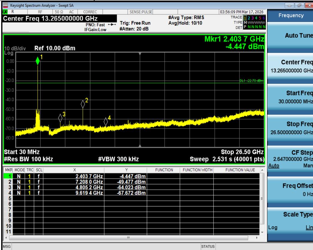
Tx. Spurious NVNT 2.4G 2403MHz Ant1 Emission
