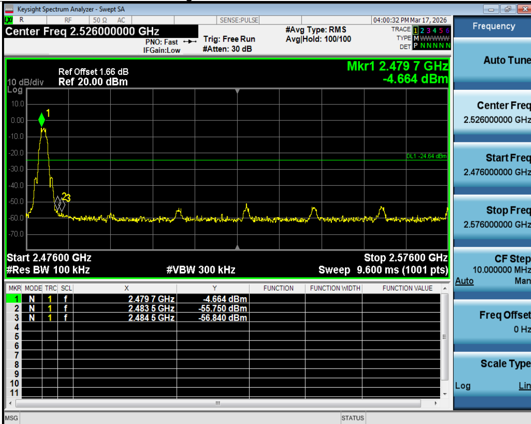
Band Edge NVNT 2.4G 2480MHz Ant1 Emission
