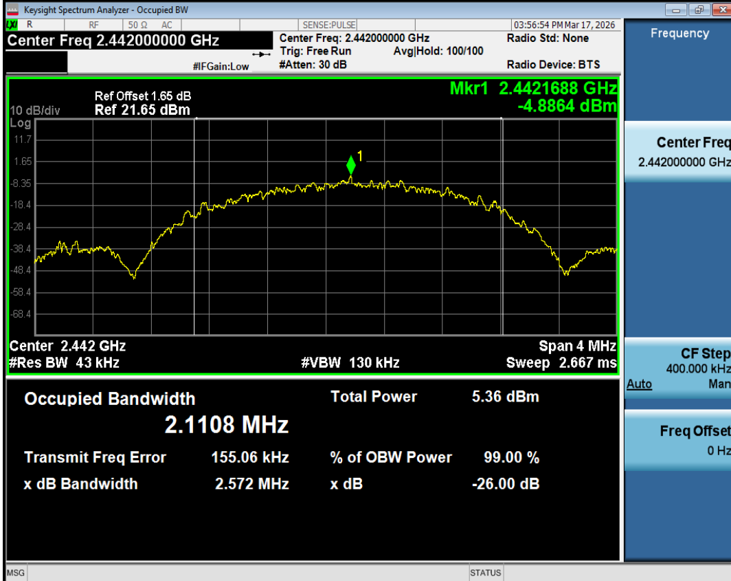
OBW NVNT 2.4G 2442MHz Ant1
