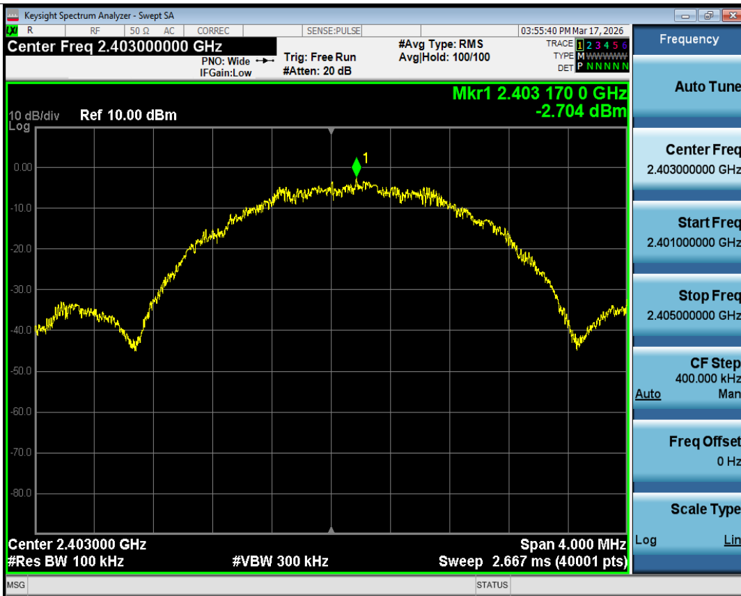
Tx. Spurious NVNT 2.4G 2403MHz Ant1 Ref
