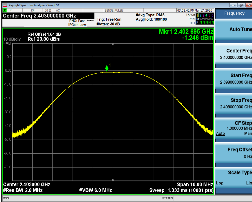
Peak Power NVNT 2.4G 2403MHz Ant1
