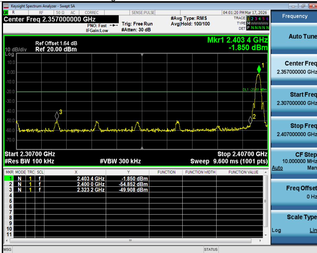
Band Edge NVNT 2.4G 2403MHz Ant1 Emission
