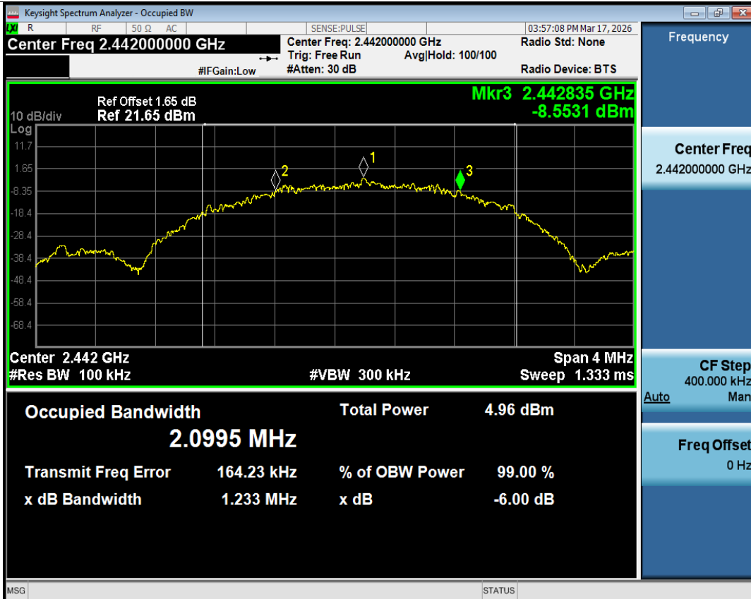
-6dB Bandwidth NVNT 2.4G 2442MHz Ant1
