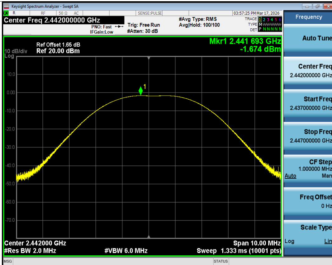
Peak Power NVNT 2.4G 2442MHz Ant1
