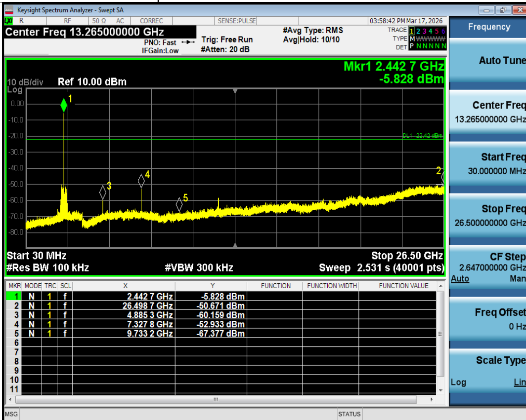
Tx. Spurious NVNT 2.4G 2442MHz Ant1 Emission
