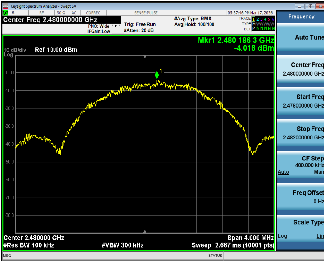
Tx. Spurious NVNT 2.4G 2480MHz Ant1 Ref
