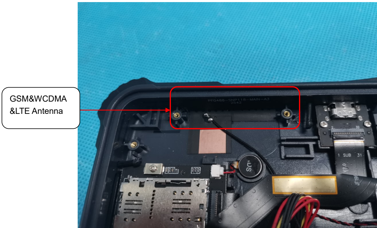
Internal View-5 of EUT
