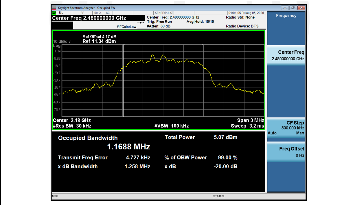
-20dB_Bandwidth_NVNT_ANT1_2-DH1_2480_00
