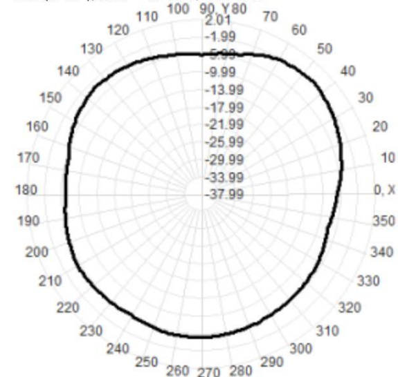
Total(H-XY), Max= -1.71dBi, CirD=6.39
