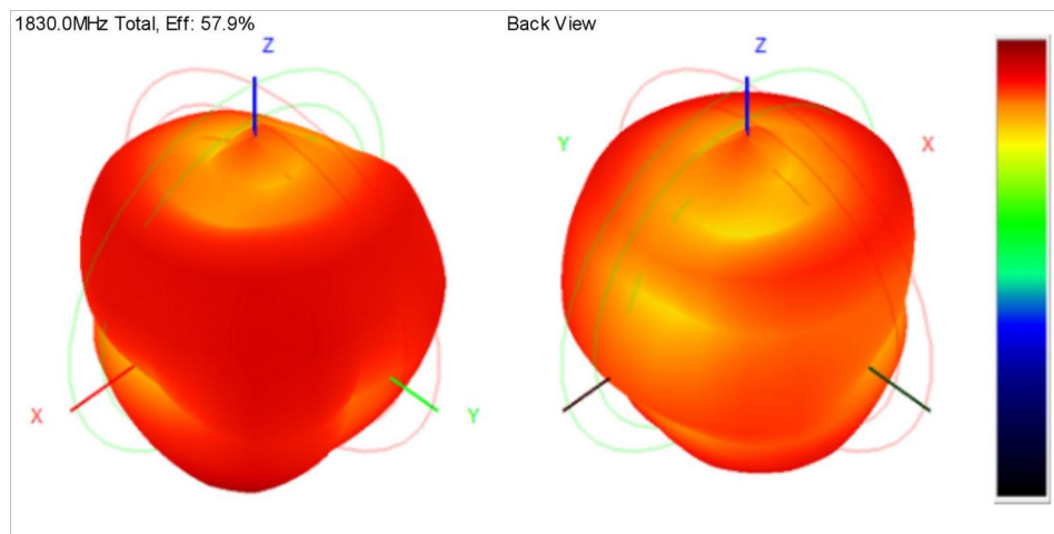
3D radiation pattern diagram
