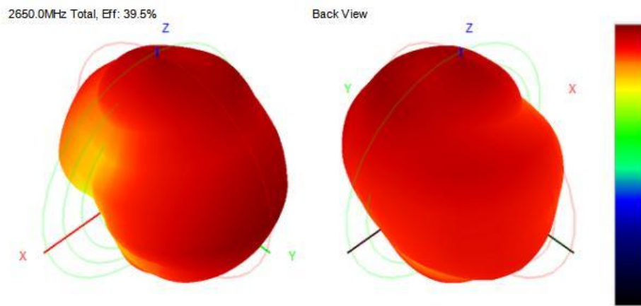
3D radiation pattern diagram
