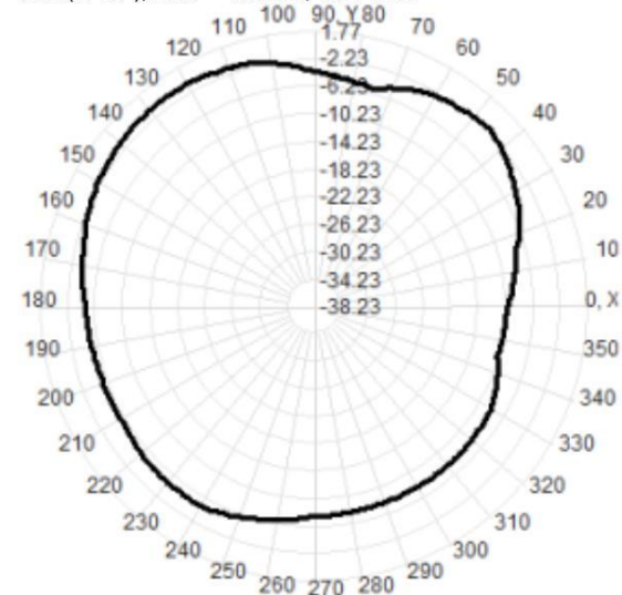
Total(H-XY), Max=-1.00dBi, CirD=9.67
