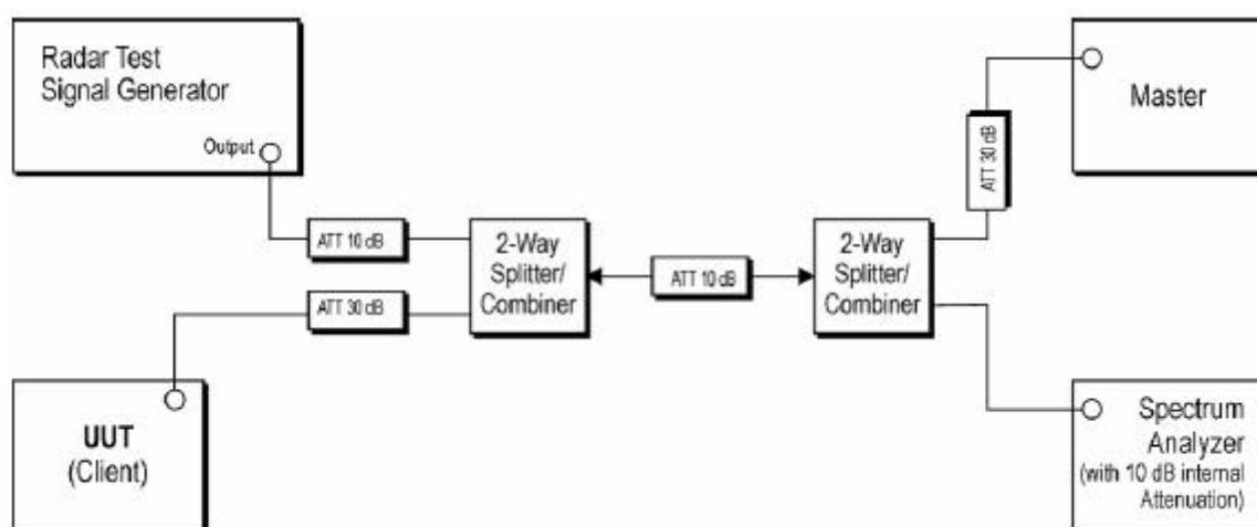
Example Conducted Setup where UUT is a Client and Radar Test Waveforms are injected into the Client.
