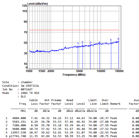
BLE_1M_TX_CH_00_Vertical-Peak
