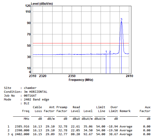
BLE_1M_TX_CH_00_Horizontal-Avg
