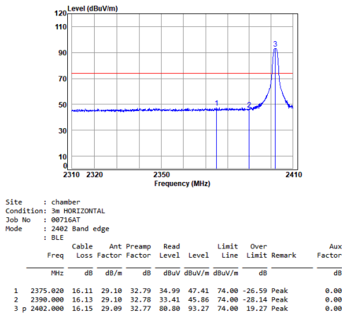
BLE_1M_TX_CH_00_Horizontal-Peak
