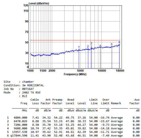
BLE_1M_TX_CH_00_Horizontal-Avg
