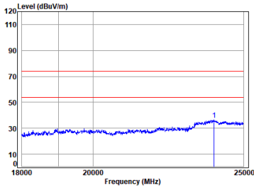
BLE 1M_TX_CH_M_Vertical
