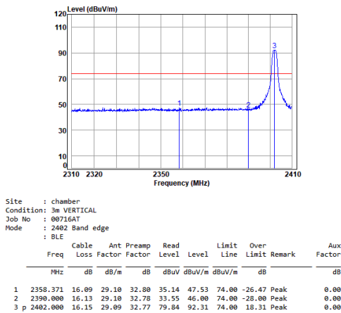
BLE_1M_TX_CH_00_Vertical-Peak
