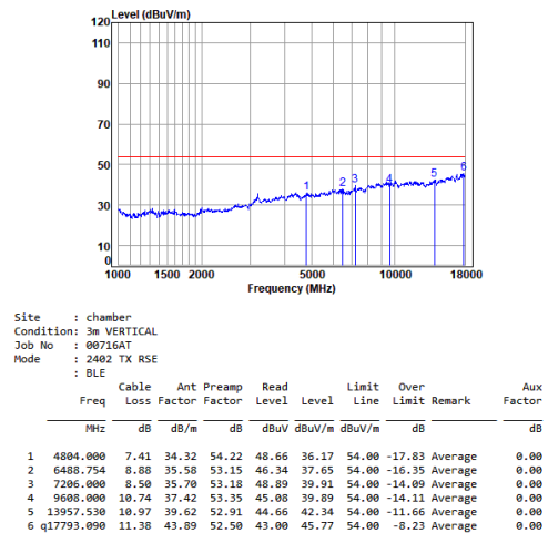
BLE_1M_TX_CH_00_Vertical-Avg
