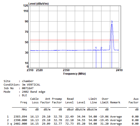
BLE_1M_TX_CH_00_Vertical-Avg
