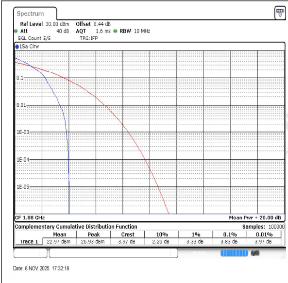
Band2-10MHz-QPSK-18900-PASS
