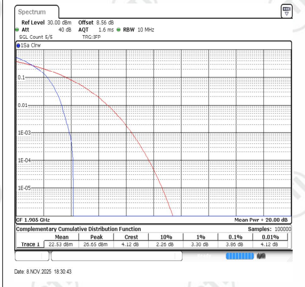
Band2-10MHz-16QAM-19150-PASS
