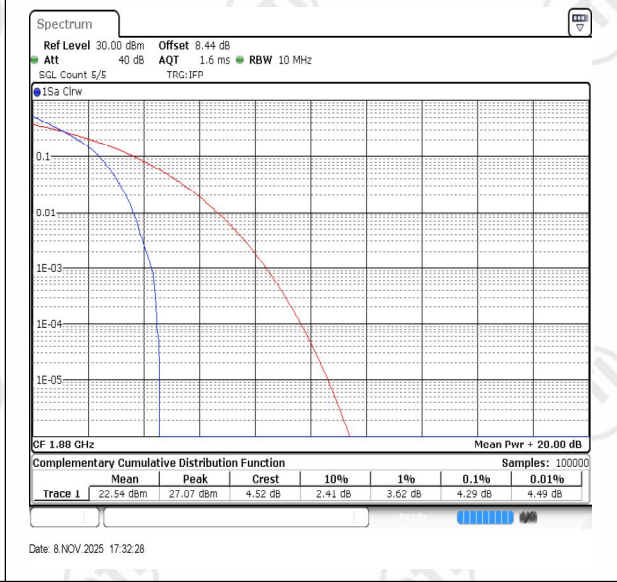
Band2-10MHz-16QAM-18900-PASS
