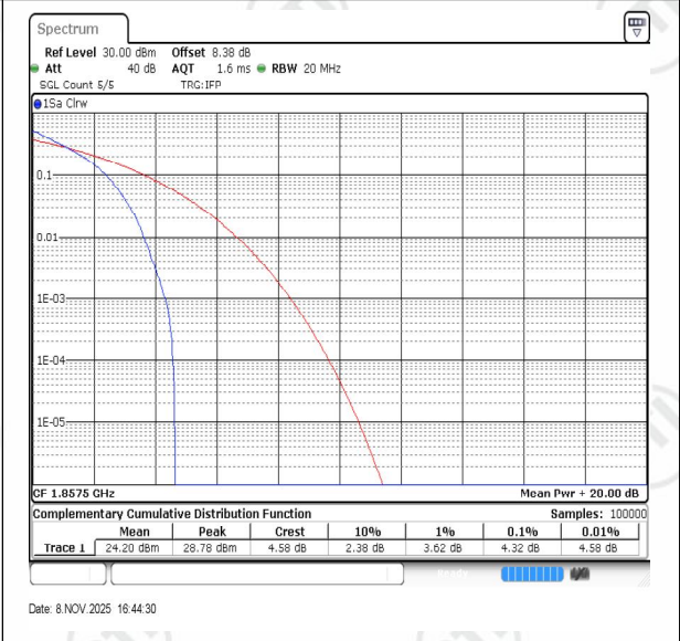
Band2-15MHz-16QAM-18675-PASS
