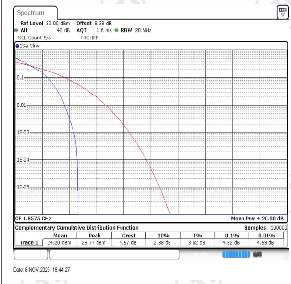
Band2-15MHz-QPSK-18675-PASS
