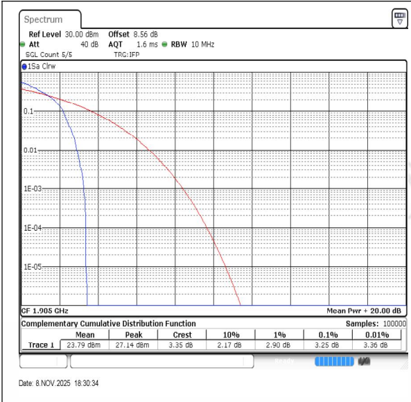
Band2-10MHz-QPSK-19150-PASS
