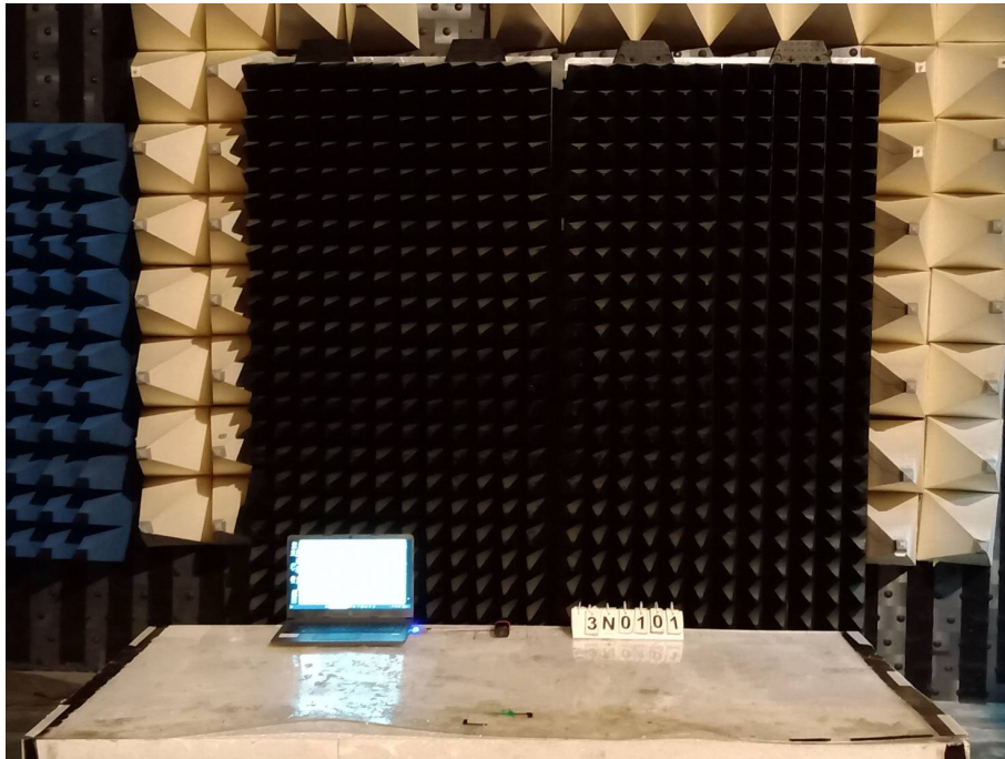
01. RADIATED BAND EDGE Front View(1GHz below)
