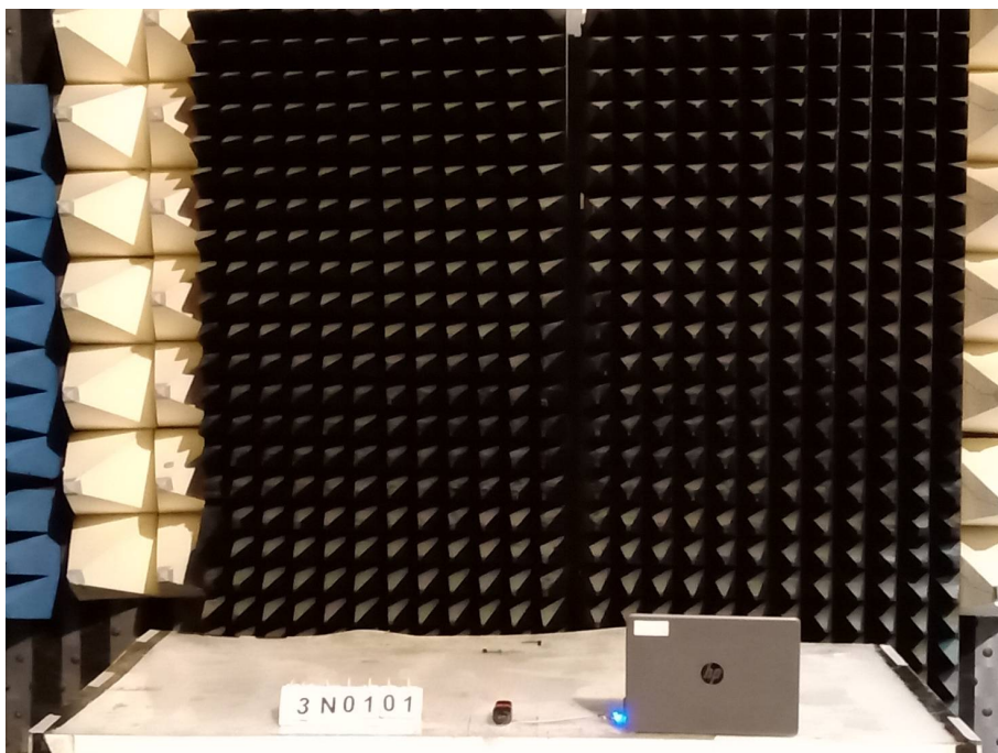
02. RADIATED BAND EDGE Rear View(1GHz below)
