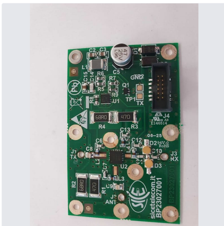
Photo 20 RF Switch Board top
