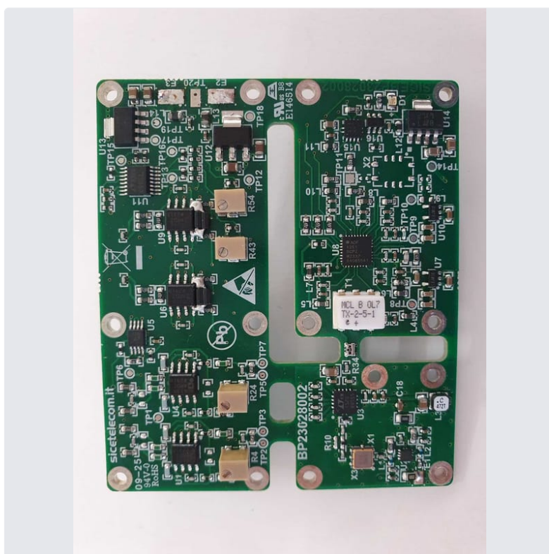
Photo 8 Down Converter Board top
