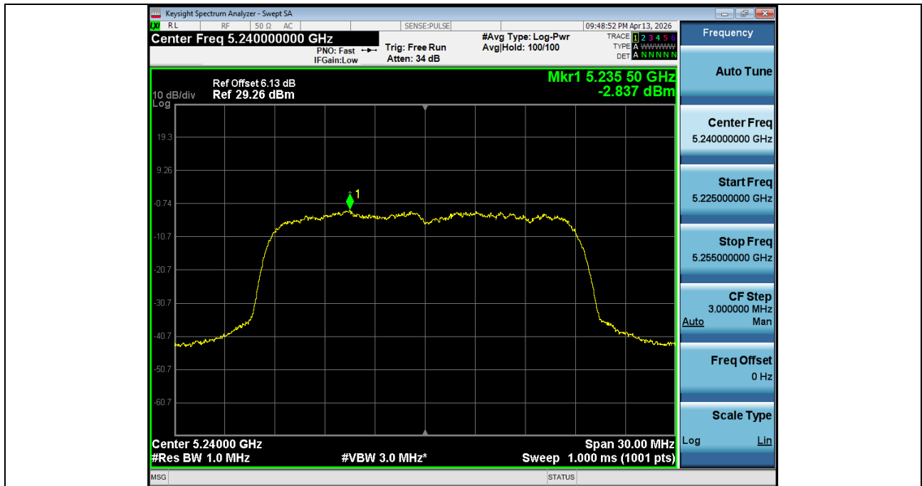
Power_Spectral_Density_NVNT_ANT2_802_11n(HT20)_5240
