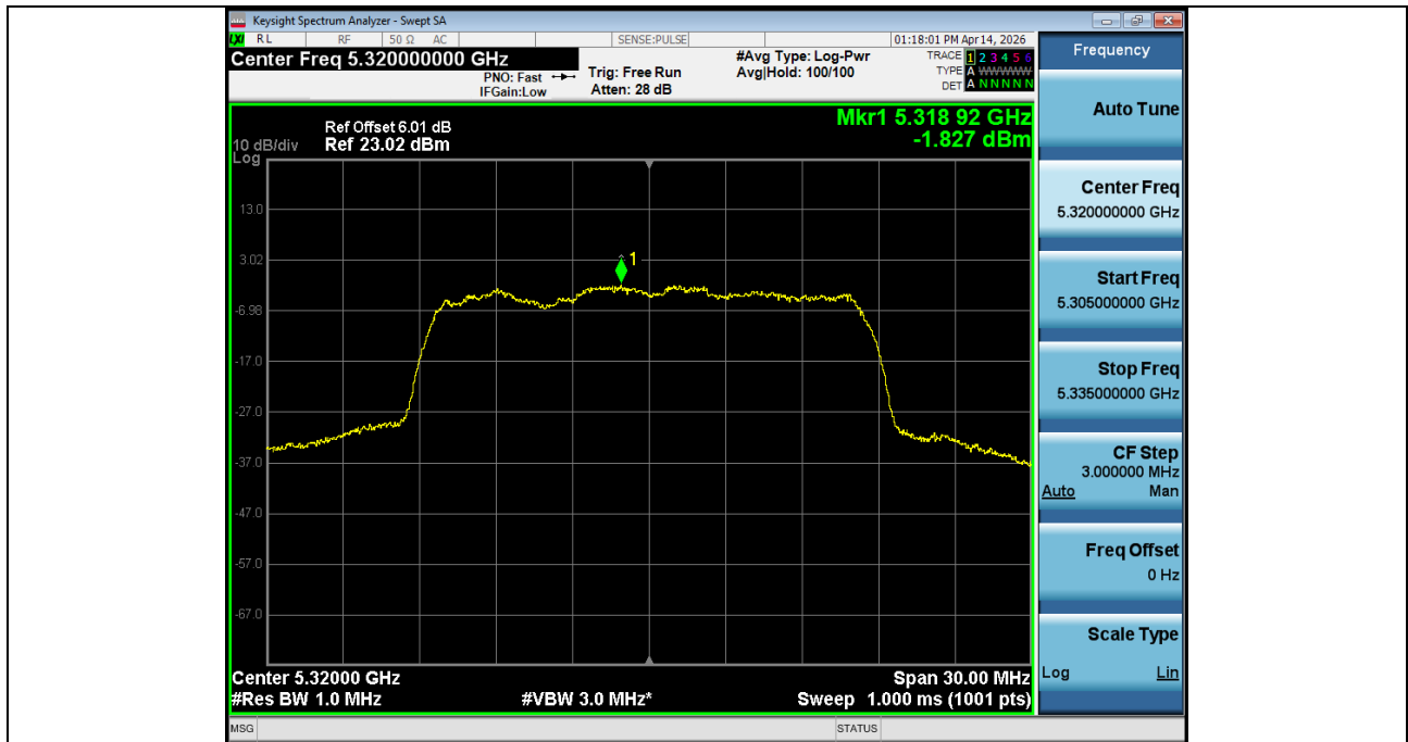
Power_Spectral_Density_NVNT_ANT2_802_11a_5320
