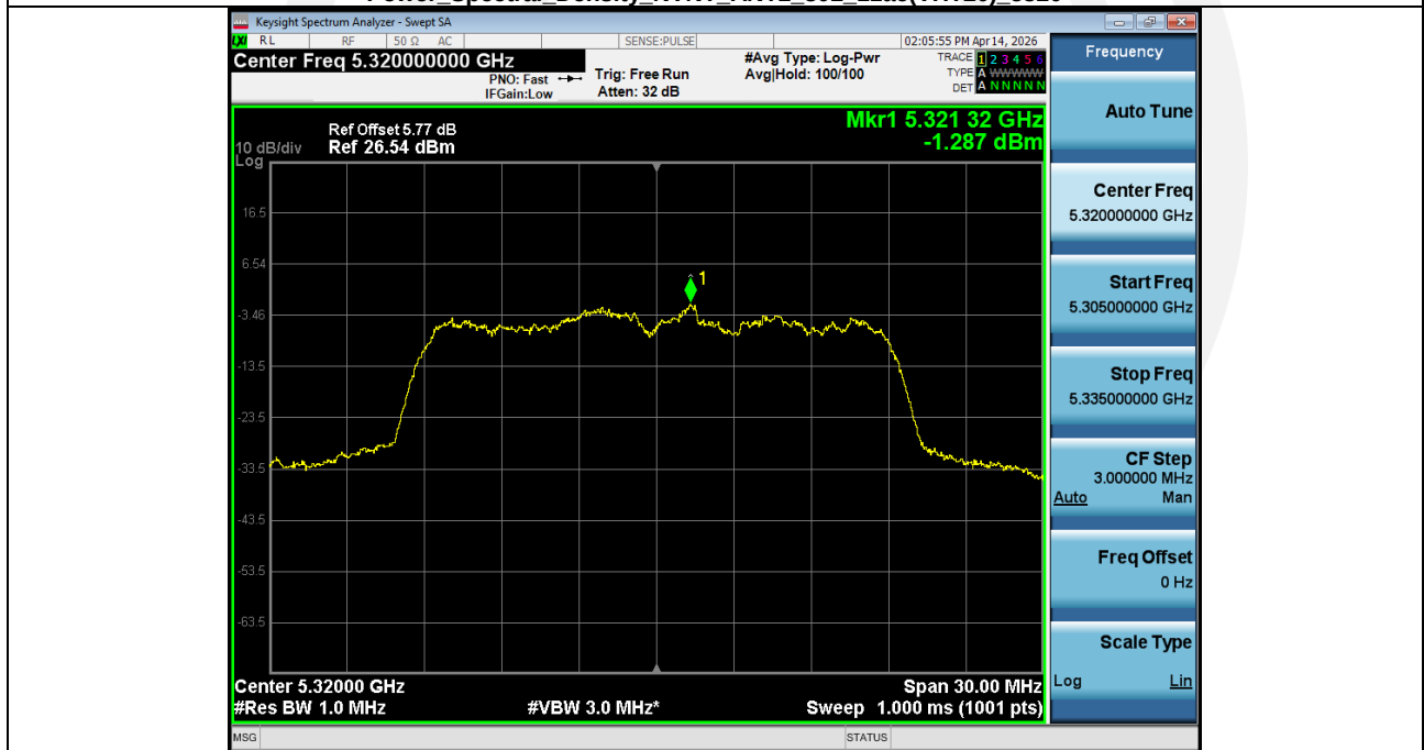
Power_Spectral_Density_NVNT_ANT2_802_11ac(VHT20)_5320
