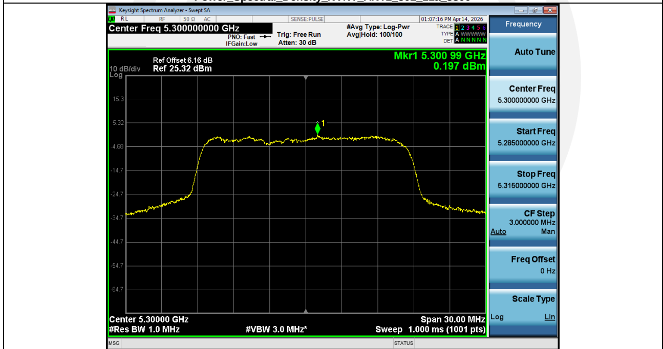
Power_Spectral_Density_NVNT_ANT2_802_11a_5300
