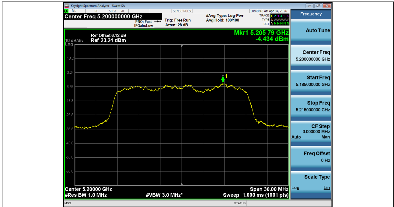
Power_Spectral_Density_NVNT_ANT2_802_11ac(VHT20)_5200
