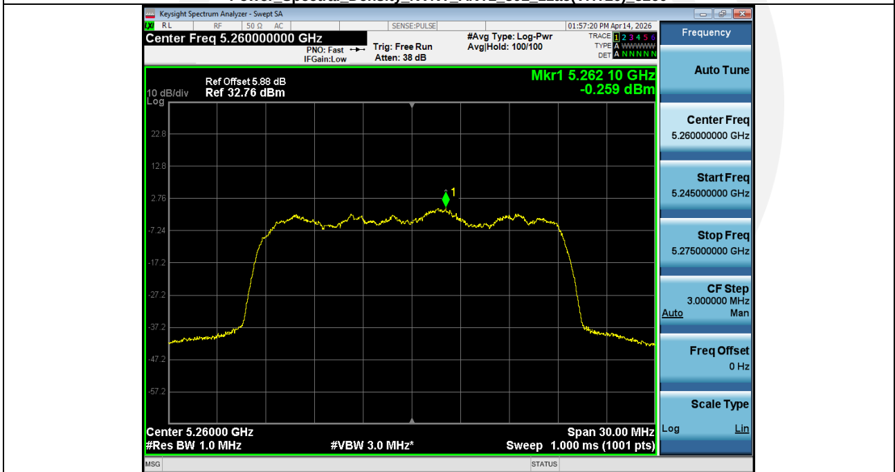
Power Spectral Density_NVNT_ANT2_802_11ac(VHT20)_5260
