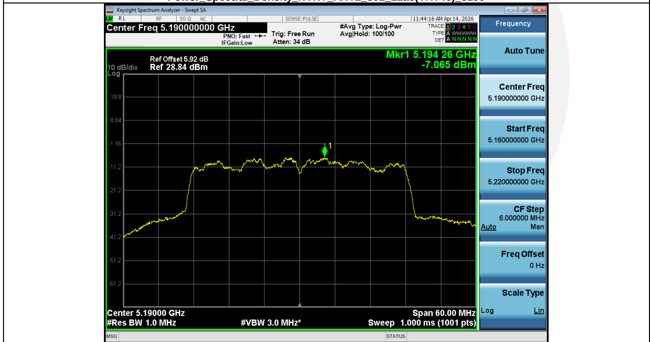
Power_Spectral_Density_NVNT_ANT2_802_11ac(VHT40)_5190
