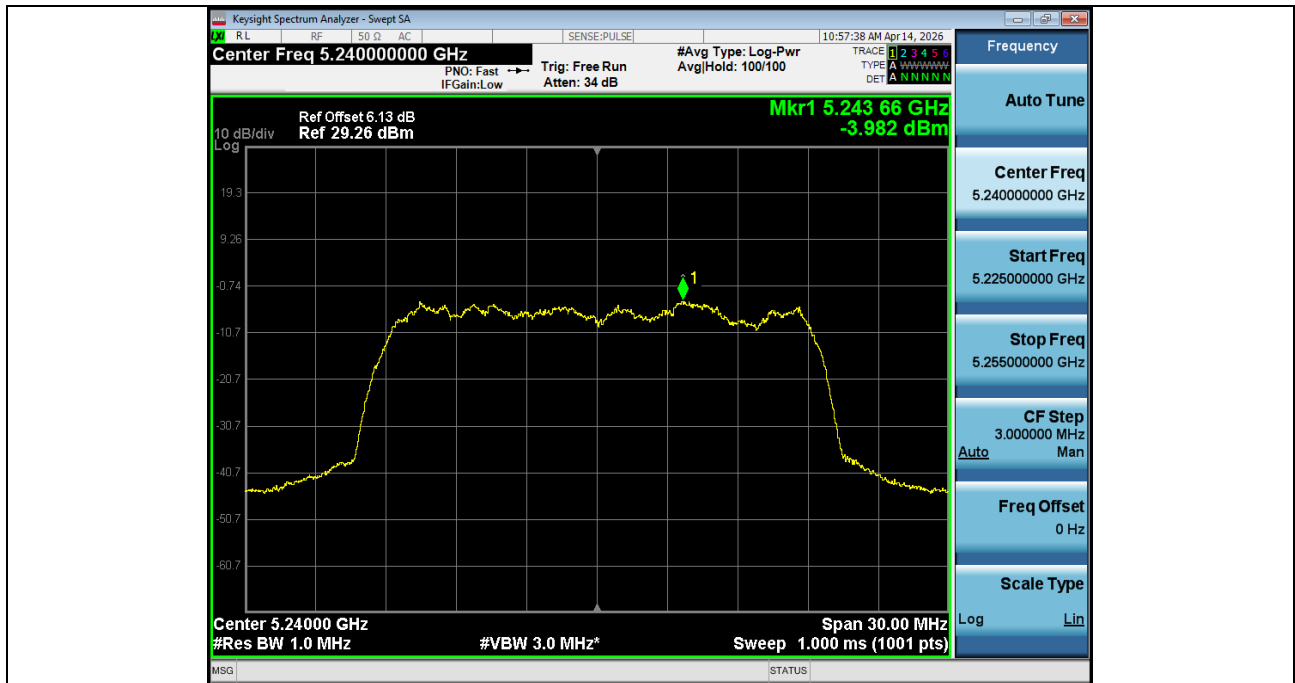
Power_Spectral_Density_NVNT_ANT2_802_11ac(VHT20)_5240
