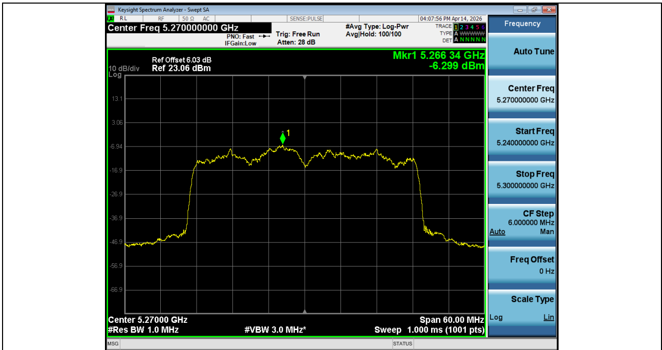
Power_Spectral_Density_NVNT_ANT2_802_11n(HT40)_5270
