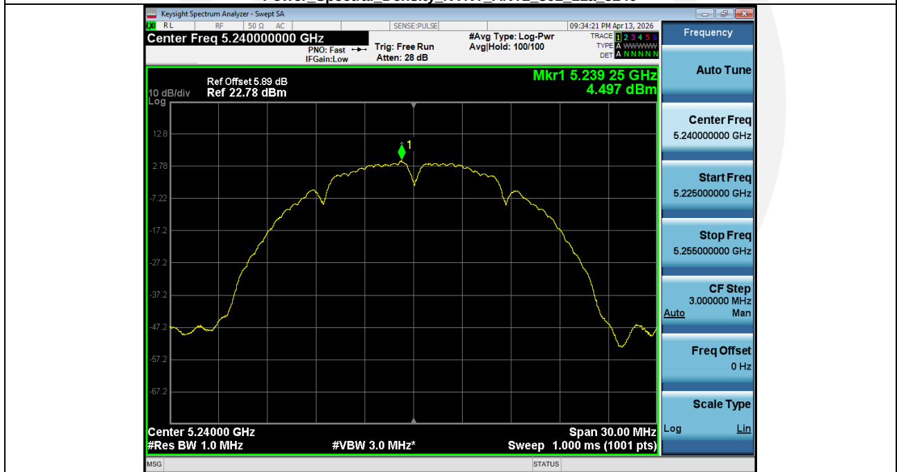
Power_Spectral_Density_NVNT_ANT2_802_11a_5240
