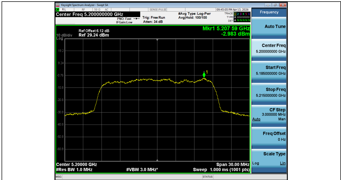
Power_Spectral_Density_NVNT_ANT2_802_11n(HT20)_5200
