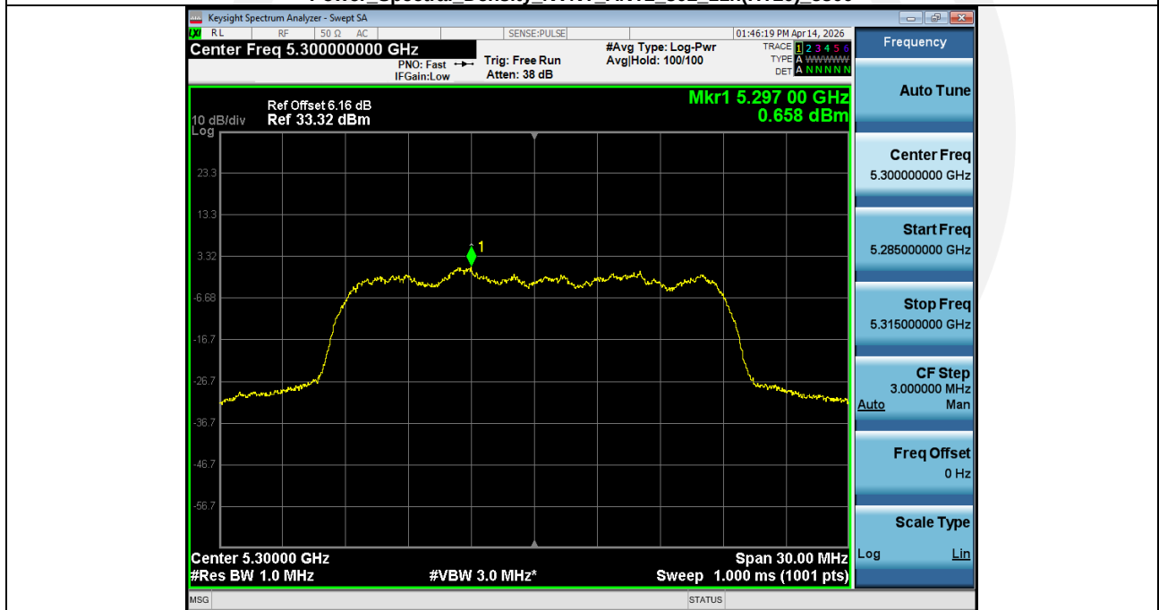
Power_Spectral_Density_NVNT_ANT2_802_11n(HT20)_5300
