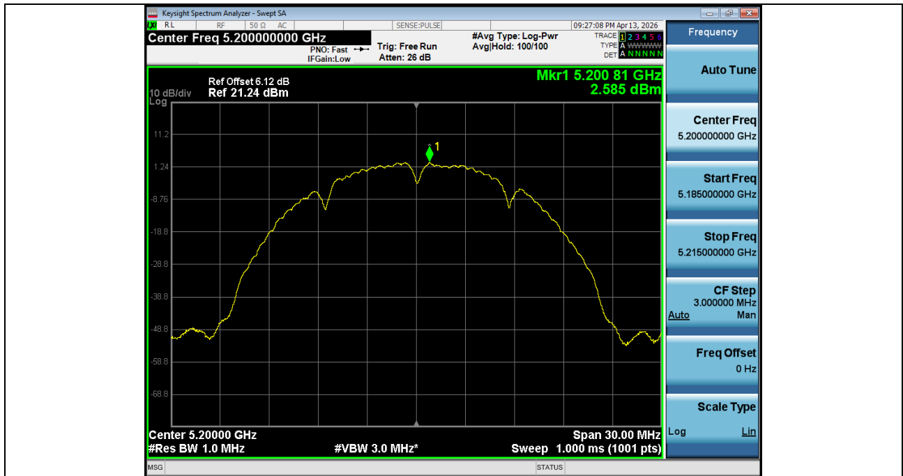
Power_Spectral_Density_NVNT_ANT2_802_11a_5200
