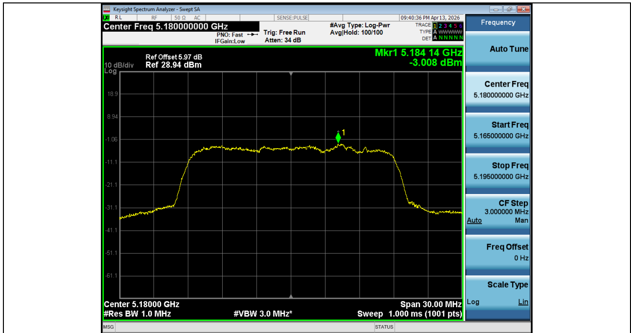
Power_Spectral_Density_NVNT_ANT2_802_11n(HT20)_5180
