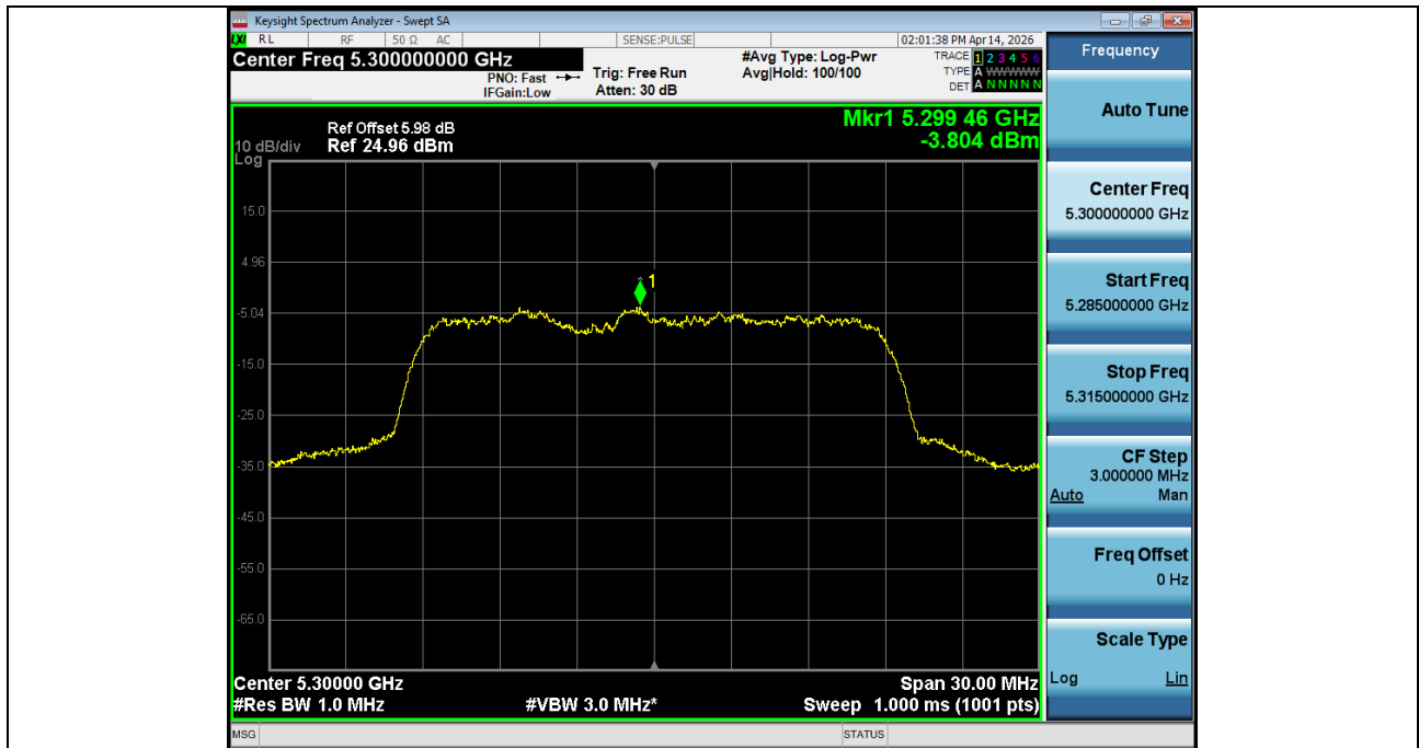
Power_Spectral_Density_NVNT_ANT2_802_11ac(VHT20)_5300
