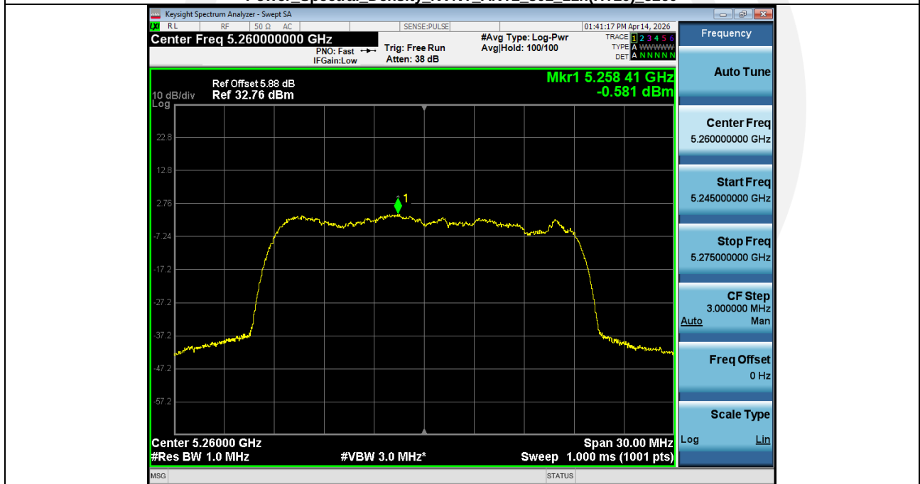
Power_Spectral_Density_NVNT_ANT2_802_11n(HT20)_5260
