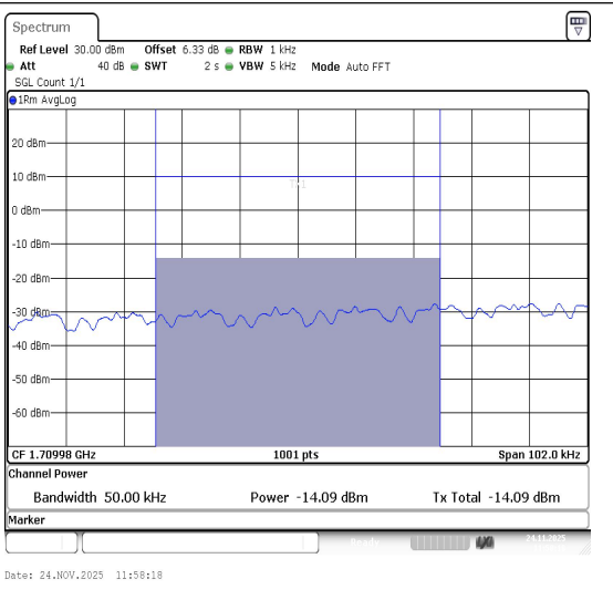
Band66-5MHz-QPSK-131997-1RB#0-PASS_Final1
