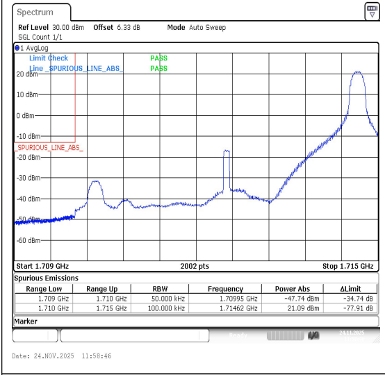
Band66-5MHz-QPSK-131997-1RB#24-PASS
