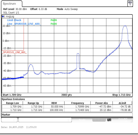
Band66-5MHz-16QAM-131997-1RB#24-PASS
