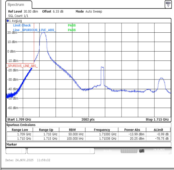
Band66-5MHz-16QAM-131997-1RB#0-PASS
