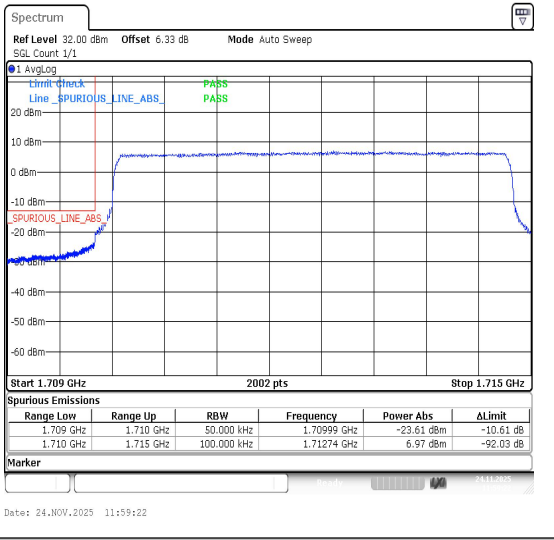
Band66-5MHz-QPSK-131997-25RB#0-PASS
