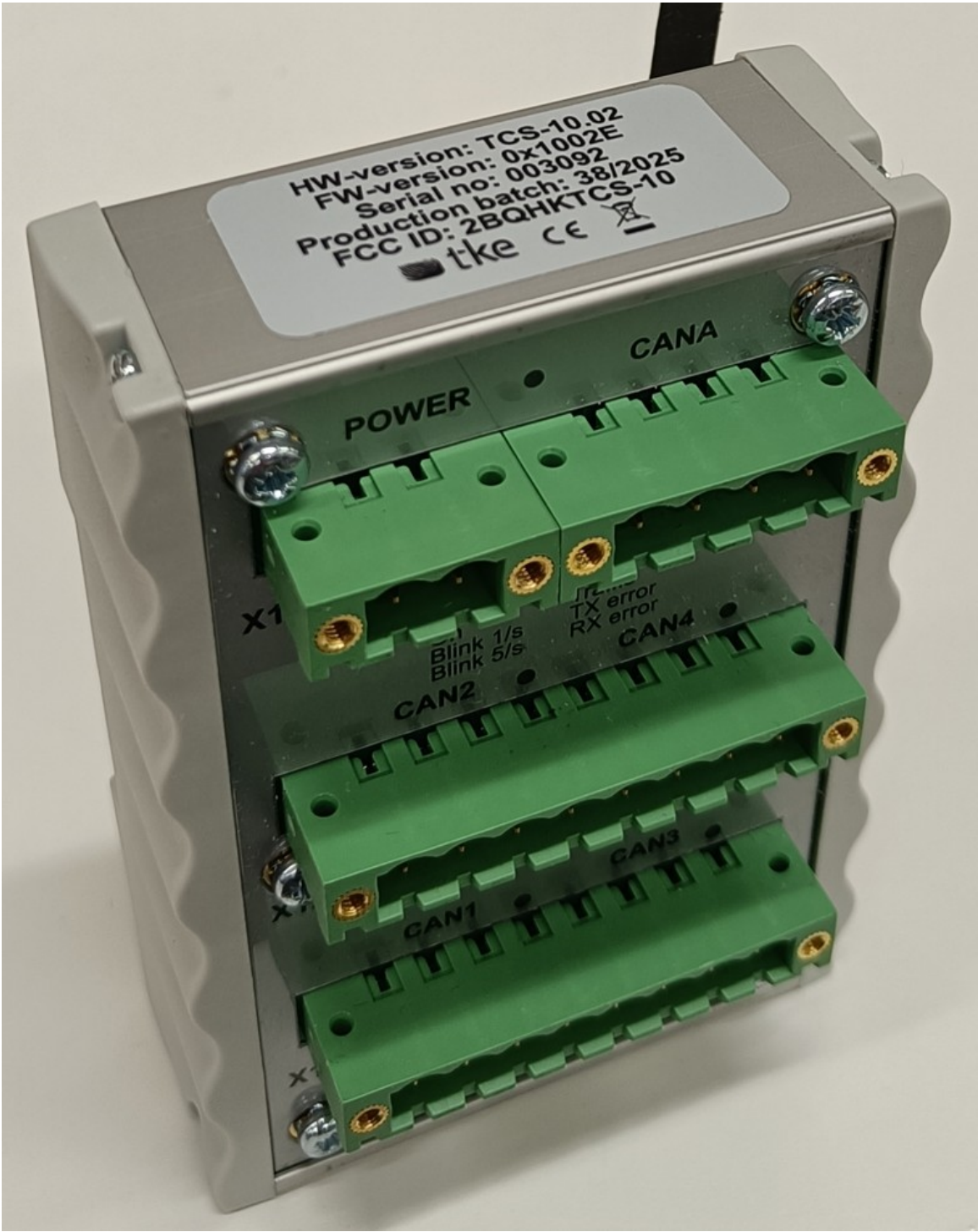
Device label
