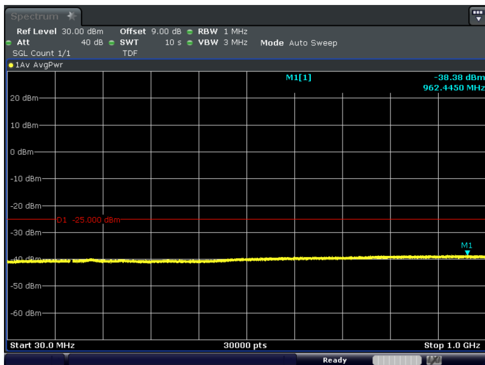
Test_Graph_band38_2595MHz_10M_QPSK_50RB#LOW_30M_1G_TX
