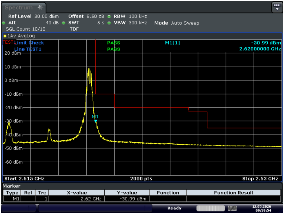
Test_Graph_band38_2617.5MHz_5M_16QAM_1RB#HIGH_Band edge
