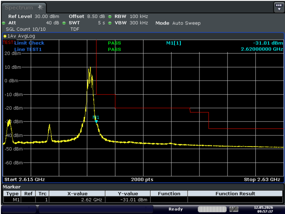
Test_Graph_band38_2617.5MHz_5M_QPSK_1RB#HIGH_Band edge
