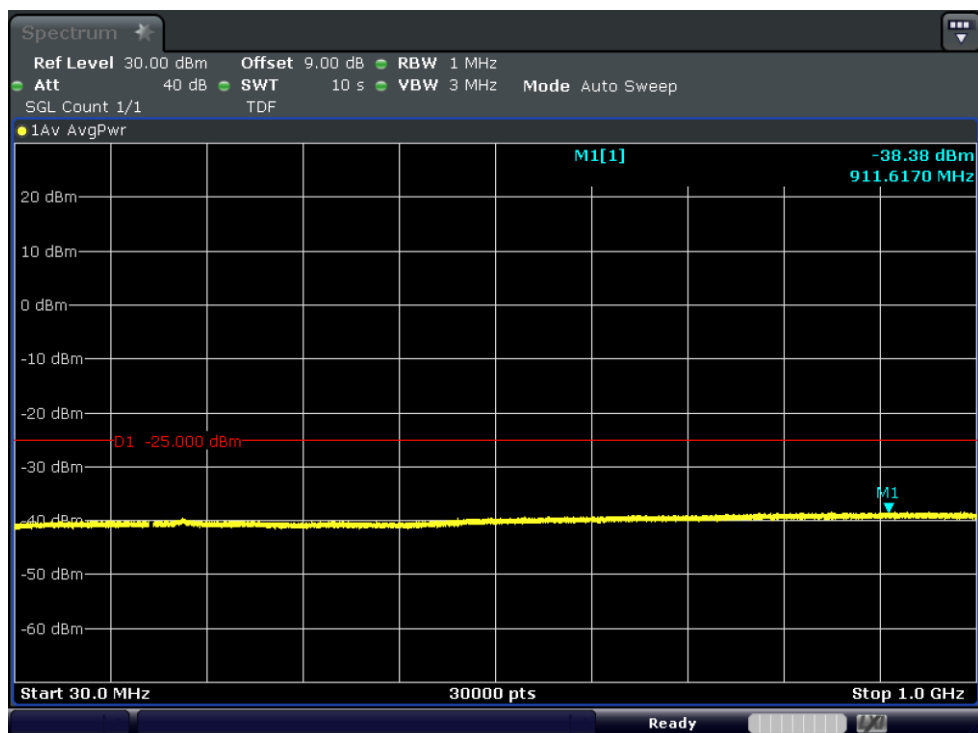
Test_Graph_band38_2617.5MHz_5M_QPSK_25RB#LOW_30M_1G_TX
