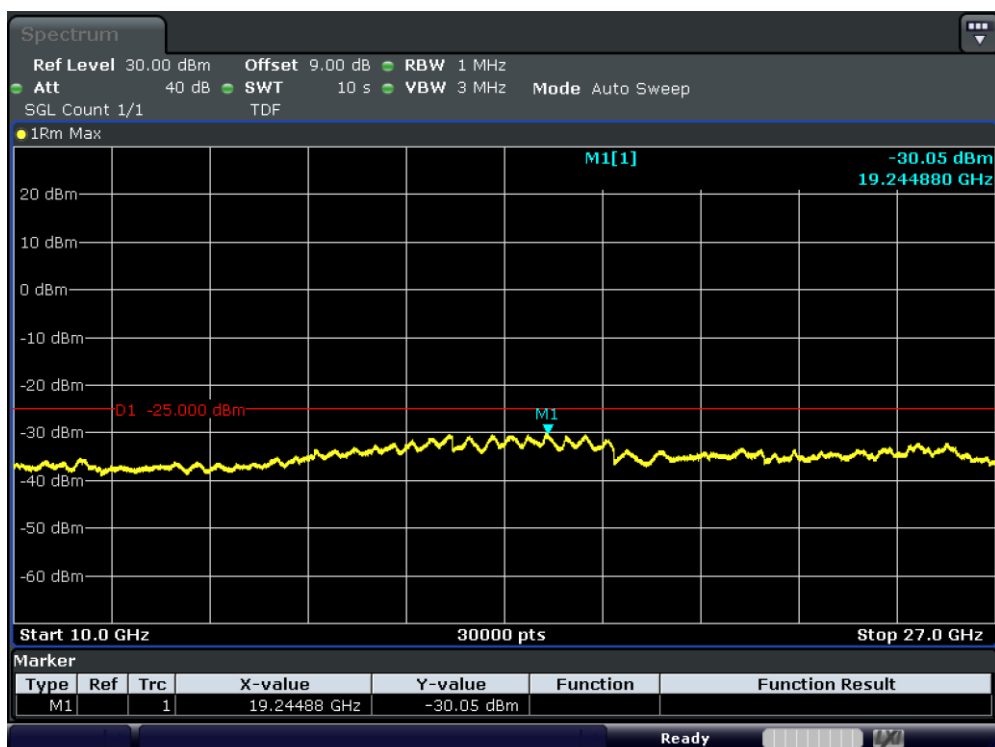
Test_Graph_band38_2612.5MHz_15M_QPSK_75RB#LOW_10G_27.0G_TX
