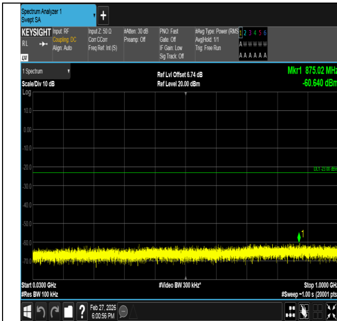
Band2-5MHz-QPSK-19175-25RB#0-30~1000-PASS
