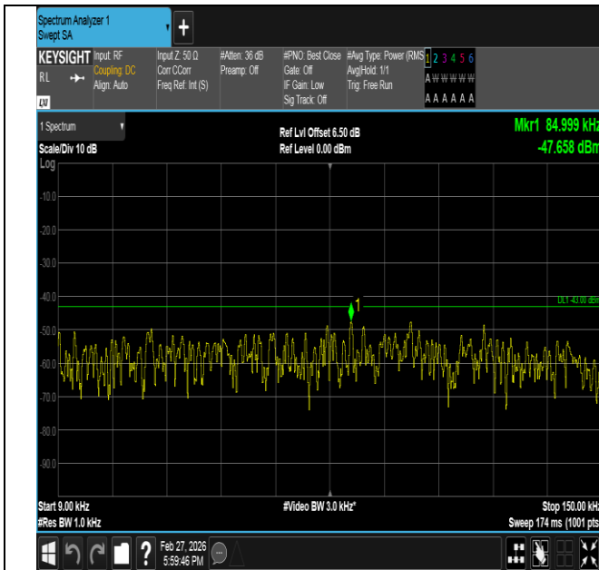
Band2-5MHz-16QAM-19175-1RB#24-0.009~0.15-PASS
