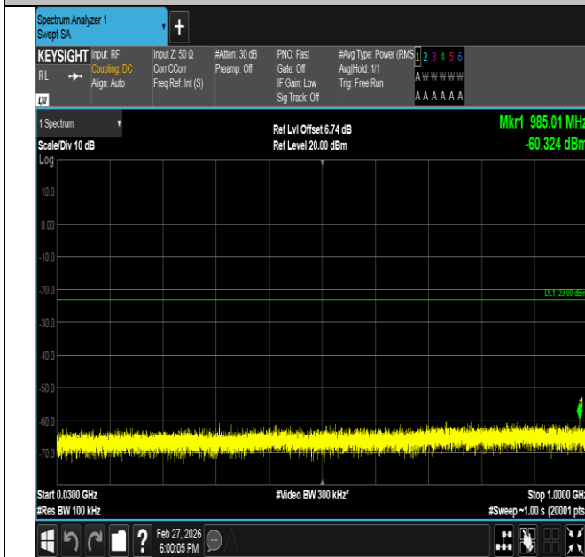
Band2-5MHz-16QAM-19175-1RB#24-30~1000-PASS
