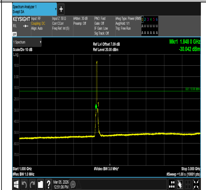
Band2-10MHz-QPSK-18650-50RB#0-1000~3000-PASS
