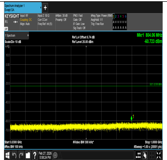
Band2-5MHz-16QAM-19175-1RB#0-30~1000-PASS
