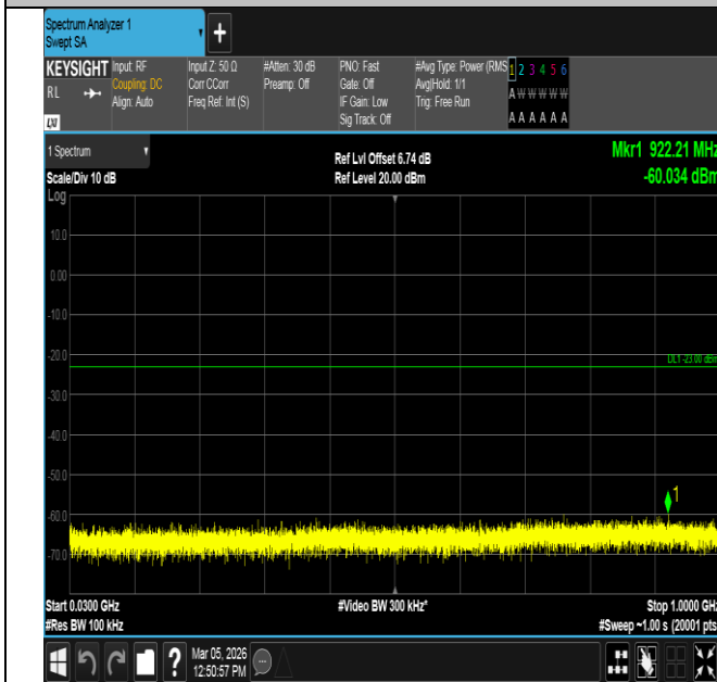
Band2-10MHz-QPSK-18650-50RB#0-30~1000-PASS
