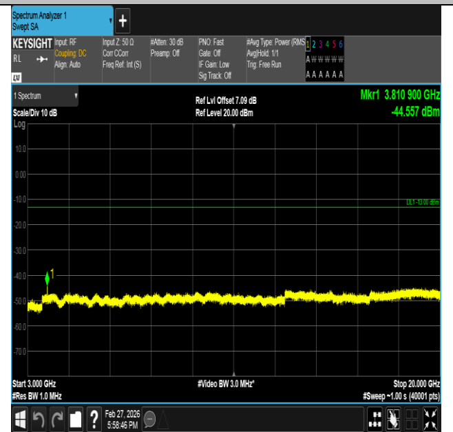
Band2-5MHz-16QAM-19175-1RB#0-3000~20000-PASS
