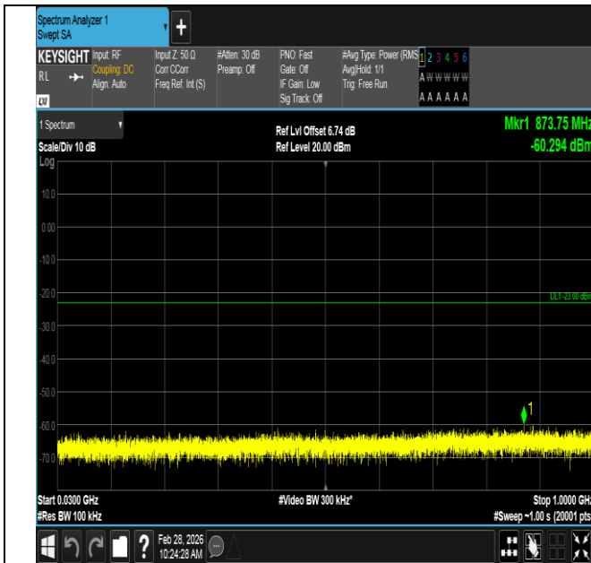
Band2-10MHz-QPSK-18650-1RB#0-30~1000-PASS
