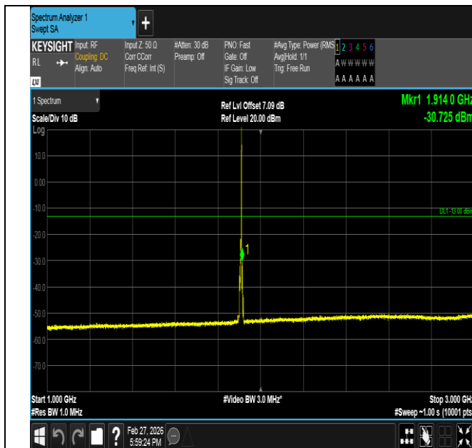
Band2-5MHz-QPSK-19175-1RB#24-1000~3000-PASS
