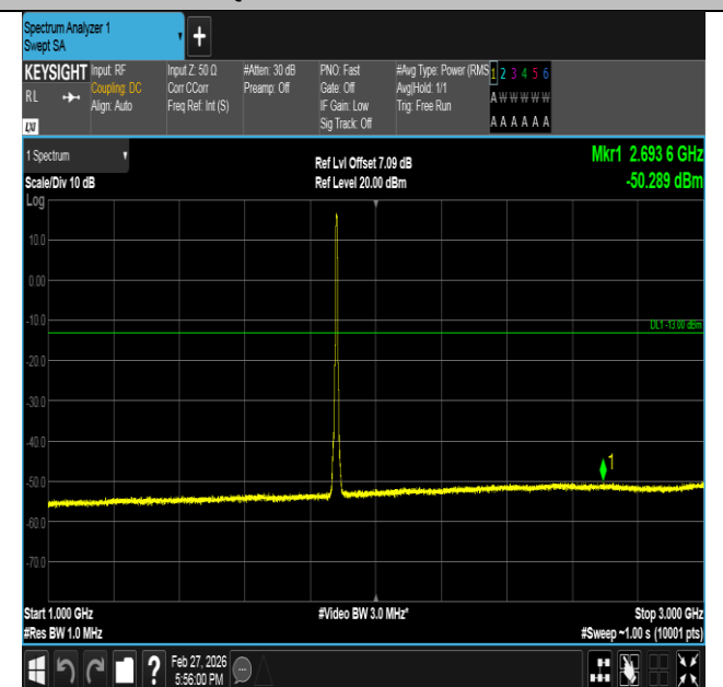
Band2-5MHz-QPSK-18900-25RB#0-1000~3000-PASS
