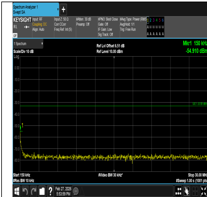
Band2-5MHz-QPSK-18900-1RB#24-0.15~30-PASS
