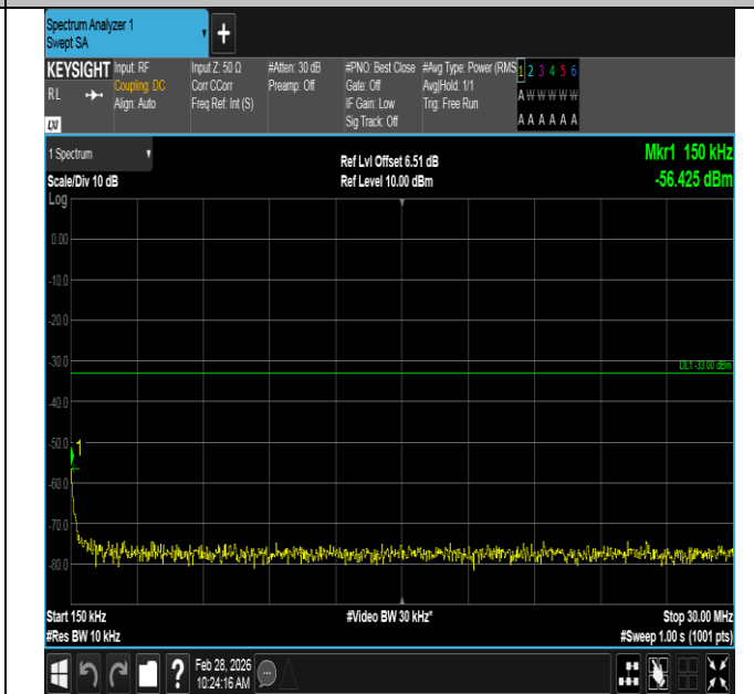
Band2-10MHz-QPSK-18650-1RB#0-0.15~30-PASS
