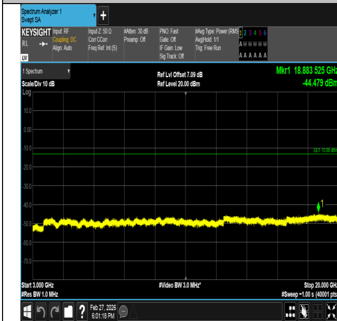
Band2-5MHz-QPSK-19175-25RB#0-3000~20000-PASS
