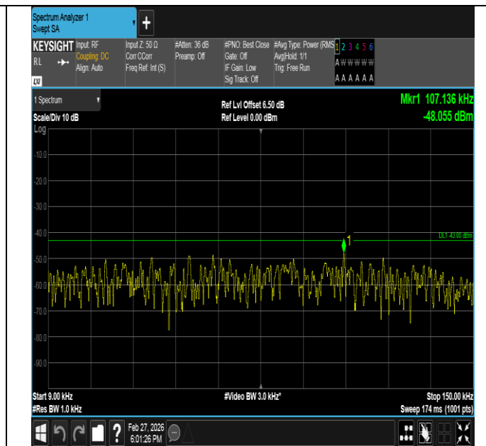
Band2-5MHz-16QAM-19175-25RB#0-0.009~0.15-PASS
