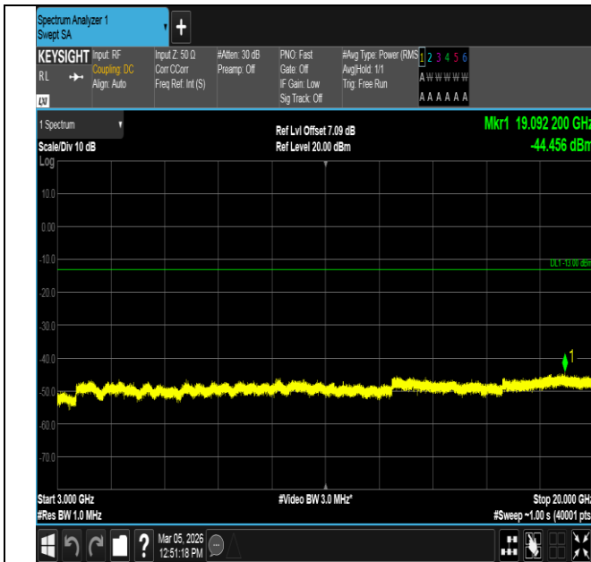
Band2-10MHz-QPSK-18650-50RB#0-3000~20000-PASS
