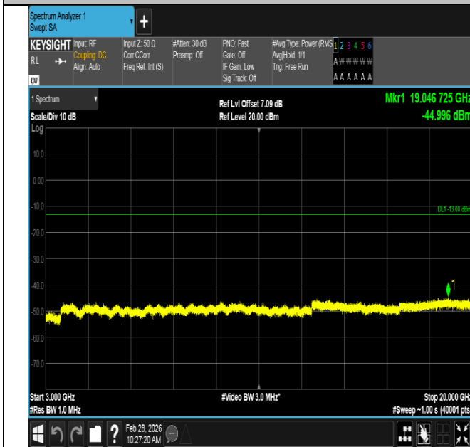
Band2-10MHz-16QAM-18650-1RB#49-3000~20000-PASS
