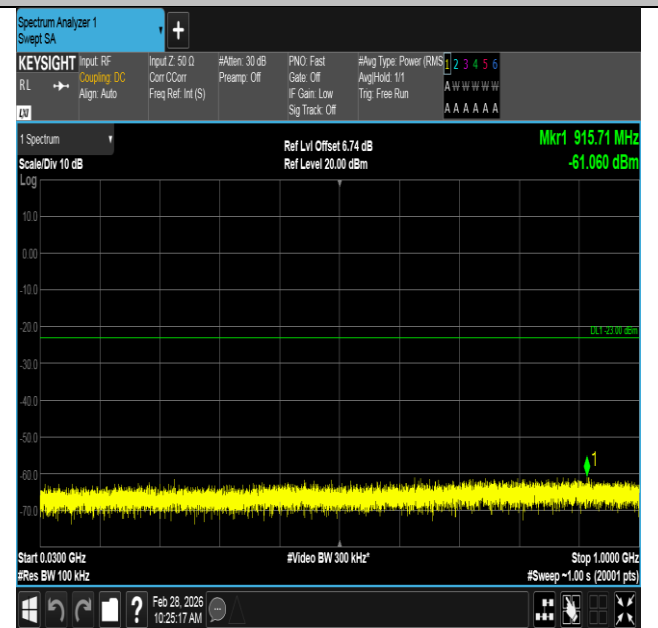
Band2-10MHz-16QAM-18650-1RB#0-30~1000-PASS
