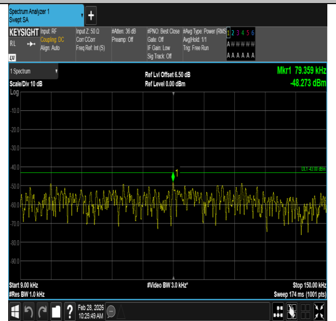
Band2-10MHz-QPSK-18650-1RB#49-0.009~0.15-PASS
