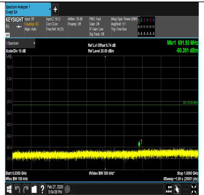
Band2-5MHz-QPSK-18900-1RB#24-30~1000-PASS
