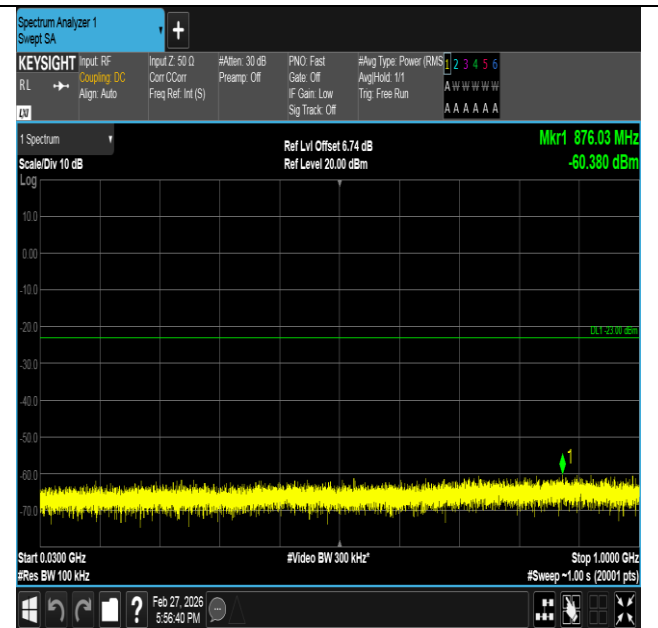
Band2-5MHz-16QAM-18900-25RB#0-30~1000-PASS
