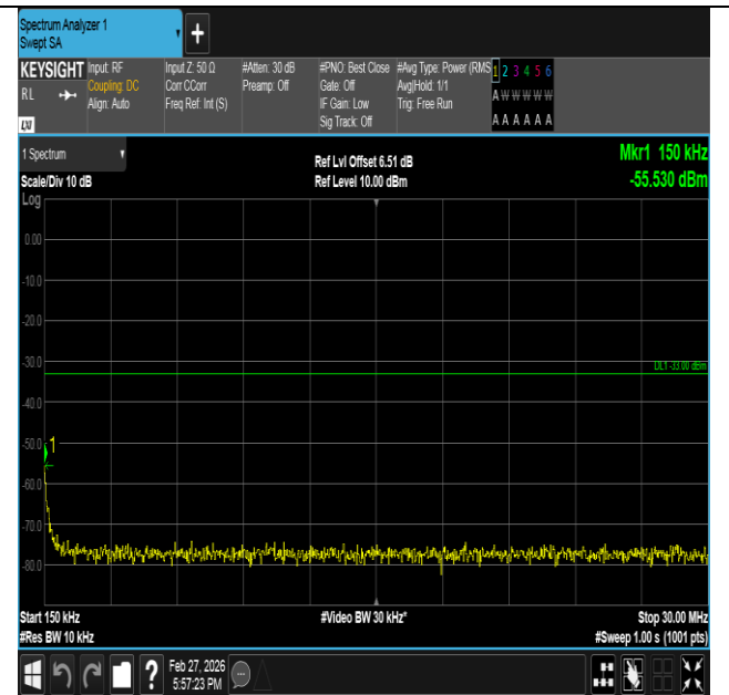
Band2-5MHz-QPSK-19175-1RB#0-0.15~30-PASS
