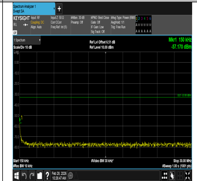
Band2-10MHz-16QAM-18650-1RB#49-0.15~30-PASS
