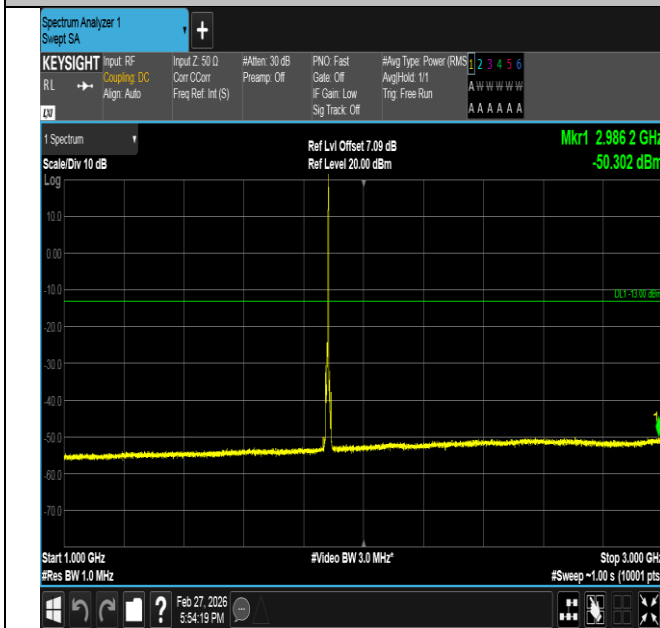
Band2-5MHz-QPSK-18900-1RB#24-1000~3000-PASS
