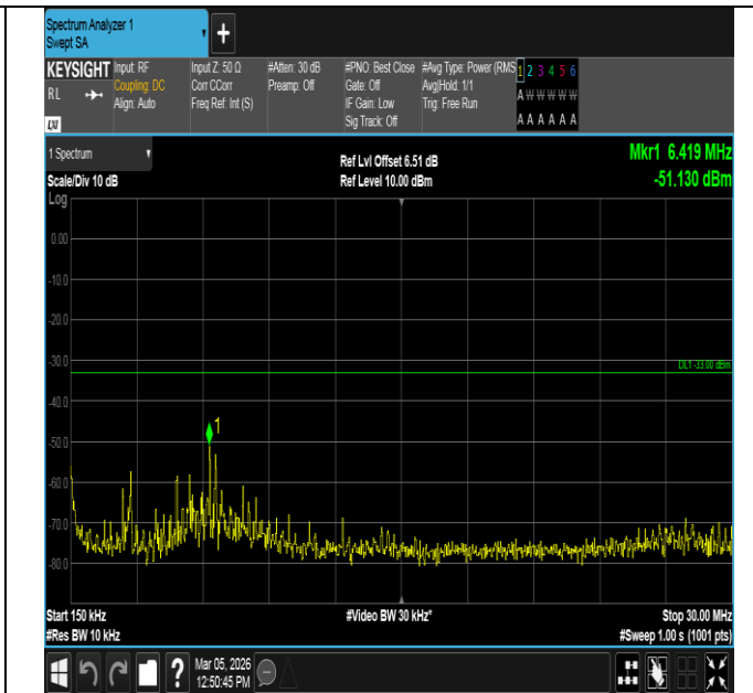
Band2-10MHz-QPSK-18650-50RB#0-0.15~30-PASS
