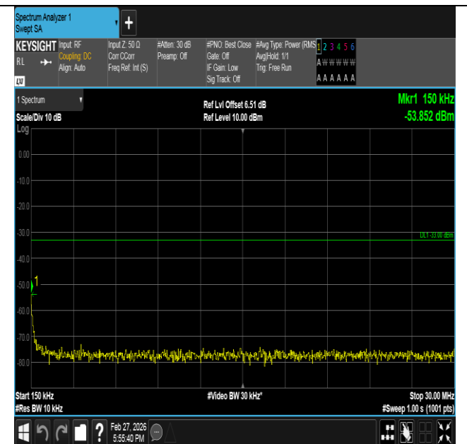
Band2-5MHz-QPSK-18900-25RB#0-0.15~30-PASS
