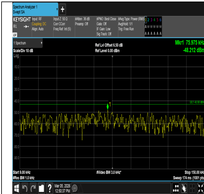
Band2-10MHz-QPSK-18650-50RB#0-0.009~0.15-PASS
