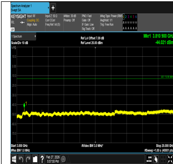
Band2-5MHz-QPSK-19175-1RB#0-3000~20000-PASS
