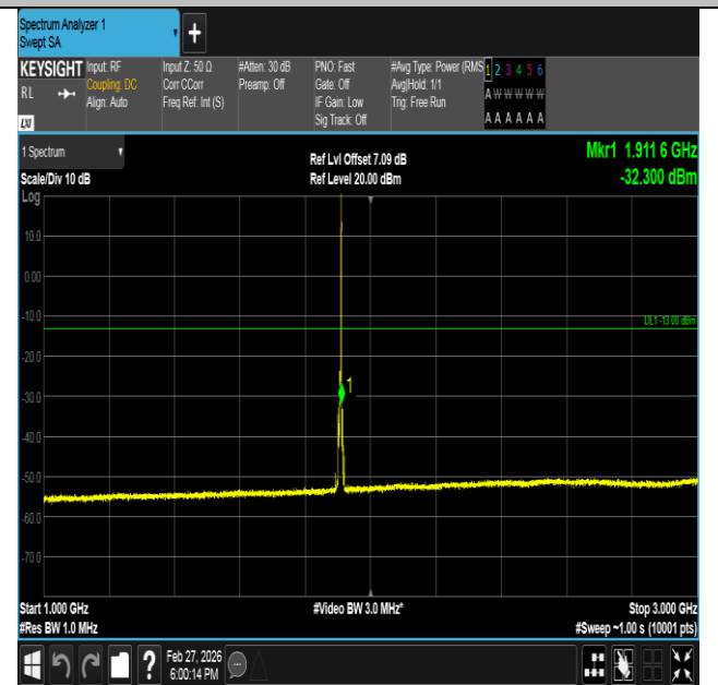
Band2-5MHz-16QAM-19175-1RB#24-1000~3000-PASS
