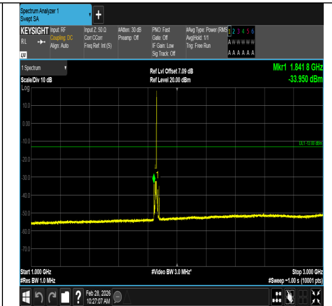
Band2-10MHz-16QAM-18650-1RB#49-1000~3000-PASS
