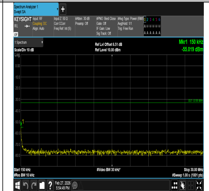
Band2-5MHz-16QAM-18900-1RB#24-0.15~30-PASS
