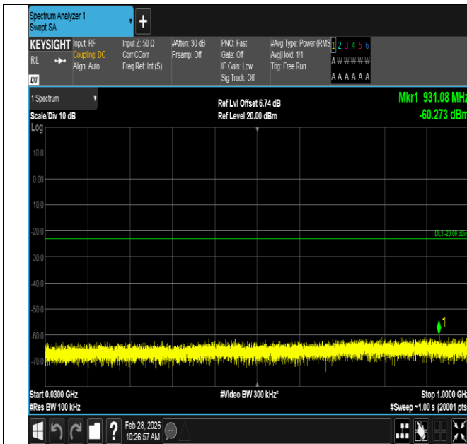
Band2-10MHz-16QAM-18650-1RB#49-30~1000-PASS
