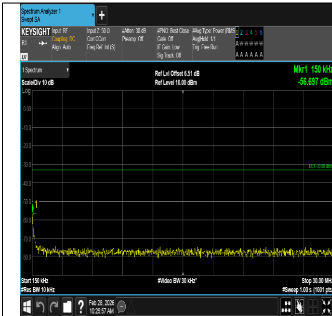
Band2-10MHz-QPSK-18650-1RB#49-0.15~30-PASS
