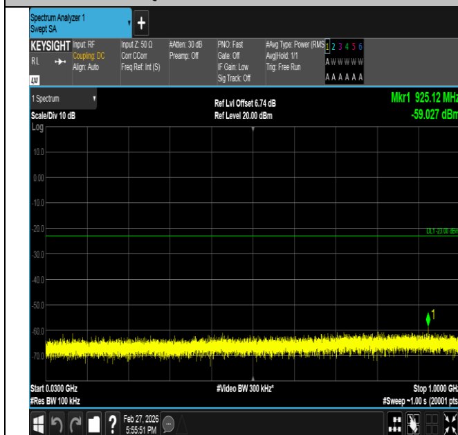
Band2-5MHz-QPSK-18900-25RB#0-30~1000-PASS
