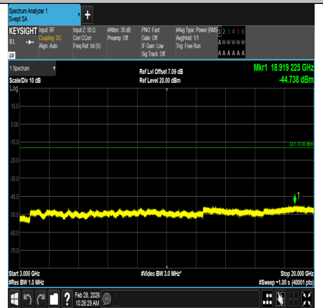
Band2-10MHz-QPSK-18650-1RB#49-3000~20000-PASS
