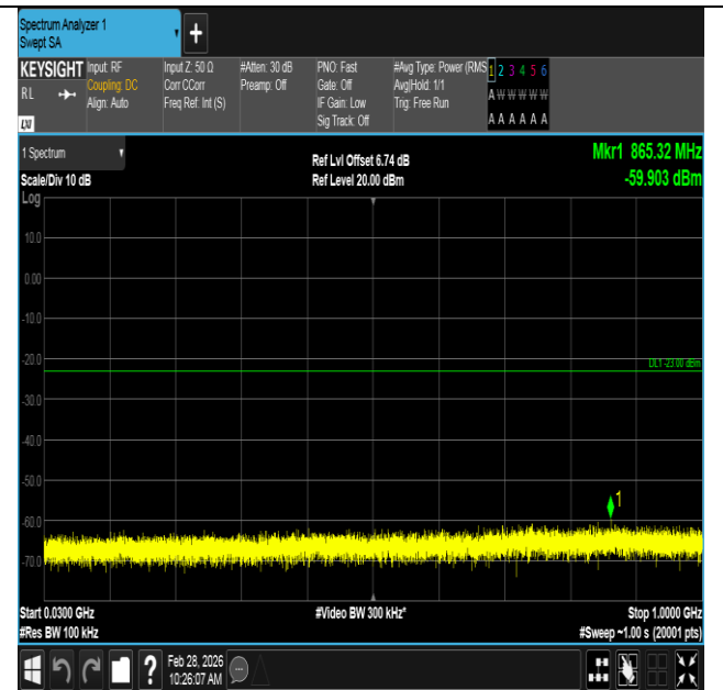
Band2-10MHz-QPSK-18650-1RB#49-30~1000-PASS
