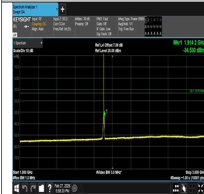
Band2-5MHz-16QAM-19175-1RB#0-1000~3000-PASS
