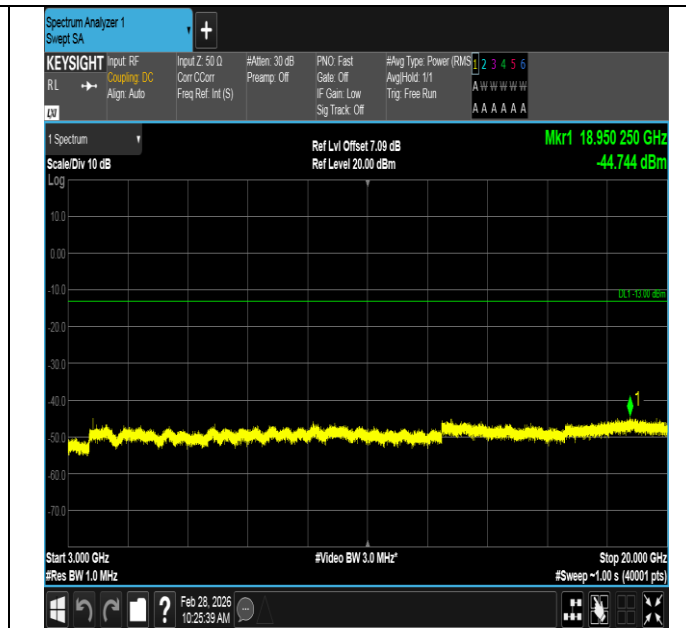
Band2-10MHz-16QAM-18650-1RB#0-3000~20000-PASS
