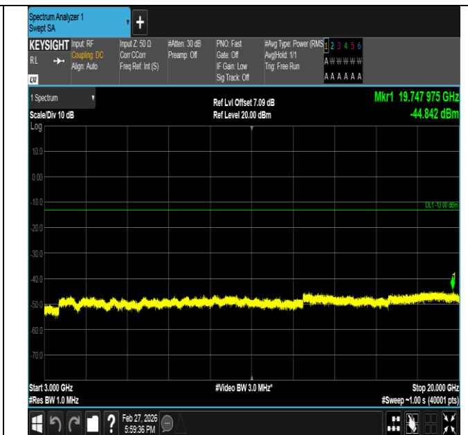
Band2-5MHz-QPSK-19175-1RB#24-3000~20000-PASS
