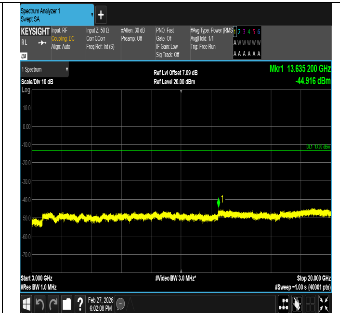
Band2-5MHz-16QAM-19175-25RB#0-3000~20000-PASS
