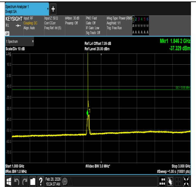
Band2-10MHz-QPSK-18650-1RB#0-1000~3000-PASS
