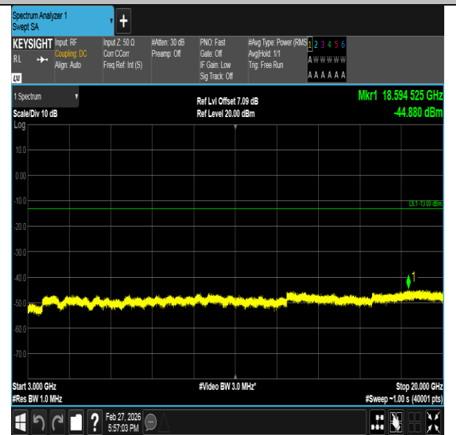
Band2-5MHz-16QAM-18900-25RB#0-3000~20000-PASS
