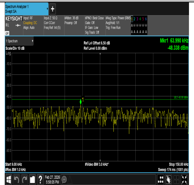
Band2-5MHz-16QAM-19175-1RB#0-0.009~0.15-PASS
