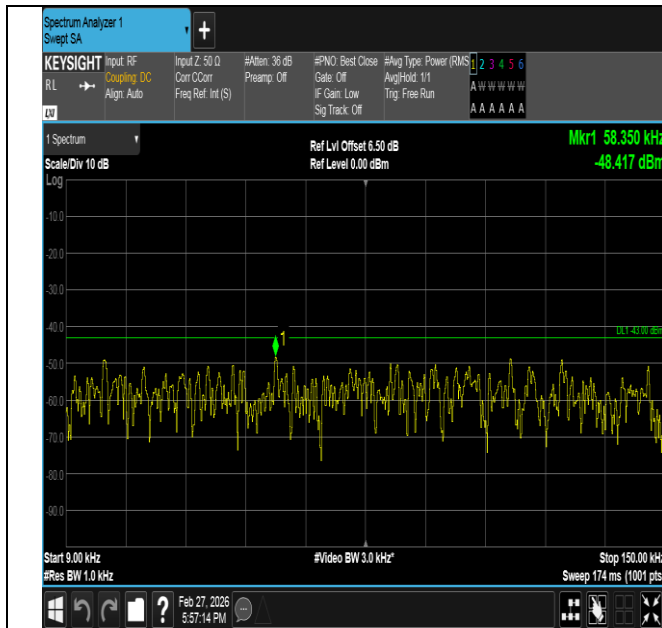
Band2-5MHz-QPSK-19175-1RB#0-0.009~0.15-PASS
