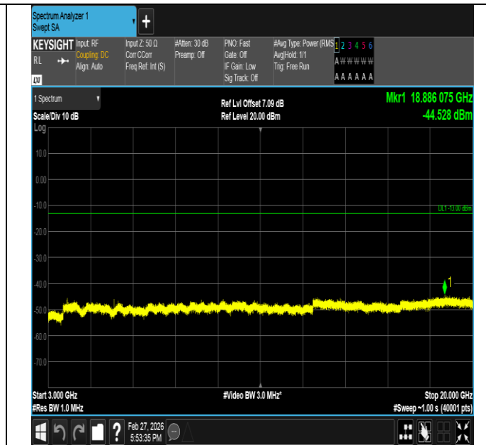
Band2-5MHz-16QAM-18900-1RB#0-3000~20000-PASS
