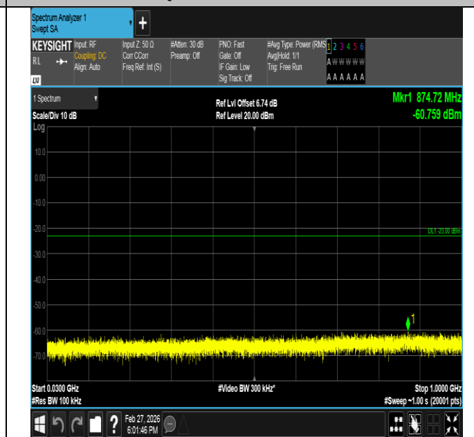
Band2-5MHz-16QAM-19175-25RB#0-30~1000-PASS
