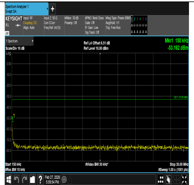
Band2-5MHz-16QAM-19175-1RB#24-0.15~30-PASS
