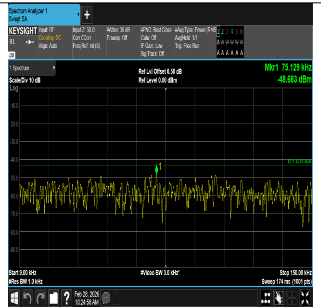
Band2-10MHz-16QAM-18650-1RB#0-0.009~0.15-PASS
