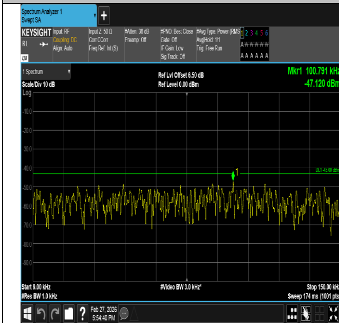
Band2-5MHz-16QAM-18900-1RB#24-0.009~0.15-PASS
