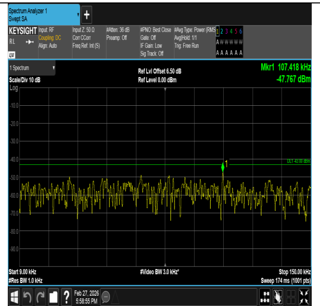
Band2-5MHz-QPSK-19175-1RB#24-0.009~0.15-PASS
