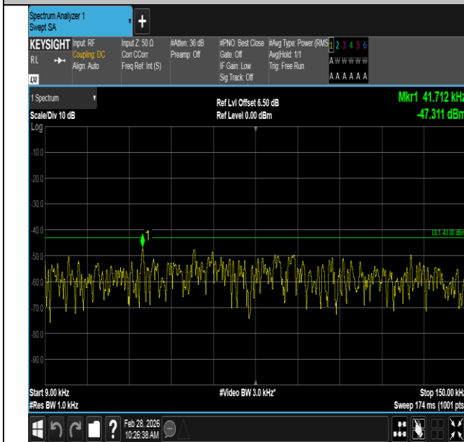
Band2-10MHz-16QAM-18650-1RB#49-0.009~0.15-PASS
