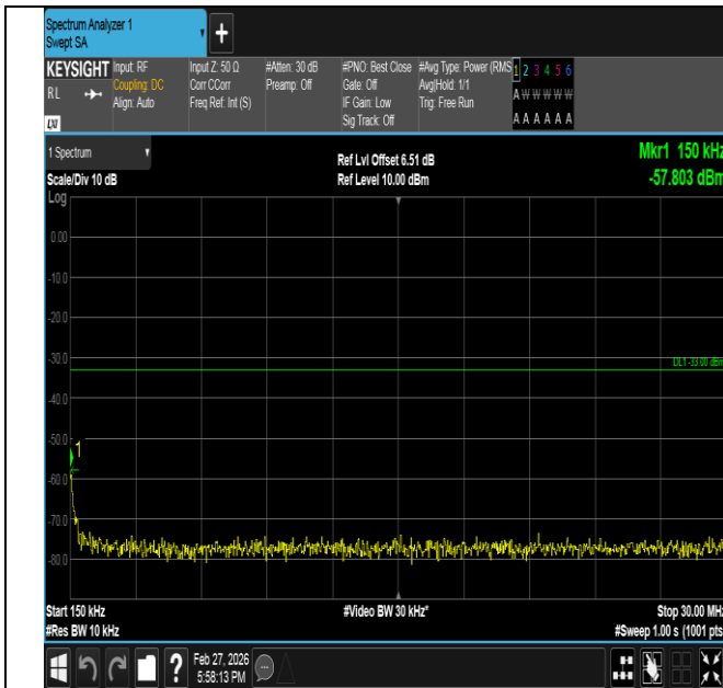
Band2-5MHz-16QAM-19175-1RB#0-0.15~30-PASS
