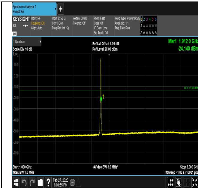
Band2-5MHz-16QAM-19175-25RB#0-1000~3000-PASS
