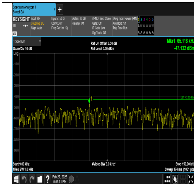
Band2-5MHz-QPSK-18900-25RB#0-0.009~0.15-PASS
