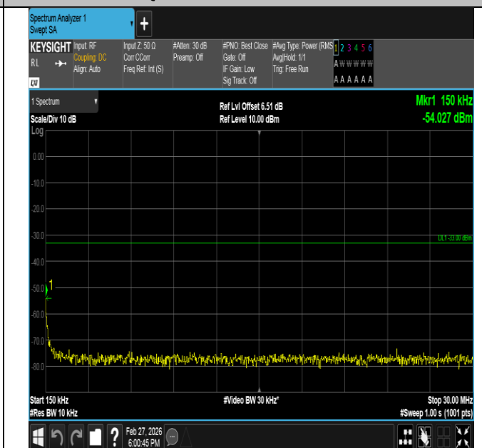
Band2-5MHz-QPSK-19175-25RB#0-0.15~30-PASS
