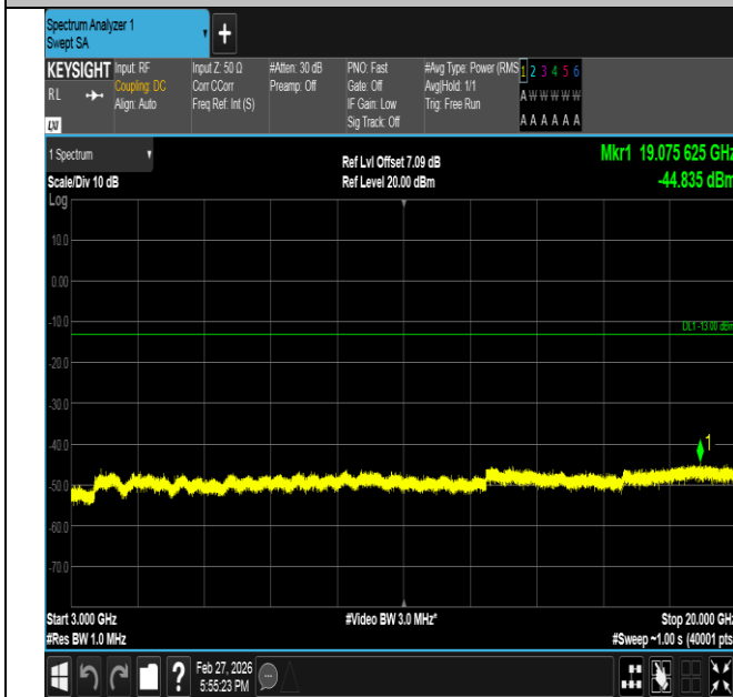
Band2-5MHz-16QAM-18900-1RB#24-3000~20000-PASS
