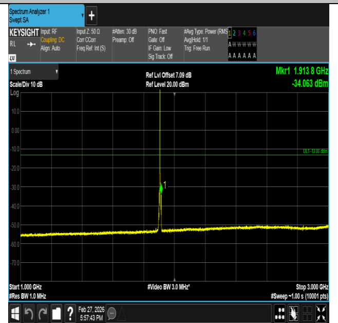
Band2-5MHz-QPSK-19175-1RB#0-1000~3000-PASS
