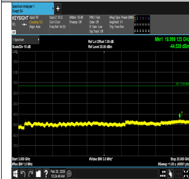
Band2-10MHz-QPSK-18650-1RB#0-3000~20000-PASS
