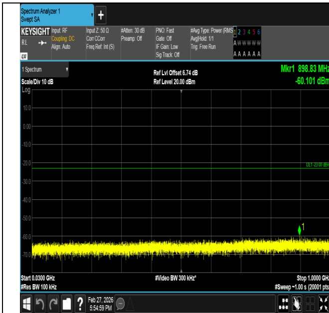
Band2-5MHz-16QAM-18900-1RB#24-30~1000-PASS
