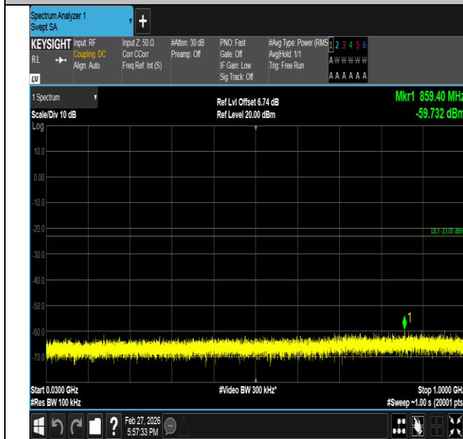
Band2-5MHz-QPSK-19175-1RB#0-30~1000-PASS
