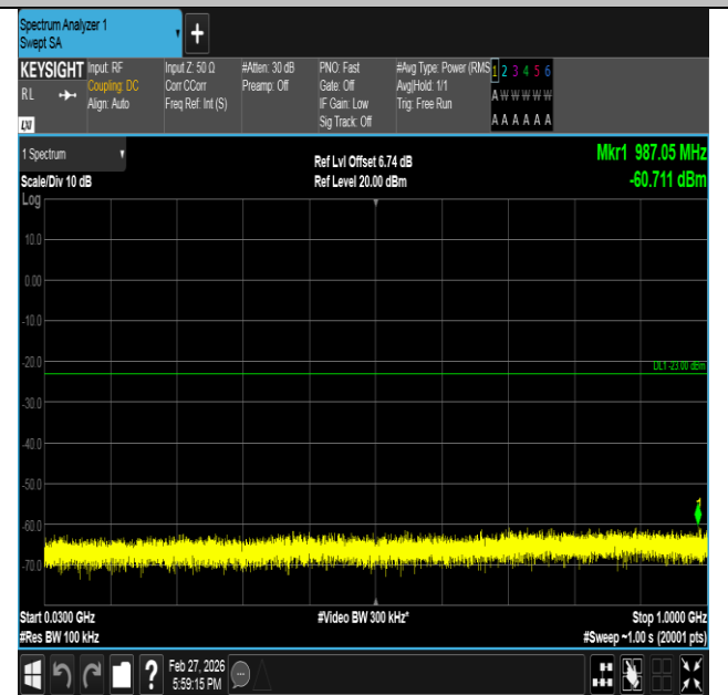
Band2-5MHz-QPSK-19175-1RB#24-30~1000-PASS
