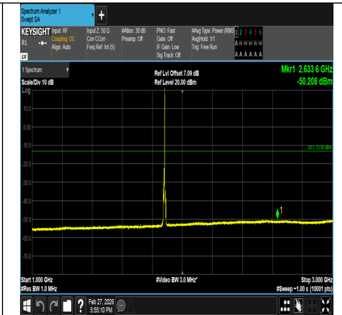
Band2-5MHz-16QAM-18900-1RB#24-1000~3000-PASS
