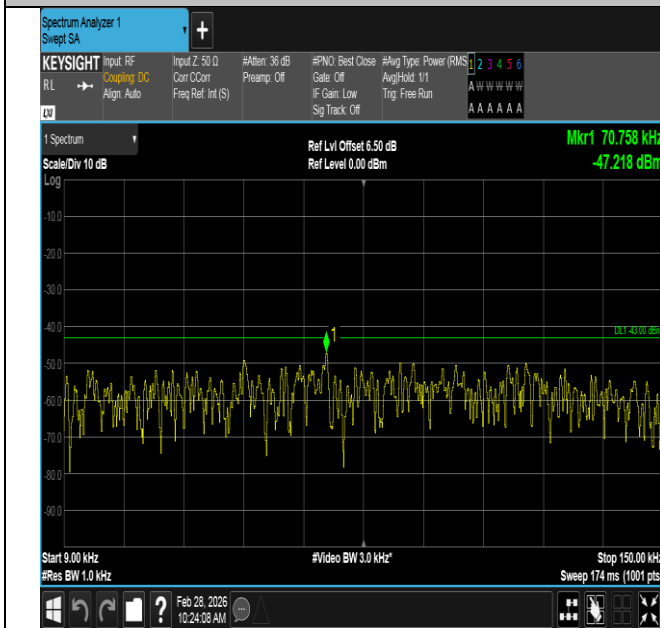
Band2-10MHz-QPSK-18650-1RB#0-0.009~0.15-PASS
