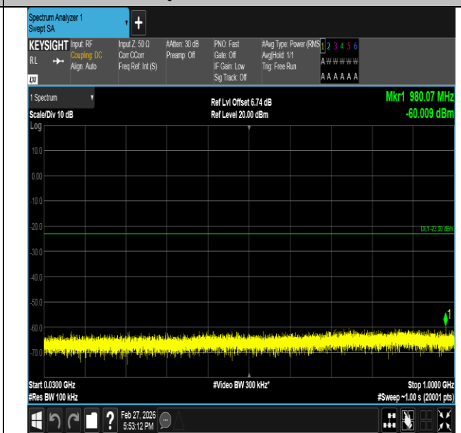
Band2-5MHz-16QAM-18900-1RB#0-30~1000-PASS
