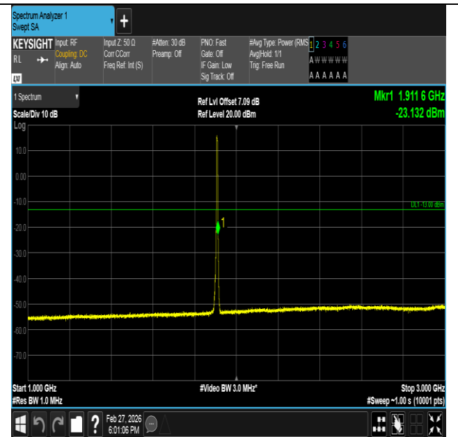
Band2-5MHz-QPSK-19175-25RB#0-1000~3000-PASS
