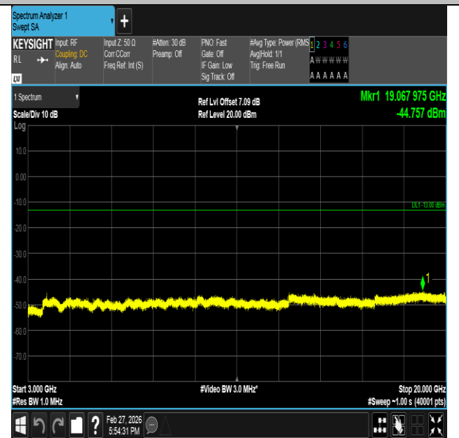
Band2-5MHz-QPSK-18900-1RB#24-3000~20000-PASS
