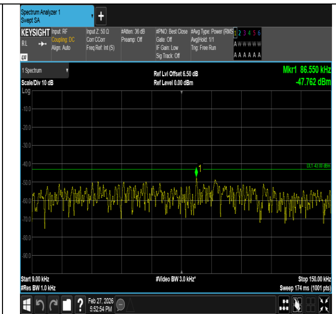
Band2-5MHz-16QAM-18900-1RB#0-0.009~0.15-PASS
