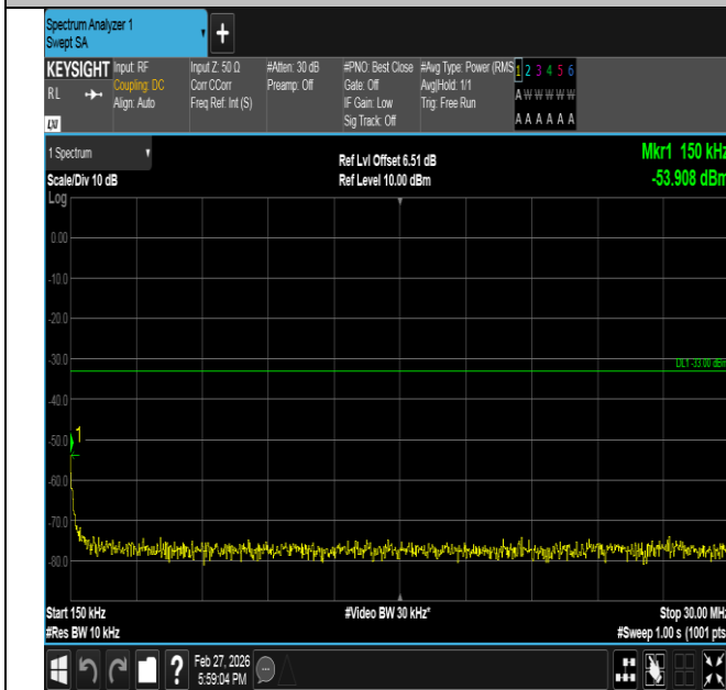
Band2-5MHz-QPSK-19175-1RB#24-0.15~30-PASS
