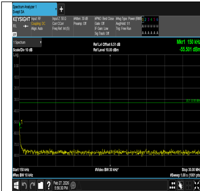
Band2-5MHz-16QAM-18900-25RB#0-0.15~30-PASS
