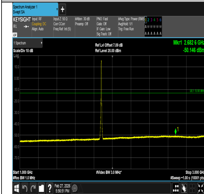
Band2-5MHz-16QAM-18900-25RB#0-1000~3000-PASS
