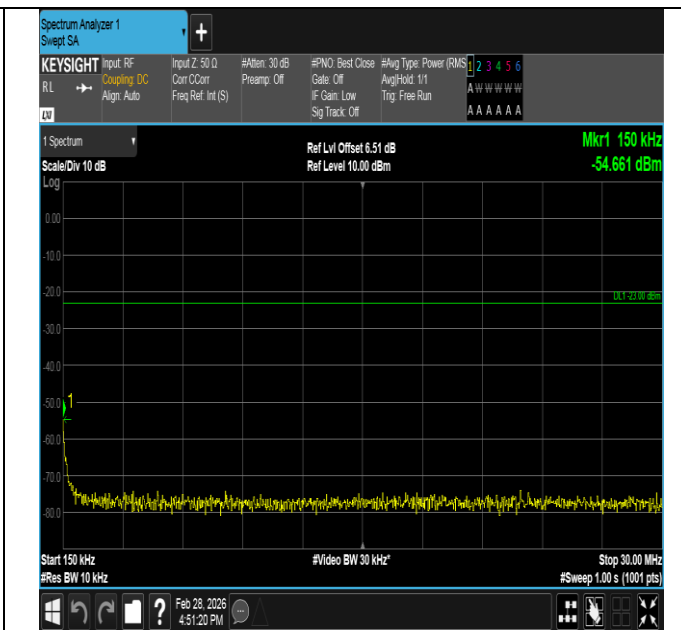
Band5-1.4MHz-QPSK-20407-6RB#0-0.15~30-PASS
