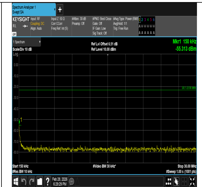
Band5-10MHz-QPSK-20600-1RB#0-0.15~30-PASS
