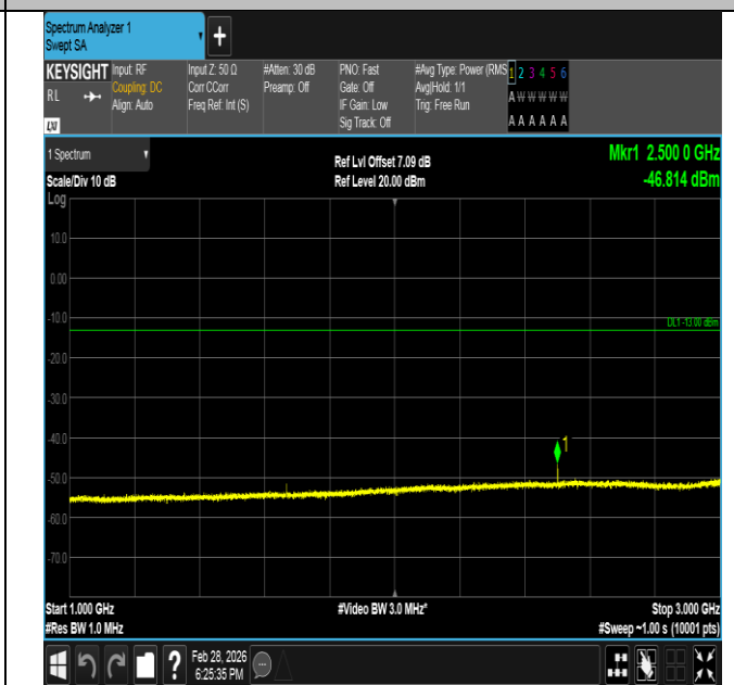
Band5-10MHz-16QAM-20450-1RB#49-1000~3000-PASS
