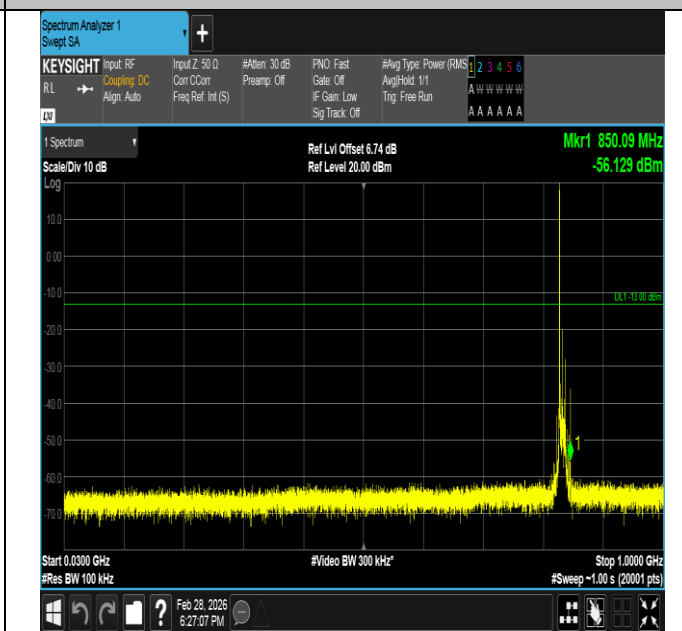
Band5-10MHz-16QAM-20525-1RB#0-30~1000-PASS
