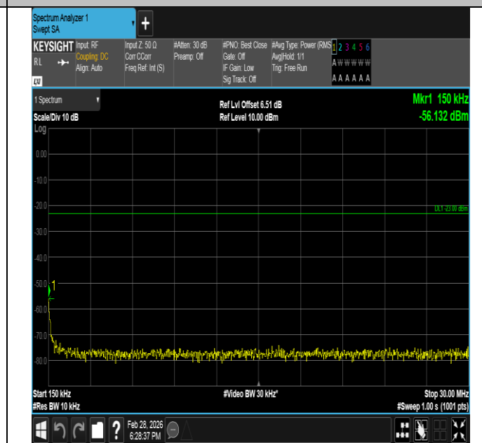
Band5-10MHz-16QAM-20525-1RB#49-0.15~30-PASS
