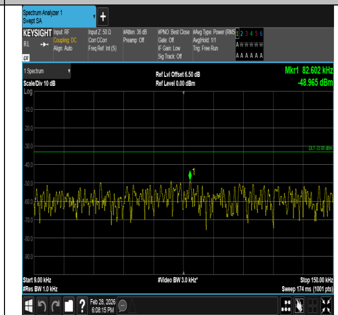
Band5-5MHz-16QAM-20625-25RB#0-0.009~0.15-PASS
