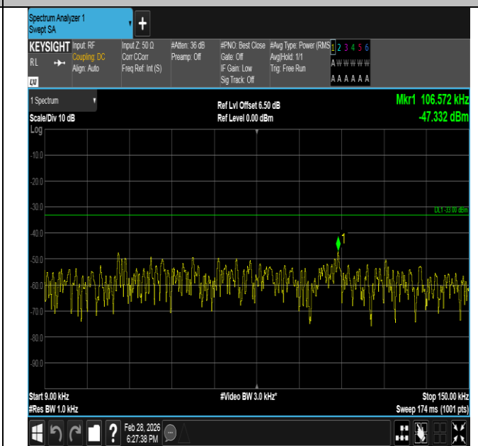
Band5-10MHz-QPSK-20525-1RB#49-0.009~0.15-PASS
