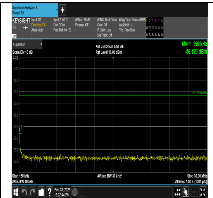
Band5-10MHz-QPSK-20450-1RB#0-0.15~30-PASS
