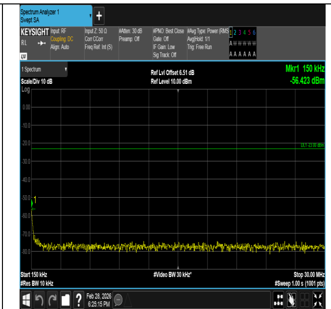
Band5-10MHz-16QAM-20450-1RB#49-0.15~30-PASS
