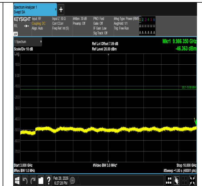
Band5-10MHz-16QAM-20525-1RB#0-3000~10000-PASS
