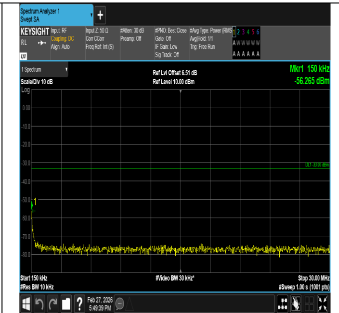
Band2-5MHz-16QAM-18625-1RB#24-0.15~30-PASS
