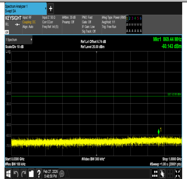
Band2-5MHz-QPSK-18625-1RB#24-30~1000-PASS
