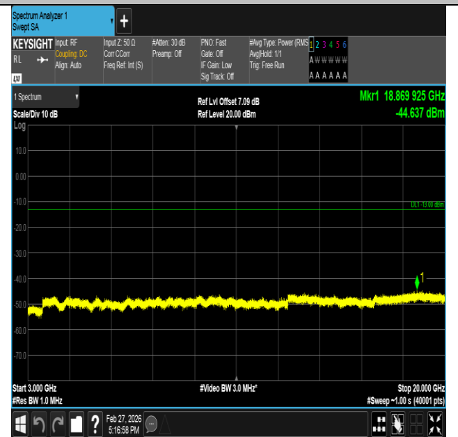
Band2-3MHz-16QAM-19185-15RB#0-3000~20000-PASS
