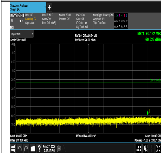
Band2-5MHz-QPSK-18625-1RB#0-30~1000-PASS
