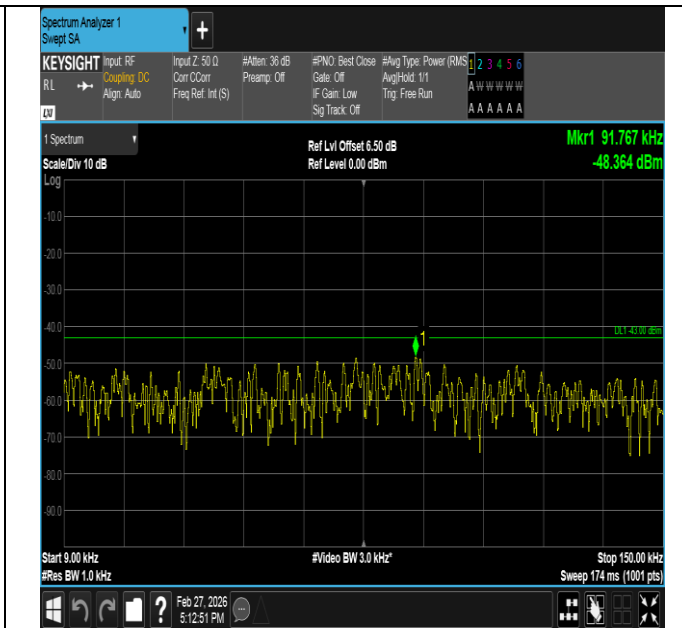
Band2-3MHz-16QAM-19185-1RB#0-0.009~0.15-PASS
