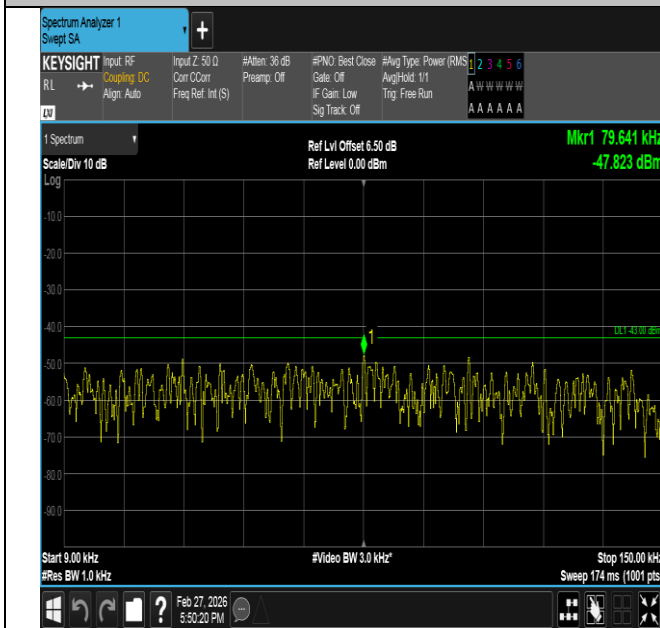
Band2-5MHz-QPSK-18625-25RB#0-0.009~0.15-PASS
