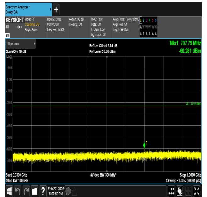
Band2-3MHz-16QAM-18900-1RB#0-30~1000-PASS
