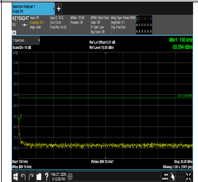
Band2-3MHz-QPSK-19185-1RB#0-0.15~30-PASS
