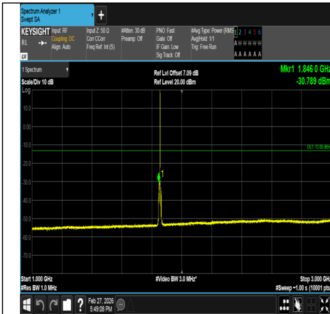
Band2-5MHz-QPSK-18625-1RB#24-1000~3000-PASS
