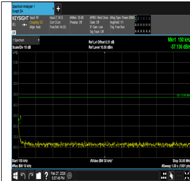
Band2-3MHz-16QAM-18900-1RB#0-0.15~30-PASS
