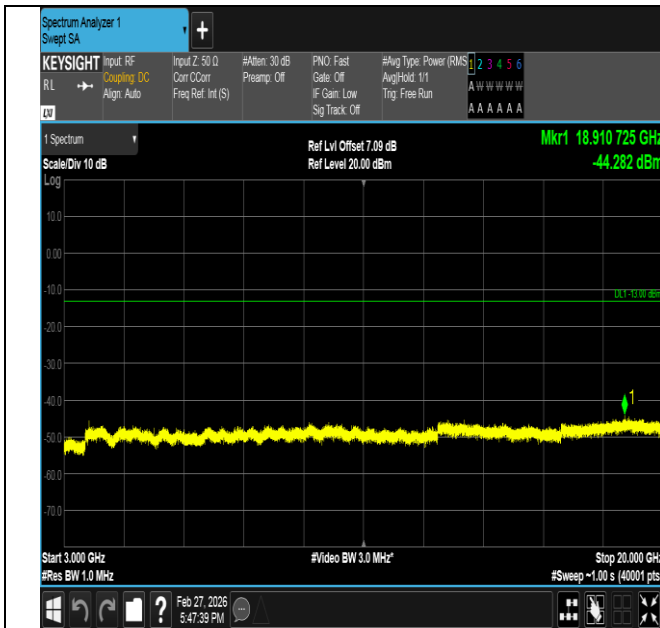
Band2-5MHz-QPSK-18625-1RB#0-3000~20000-PASS
