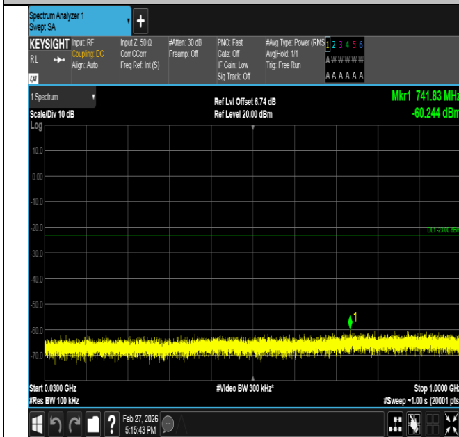
Band2-3MHz-QPSK-19185-15RB#0-30~1000-PASS
