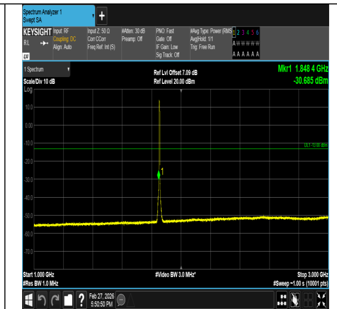
Band2-5MHz-QPSK-18625-25RB#0-1000~3000-PASS
