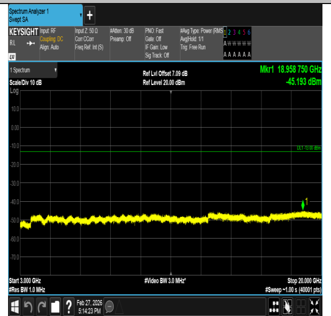
Band2-3MHz-QPSK-19185-1RB#14-3000~20000-PASS
