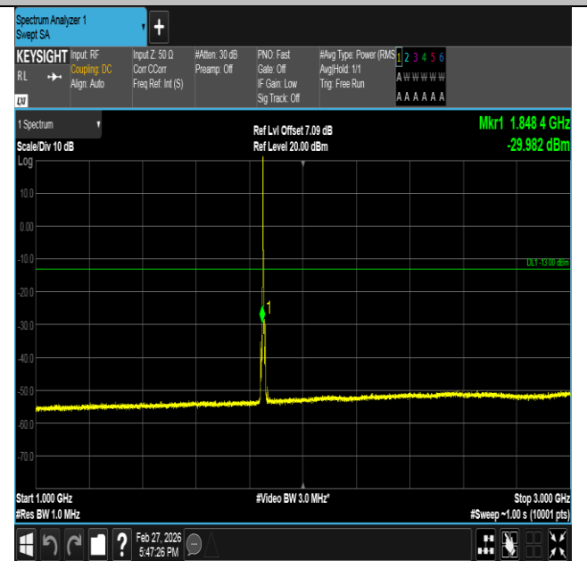
Band2-5MHz-QPSK-18625-1RB#0-1000~3000-PASS
