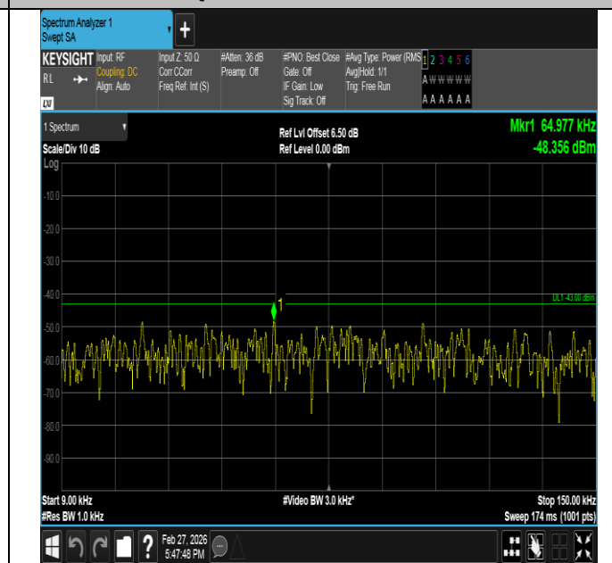
Band2-5MHz-16QAM-18625-1RB#0-0.009~0.15-PASS
