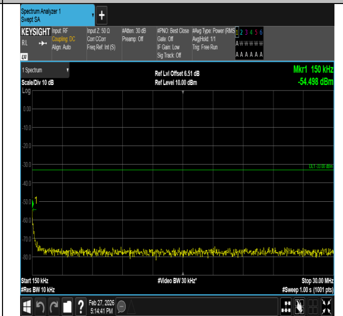
Band2-3MHz-16QAM-19185-1RB#14-0.15~30-PASS
