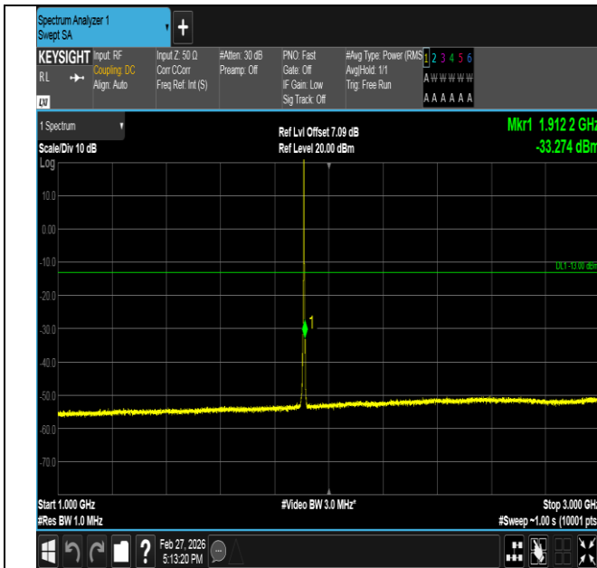
Band2-3MHz-16QAM-19185-1RB#0-1000~3000-PASS
