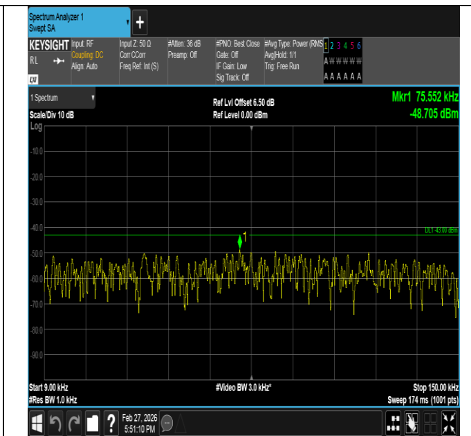
Band2-5MHz-16QAM-18625-25RB#0-0.009~0.15-PASS
