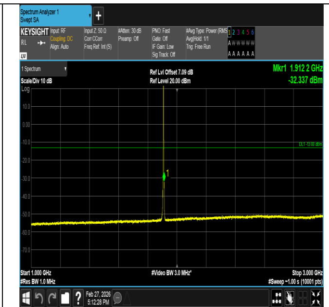
Band2-3MHz-QPSK-19185-1RB#0-1000~3000-PASS
