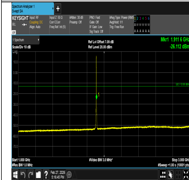
Band2-3MHz-16QAM-19185-15RB#0-1000~3000-PASS
