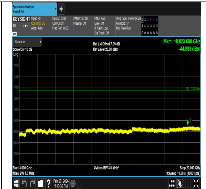
Band2-3MHz-16QAM-19185-1RB#0-3000~20000-PASS
