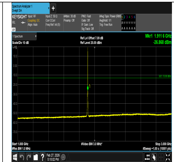
Band2-3MHz-16QAM-19185-1RB#14-1000~3000-PASS
