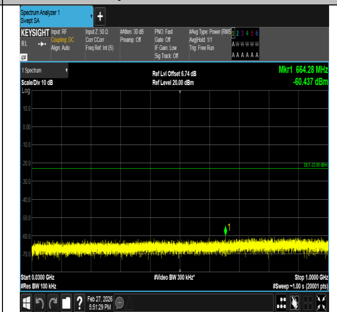
Band2-5MHz-16QAM-18625-25RB#0-30~1000-PASS
