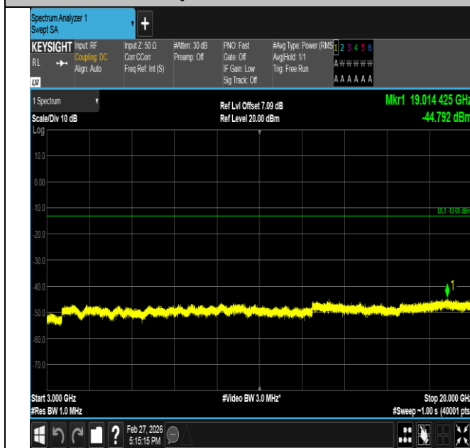
Band2-3MHz-16QAM-19185-1RB#14-3000~20000-PASS
