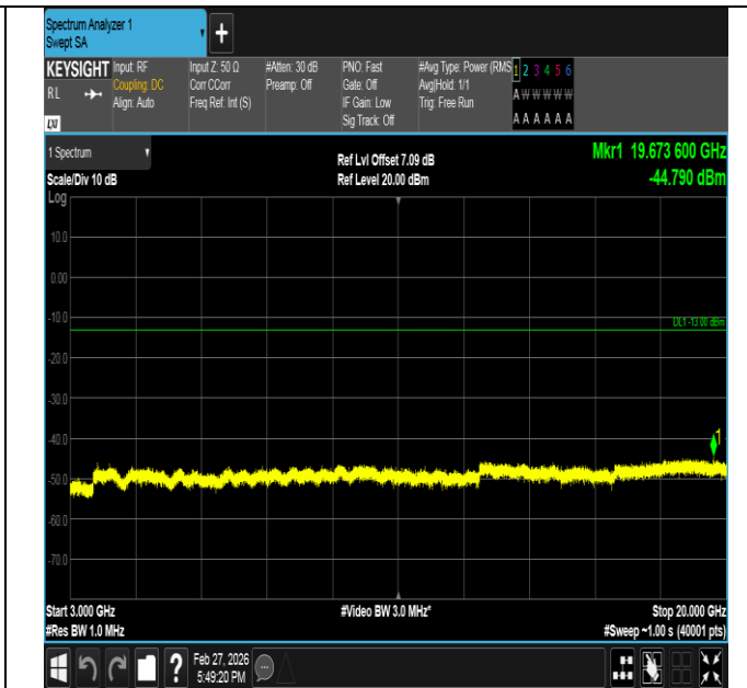
Band2-5MHz-QPSK-18625-1RB#24-3000~20000-PASS
