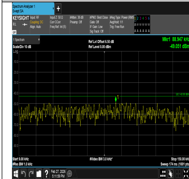
Band2-3MHz-QPSK-19185-1RB#0-0.009~0.15-PASS
