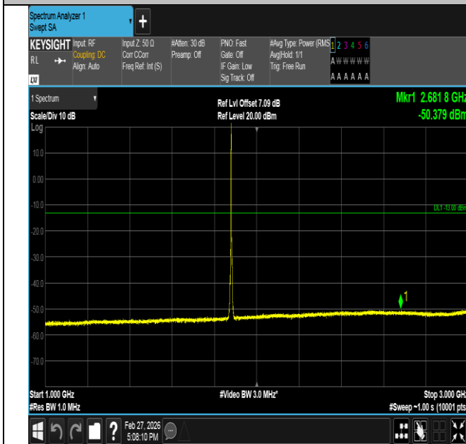
Band2-3MHz-16QAM-18900-1RB#0-1000~3000-PASS
