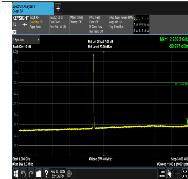
Band2-3MHz-16QAM-18900-15RB#0-1000~3000-PASS
