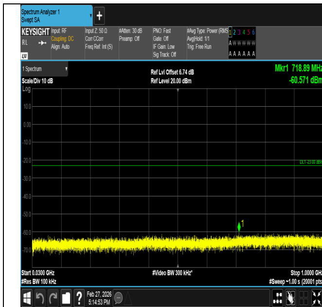
Band2-3MHz-16QAM-19185-1RB#14-30~1000-PASS
