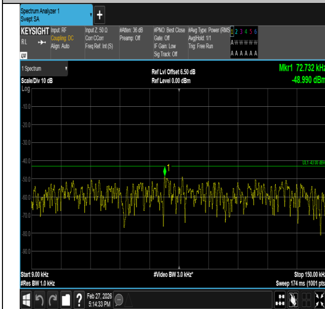
Band2-3MHz-16QAM-19185-1RB#14-0.009~0.15-PASS
