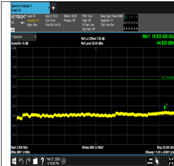
Band2-3MHz-QPSK-19185-15RB#0-3000~20000-PASS
