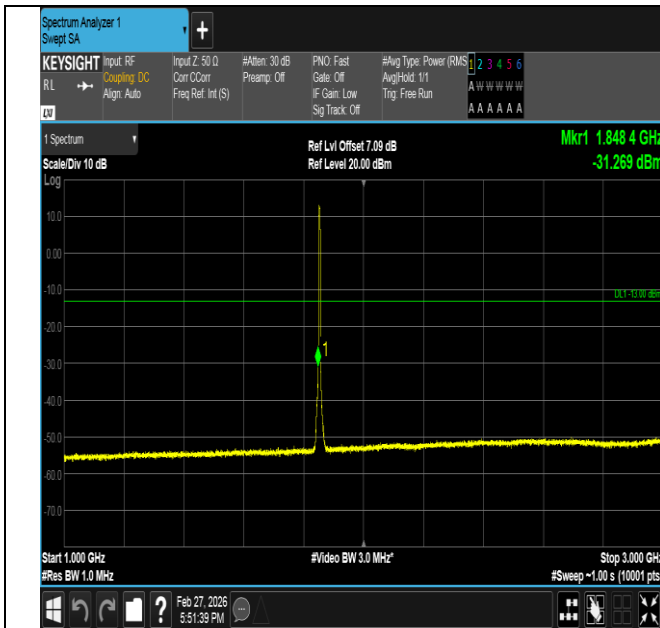
Band2-5MHz-16QAM-18625-25RB#0-1000~3000-PASS
