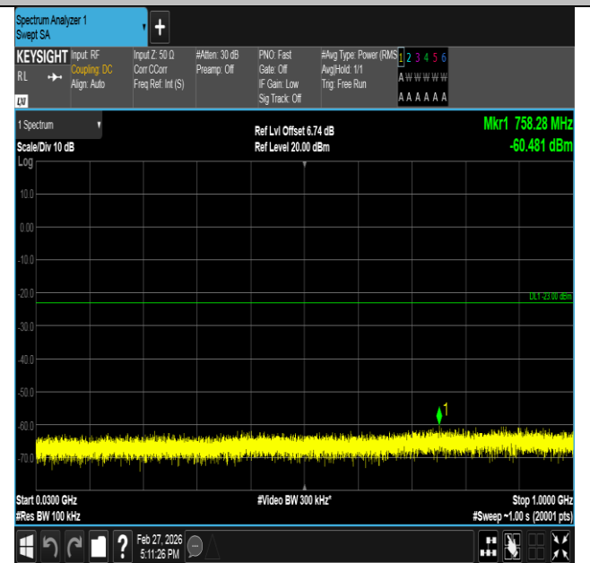
Band2-3MHz-16QAM-18900-15RB#0-30~1000-PASS
