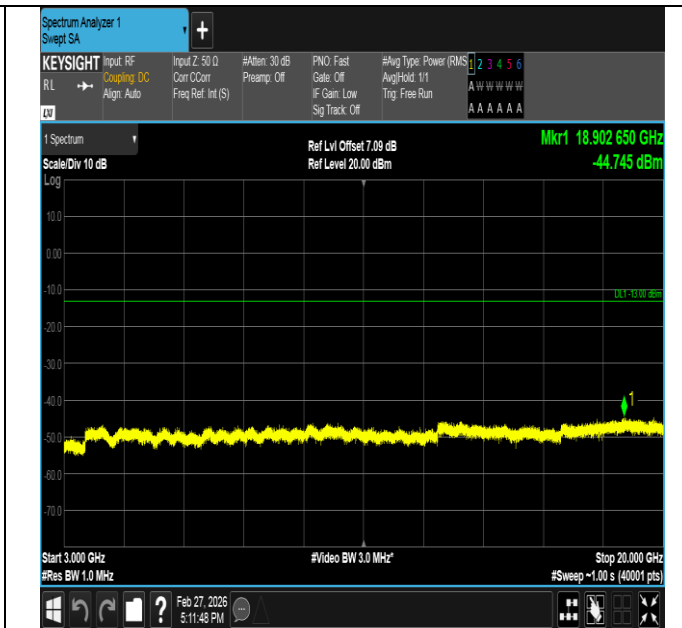
Band2-3MHz-16QAM-18900-15RB#0-3000~20000-PASS
