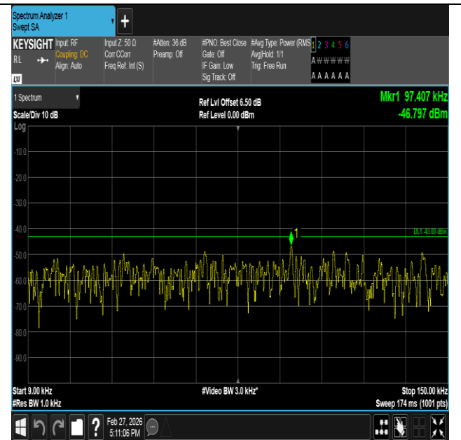
Band2-3MHz-16QAM-18900-15RB#0-0.009~0.15-PASS
