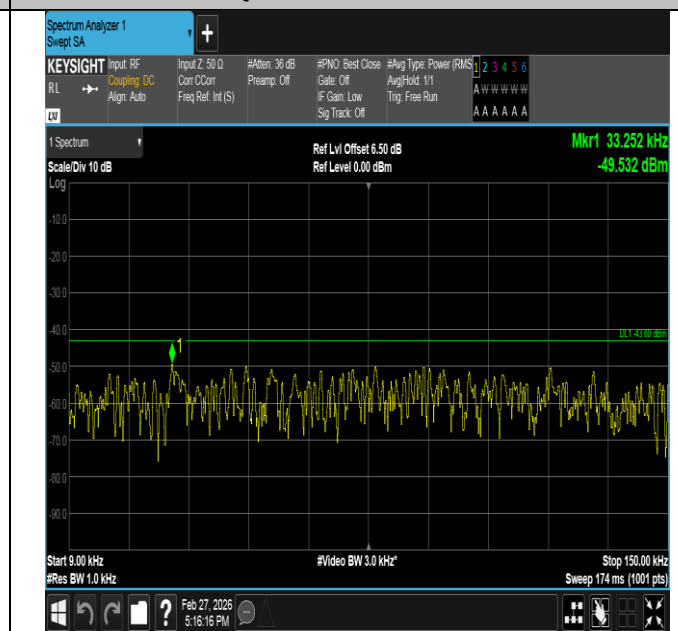
Band2-3MHz-16QAM-19185-15RB#0-0.009~0.15-PASS
