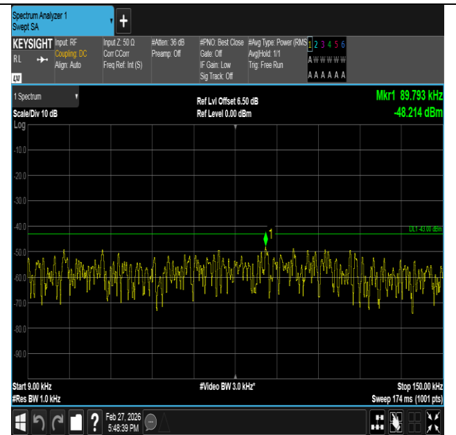
Band2-5MHz-QPSK-18625-1RB#24-0.009~0.15-PASS
