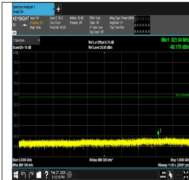
Band2-3MHz-QPSK-19185-1RB#0-30~1000-PASS
