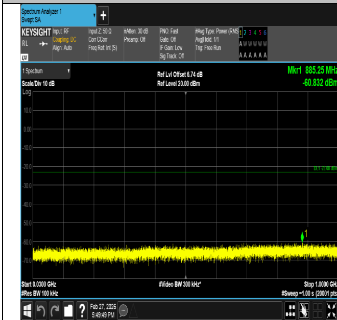
Band2-5MHz-16QAM-18625-1RB#24-30~1000-PASS
