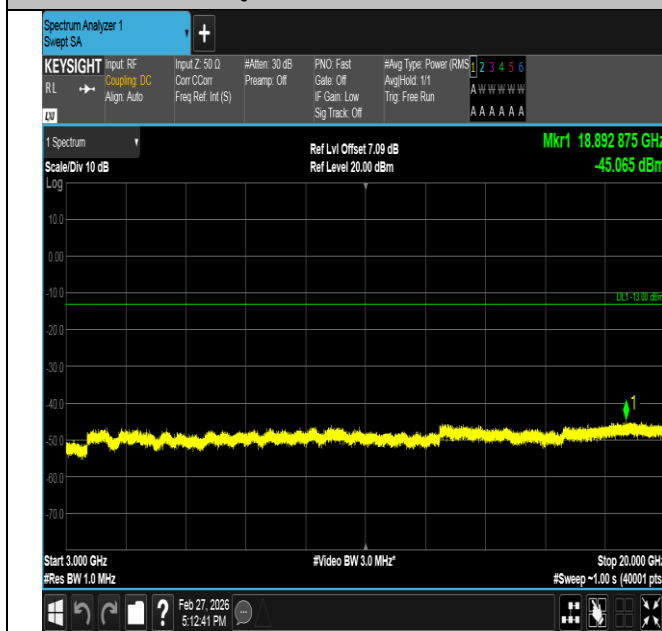
Band2-3MHz-QPSK-19185-1RB#0-3000~20000-PASS
