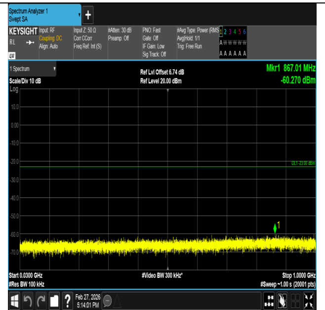
Band2-3MHz-QPSK-19185-1RB#14-30~1000-PASS
