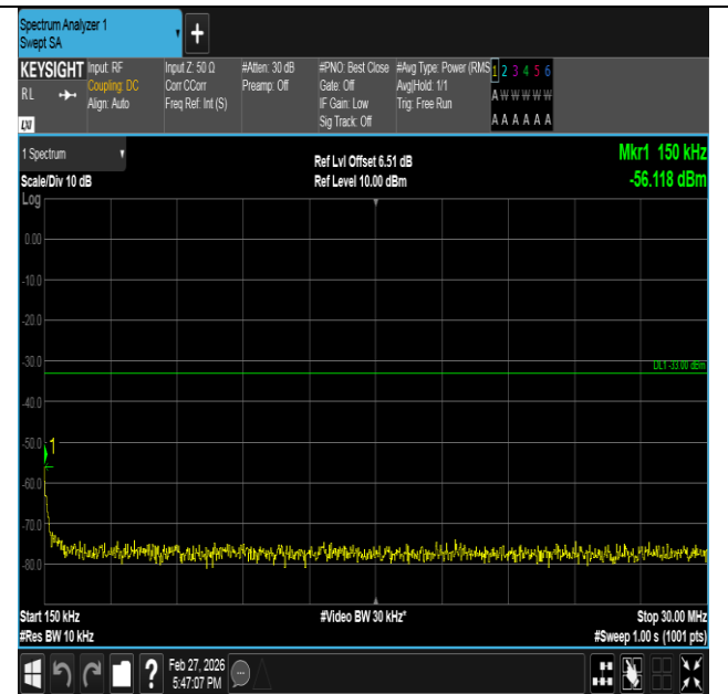
Band2-5MHz-QPSK-18625-1RB#0-0.15~30-PASS
