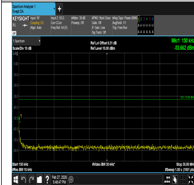
Band2-5MHz-QPSK-18625-1RB#24-0.15~30-PASS
