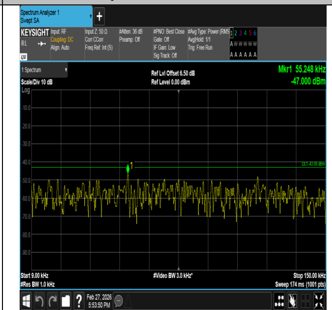
Band2-5MHz-QPSK-18900-1RB#24-0.009~0.15-PASS
