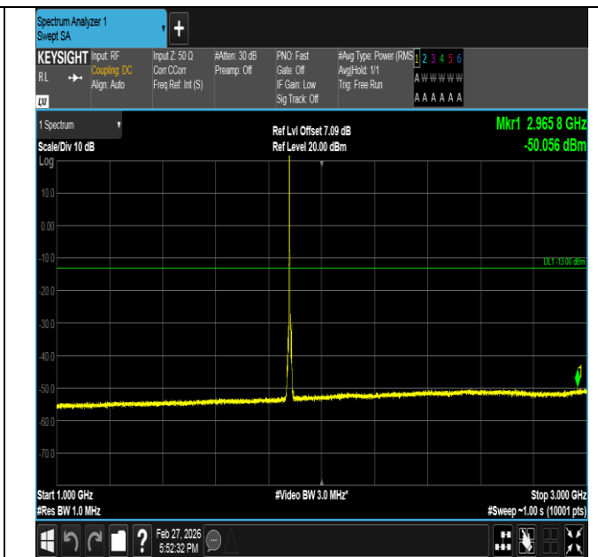
Band2-5MHz-QPSK-18900-1RB#0-1000~3000-PASS
