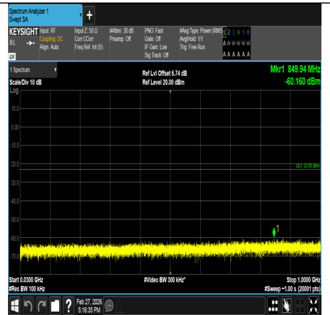
Band2-3MHz-16QAM-19185-15RB#0-30~1000-PASS
