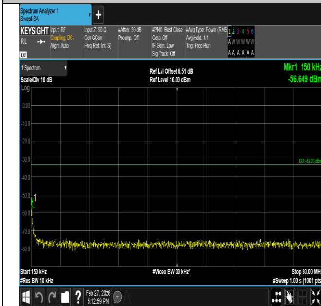
Band2-3MHz-16QAM-19185-1RB#0-0.15~30-PASS
