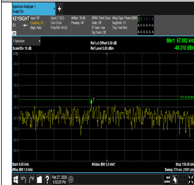
Band2-5MHz-QPSK-18900-1RB#0-0.009~0.15-PASS
