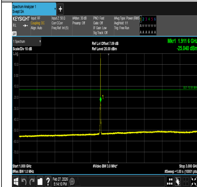
Band2-3MHz-QPSK-19185-1RB#14-1000~3000-PASS
