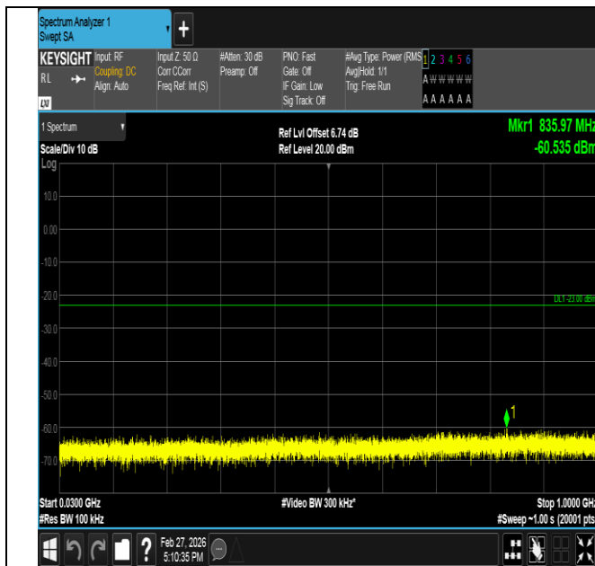
Band2-3MHz-QPSK-18900-15RB#0-30~1000-PASS
