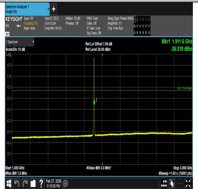
Band2-3MHz-QPSK-19185-15RB#0-1000~3000-PASS
