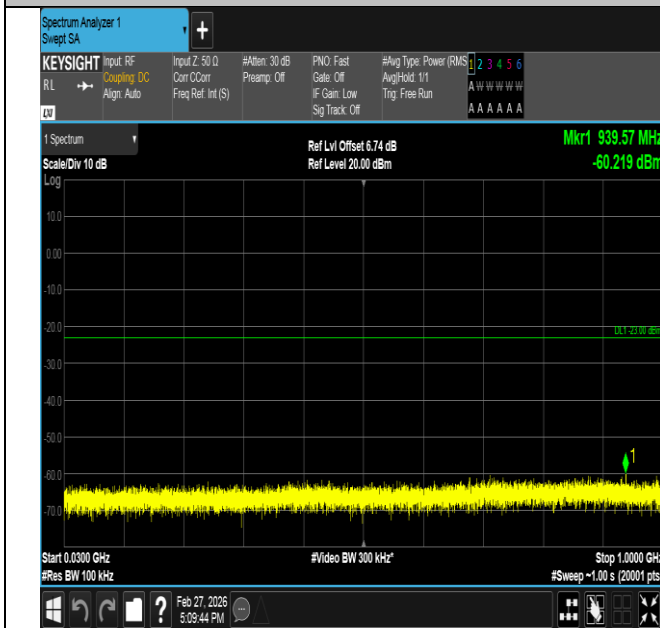
Band2-3MHz-16QAM-18900-1RB#14-30~1000-PASS
