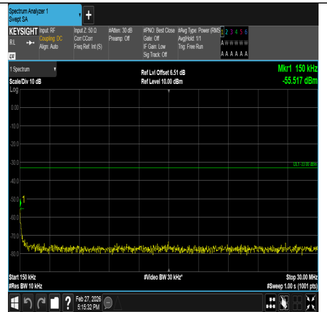
Band2-3MHz-QPSK-19185-15RB#0-0.15~30-PASS
