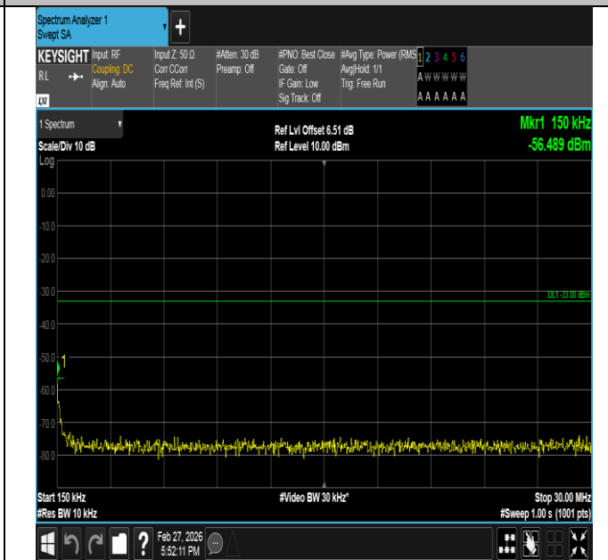
Band2-5MHz-QPSK-18900-1RB#0-0.15~30-PASS
