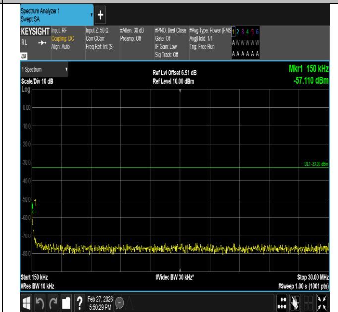
Band2-5MHz-QPSK-18625-25RB#0-0.15~30-PASS
