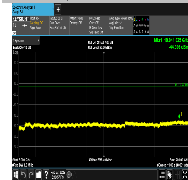
Band2-3MHz-QPSK-18900-15RB#0-3000~20000-PASS
