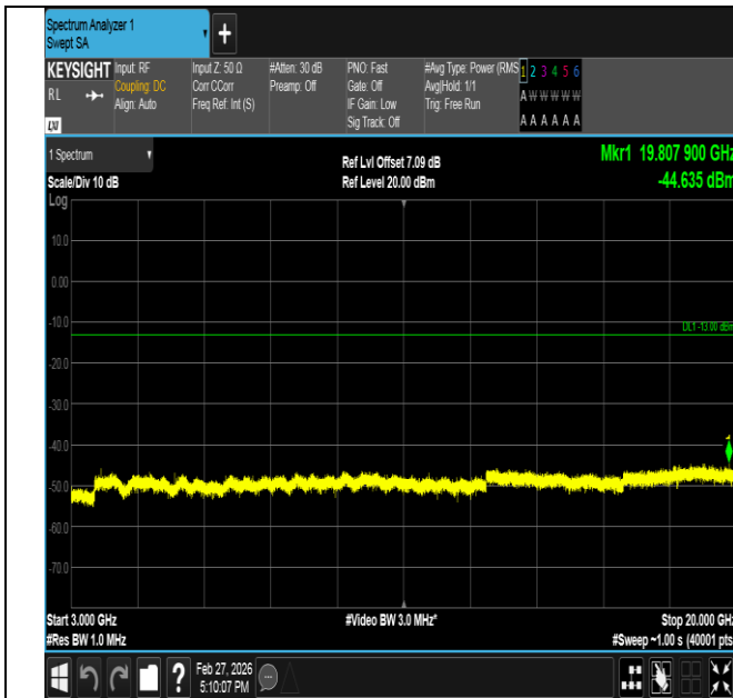
Band2-3MHz-16QAM-18900-1RB#14-3000~20000-PASS
