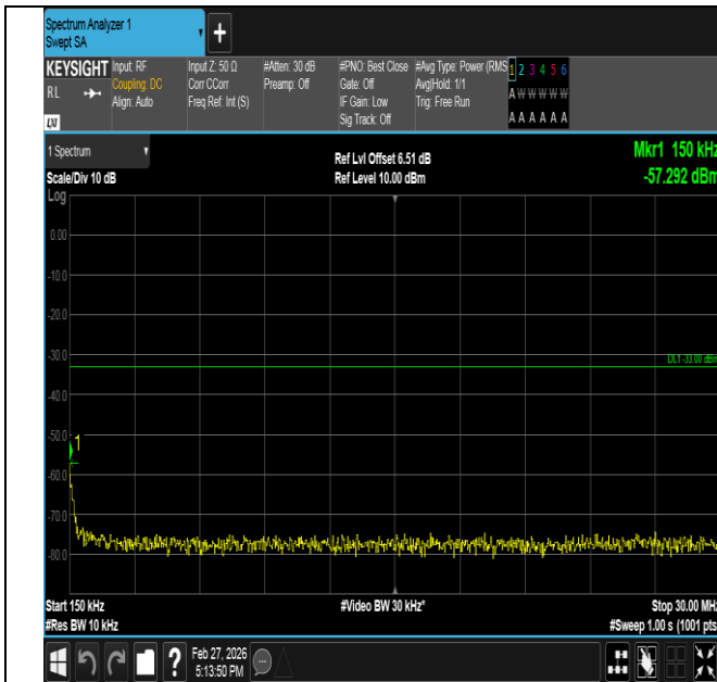
Band2-3MHz-QPSK-19185-1RB#14-0.15~30-PASS
