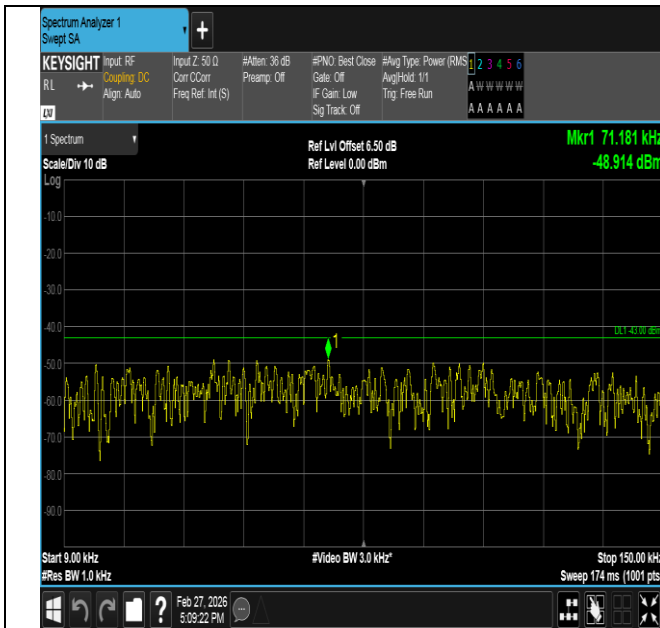
Band2-3MHz-16QAM-18900-1RB#14-0.009~0.15-PASS
