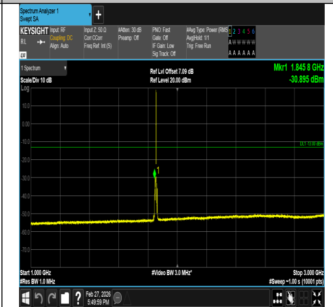
Band2-5MHz-16QAM-18625-1RB#24-1000~3000-PASS
