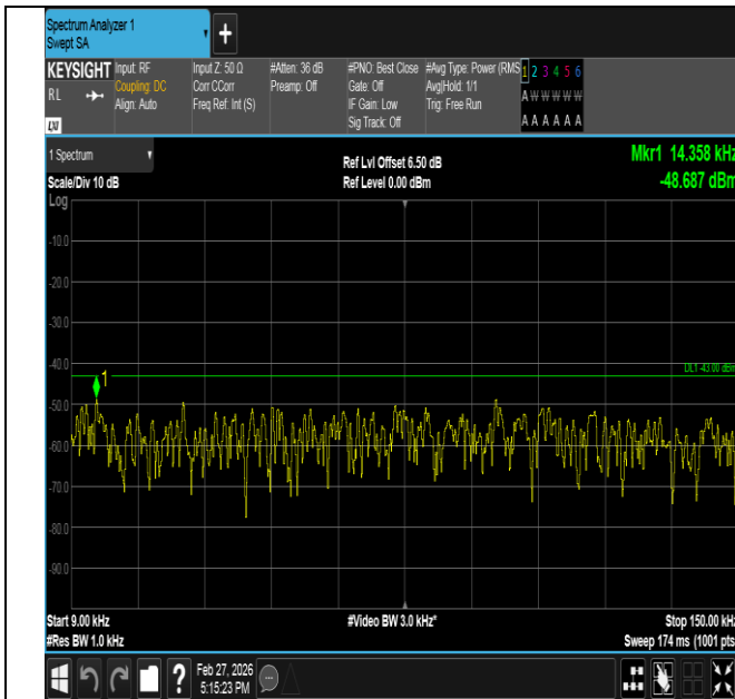
Band2-3MHz-QPSK-19185-15RB#0-0.009~0.15-PASS
