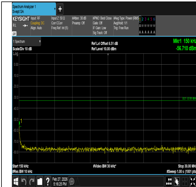
Band2-3MHz-16QAM-19185-15RB#0-0.15~30-PASS
