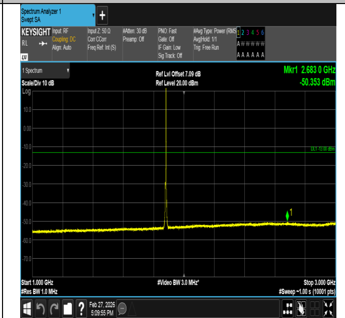
Band2-3MHz-16QAM-18900-1RB#14-1000~3000-PASS
