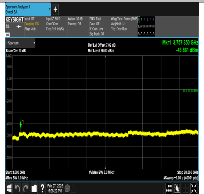
Band2-3MHz-16QAM-18900-1RB#0-3000~20000-PASS
