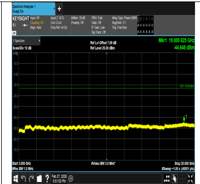
Band2-5MHz-16QAM-18625-25RB#0-3000~20000-PASS
