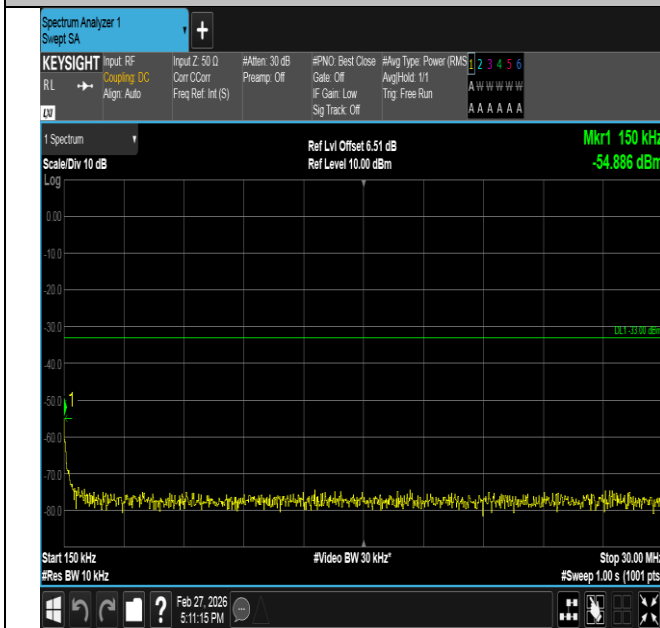
Band2-3MHz-16QAM-18900-15RB#0-0.15~30-PASS
