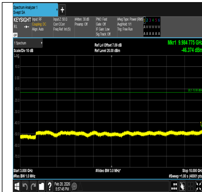
Band5-5MHz-QPSK-20425-25RB#0-3000~10000-PASS
