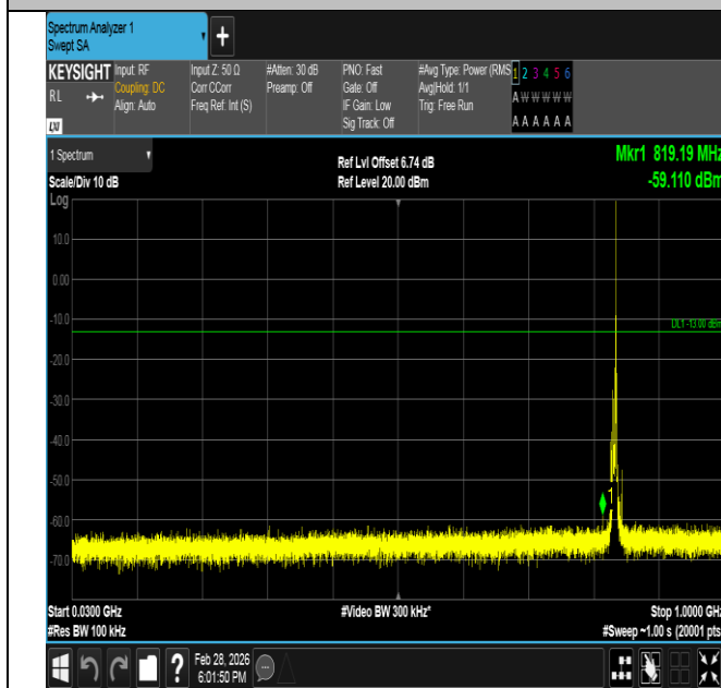
Band5-5MHz-16QAM-20525-1RB#24-30~1000-PASS
