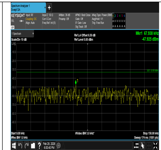
Band5-5MHz-QPSK-20525-1RB#24-0.009~0.15-PASS
