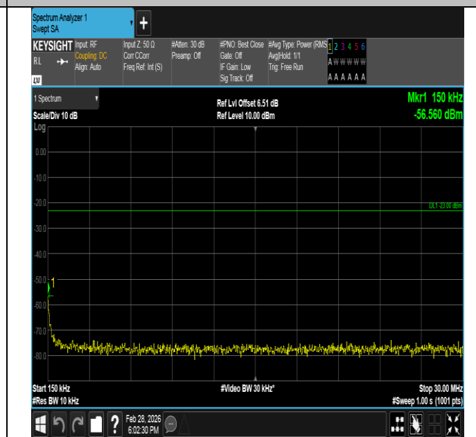
Band5-5MHz-QPSK-20525-25RB#0-0.15~30-PASS
