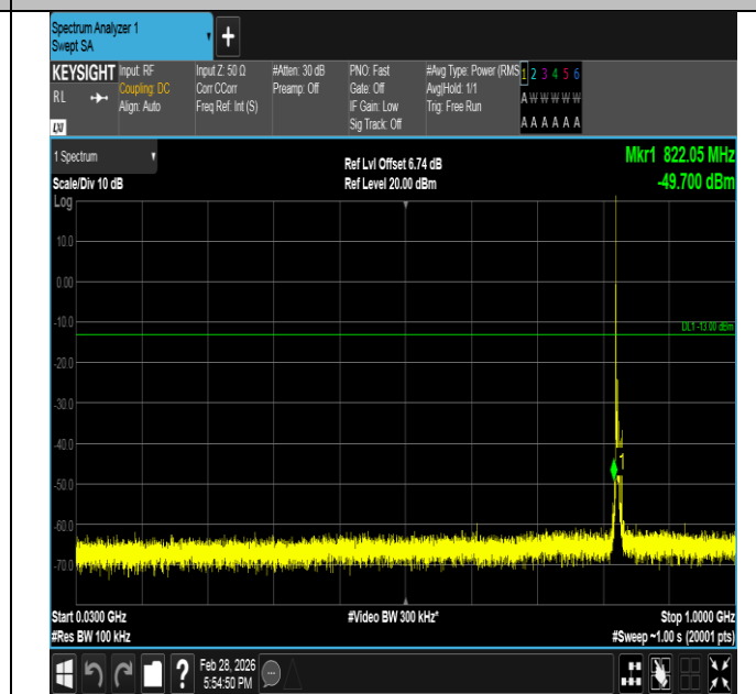
Band5-5MHz-16QAM-20425-1RB#0-30~1000-PASS
