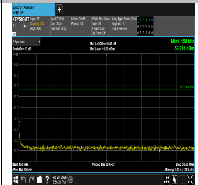
Band5-5MHz-16QAM-20425-1RB#24-0.15~30-PASS
