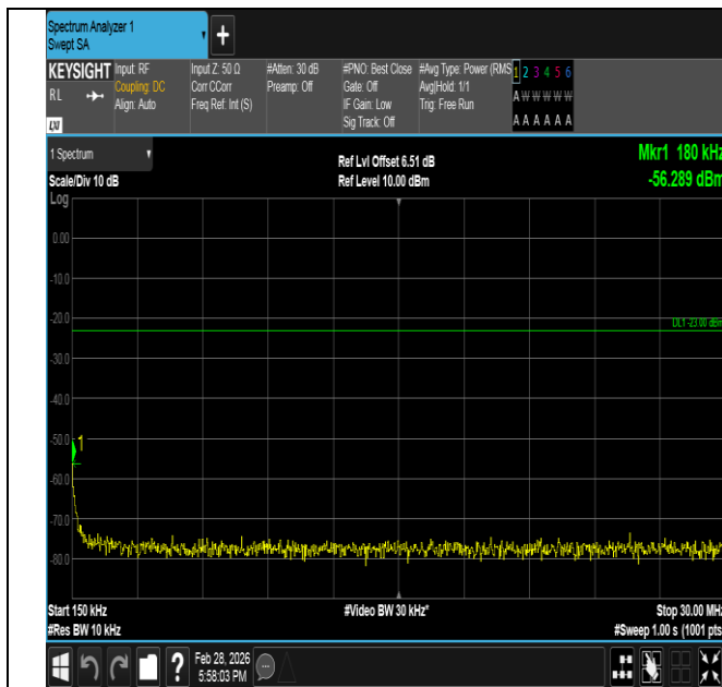
Band5-5MHz-16QAM-20425-25RB#0-0.15~30-PASS
