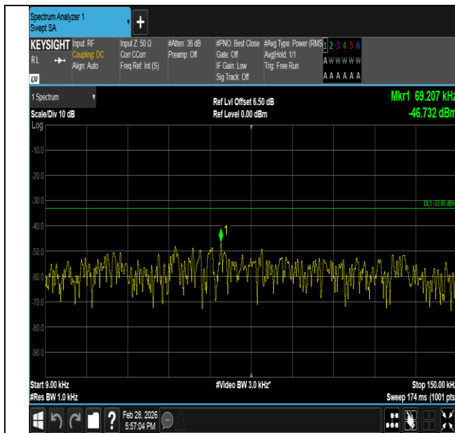
Band5-5MHz-QPSK-20425-25RB#0-0.009~0.15-PASS
