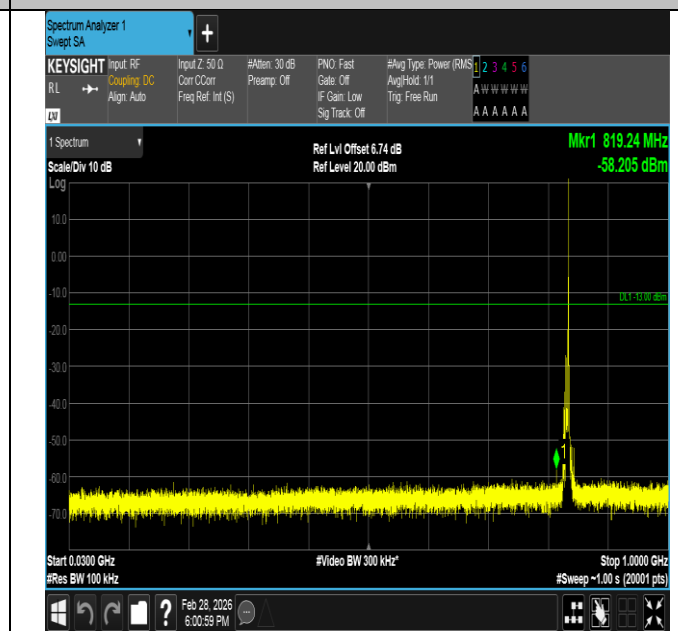
Band5-5MHz-QPSK-20525-1RB#24-30~1000-PASS
