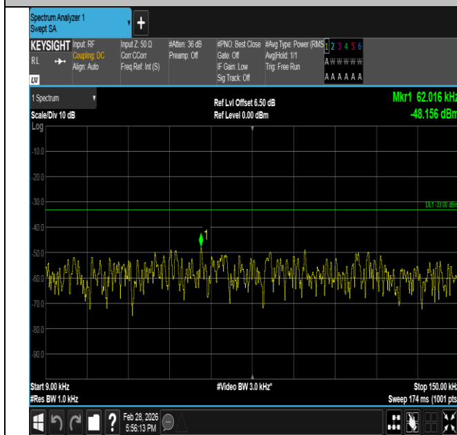
Band5-5MHz-16QAM-20425-1RB#24-0.009~0.15-PASS
