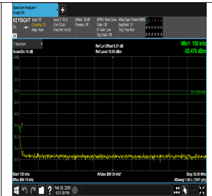
Band5-5MHz-16QAM-20525-1RB#24-0.15~30-PASS
