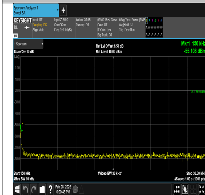
Band5-5MHz-QPSK-20525-1RB#24-0.15~30-PASS
