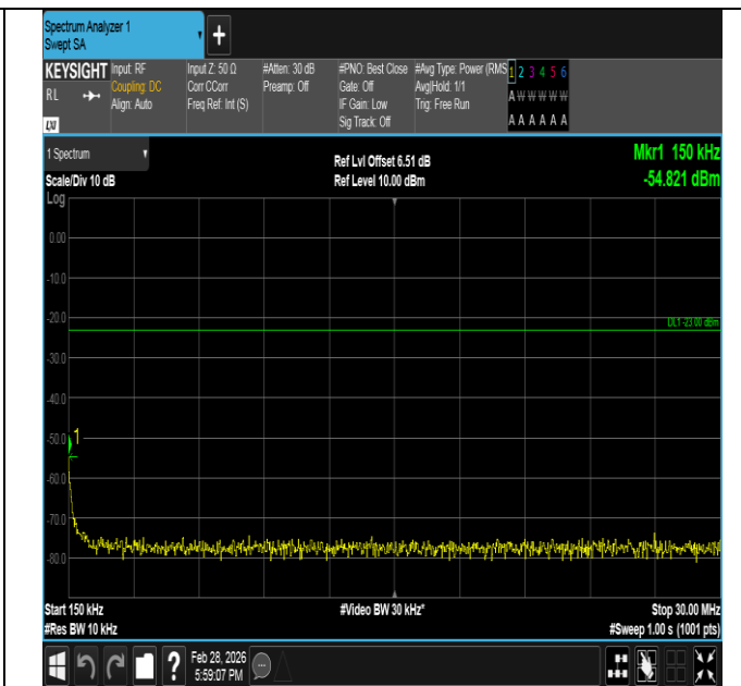
Band5-5MHz-QPSK-20525-1RB#0-0.15~30-PASS
