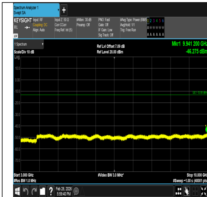
Band5-5MHz-QPSK-20525-1RB#0-3000~10000-PASS
