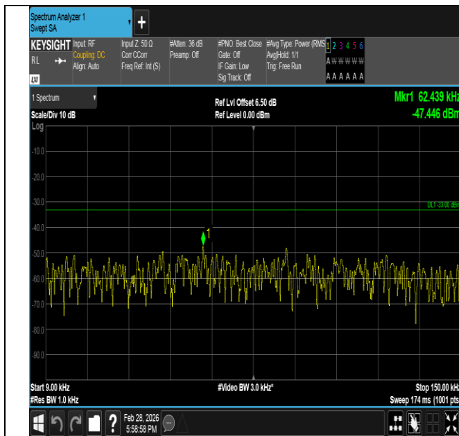
Band5-5MHz-QPSK-20525-1RB#0-0.009~0.15-PASS
