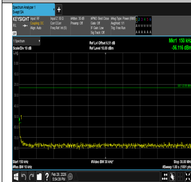
Band5-5MHz-16QAM-20425-1RB#0-0.15~30-PASS
