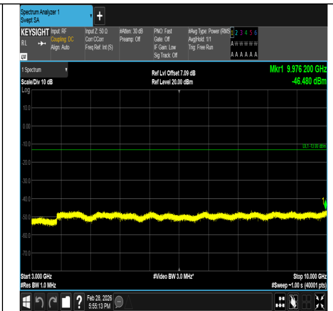
Band5-5MHz-16QAM-20425-1RB#0-3000~10000-PASS
