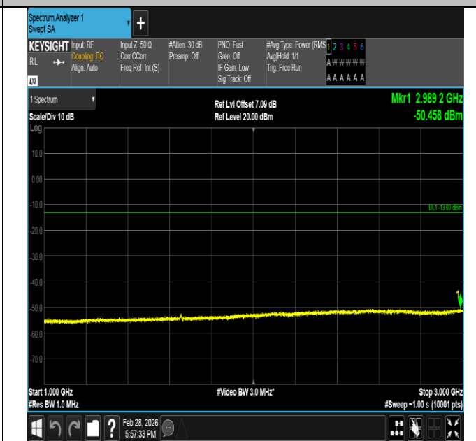
Band5-5MHz-QPSK-20425-25RB#0-1000~3000-PASS
