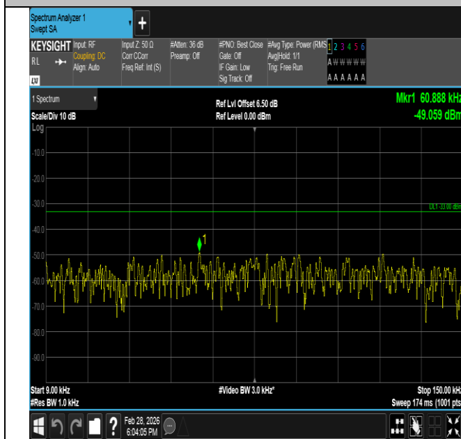
Band5-5MHz-QPSK-20625-1RB#0-0.009~0.15-PASS
