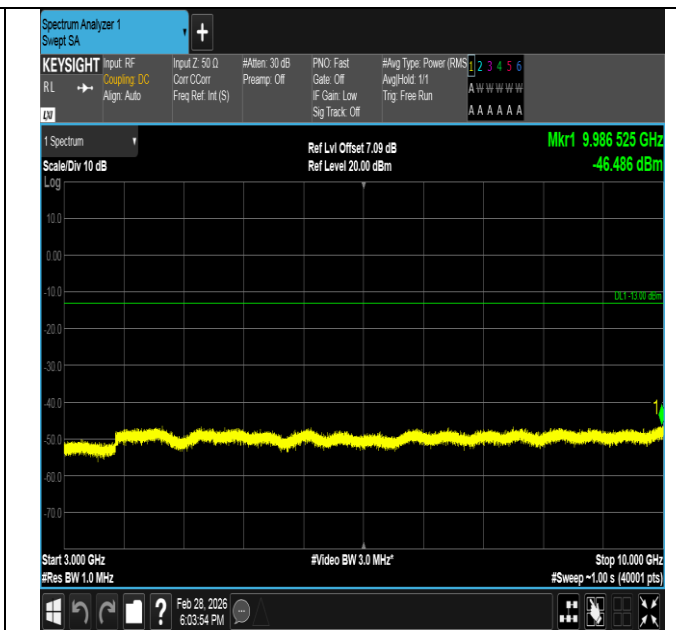
Band5-5MHz-16QAM-20525-25RB#0-3000~10000-PASS
