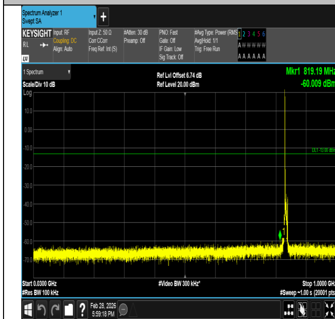
Band5-5MHz-QPSK-20525-1RB#0-30~1000-PASS
