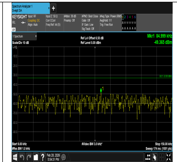
Band5-5MHz-16QAM-20425-1RB#0-0.009~0.15-PASS
