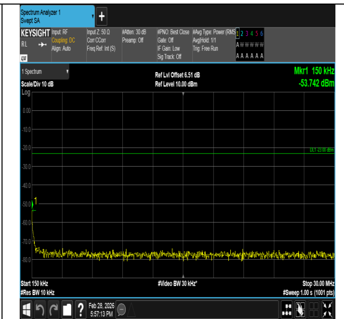
Band5-5MHz-QPSK-20425-25RB#0-0.15~30-PASS
