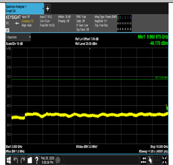
Band5-5MHz-16QAM-20425-25RB#0-3000~10000-PASS
