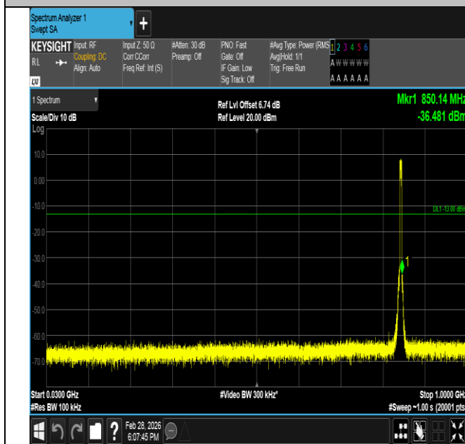
Band5-5MHz-QPSK-20625-25RB#0-30~1000-PASS
