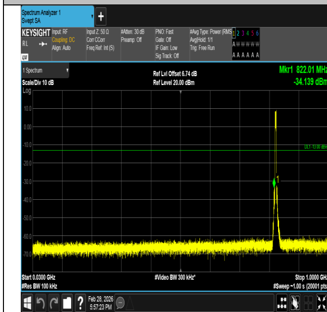
Band5-5MHz-QPSK-20425-25RB#0-30~1000-PASS
