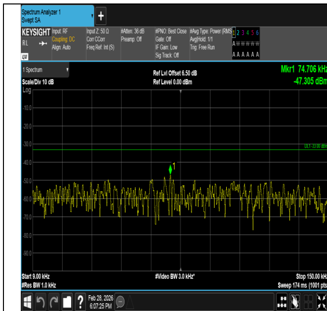
Band5-5MHz-QPSK-20625-25RB#0-0.009~0.15-PASS
