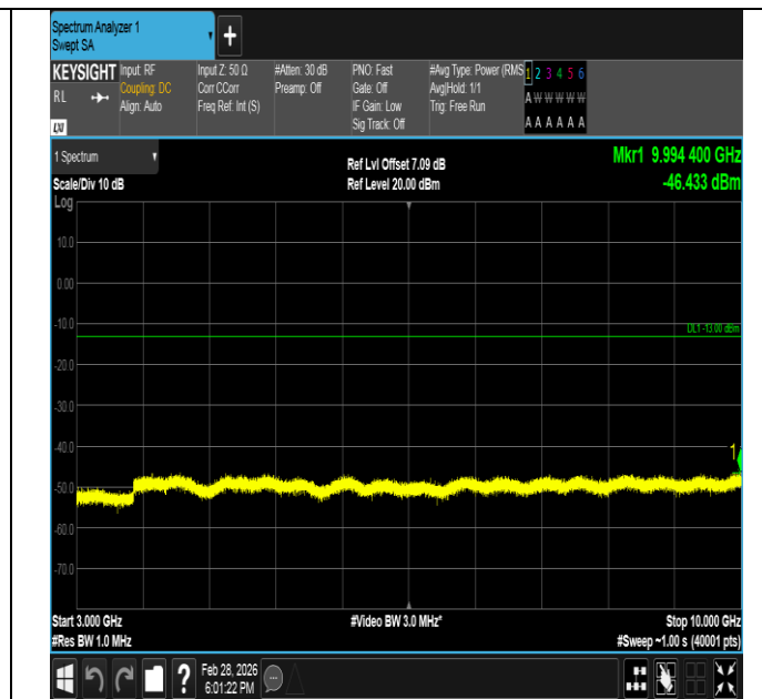
Band5-5MHz-QPSK-20525-1RB#24-3000~10000-PASS
