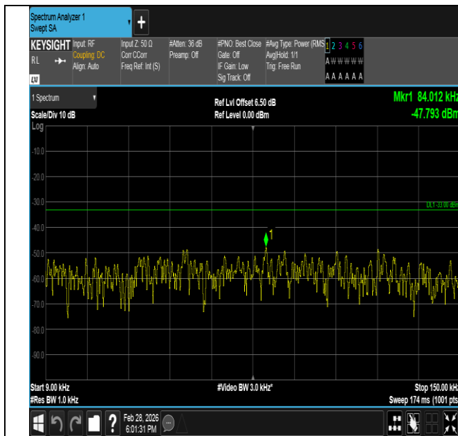
Band5-5MHz-16QAM-20525-1RB#24-0.009~0.15-PASS
