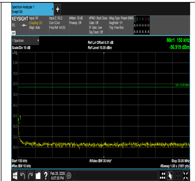
Band5-5MHz-QPSK-20625-25RB#0-0.15~30-PASS
