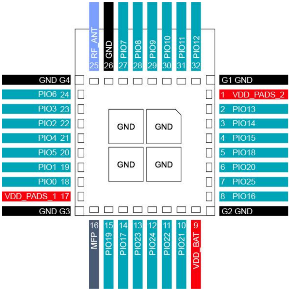
Figure 6: MQM711-0-50-0P Module Pin Map
