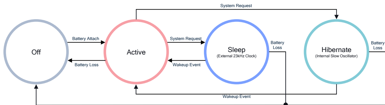
Figure 9: Power State Diagram
