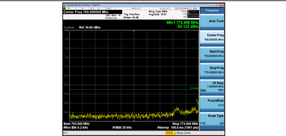
Band13-5MHz-QPSK-23205-1RB#0-Range3:763~775MHz
