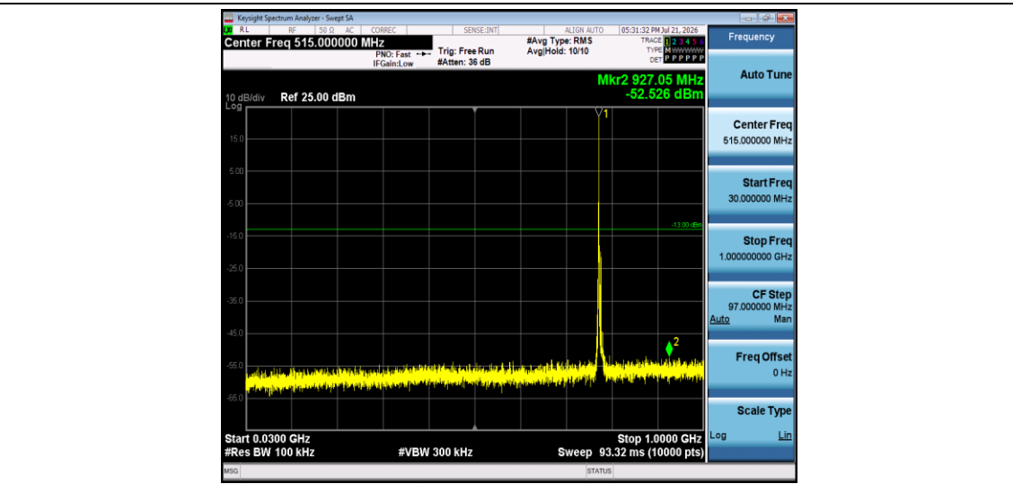
Band13-5MHz-QPSK-23205-1RB#0-Range1:30~1000MHz
