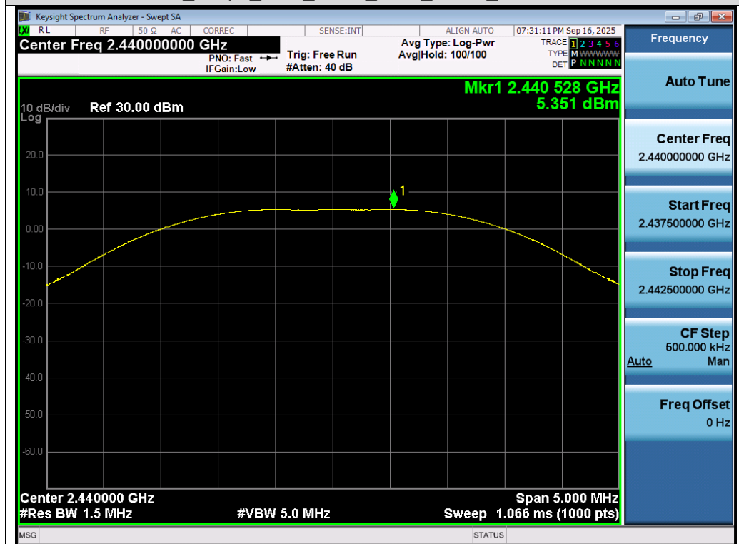
Test_Graph_SRD_ANT1_2440_GFSK_Peak Power
