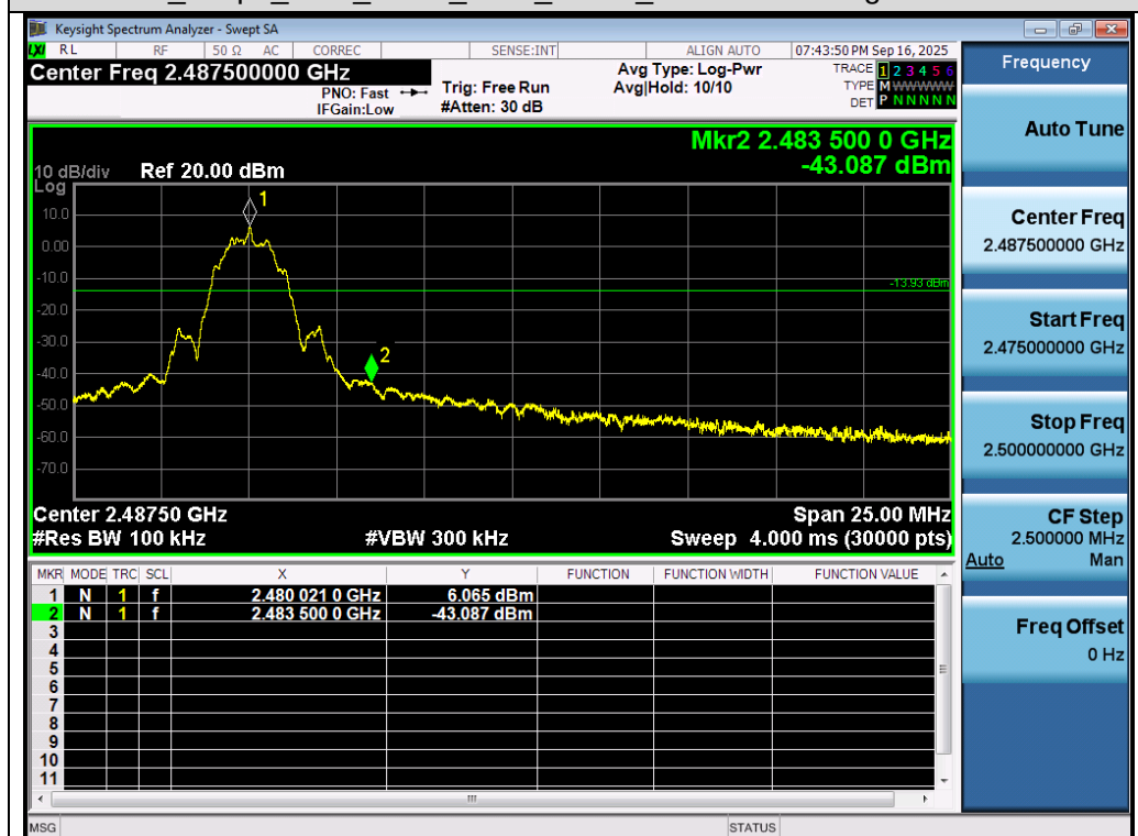
Test_Graph_SRD_ANT1_2480_GFSK_Higher Band Edge Emissions
