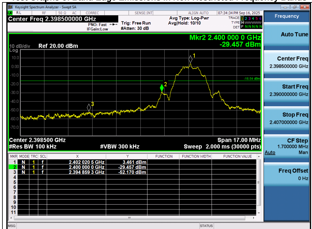
Test_Graph_SRD_ANT1_2402_GFSK_Lower Band Edge Emissions
