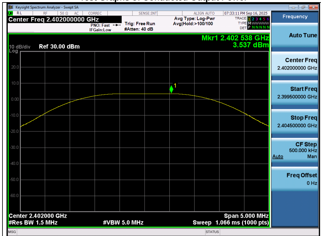
Test_Graph_SRD_ANT1_2402_GFSK_Peak Power
