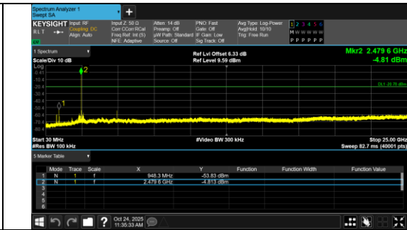
30.0 MHz - 25000.0 MHz BLE 2M_Channel 39
