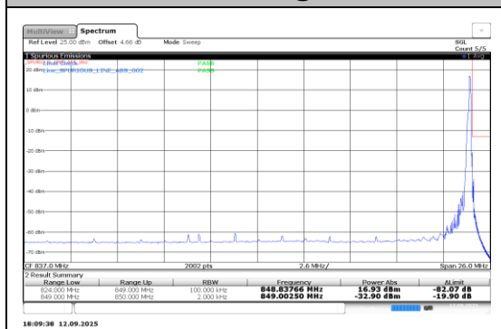
Band5-0.18-BPSK-20648-1@11-15kHz-PASS
