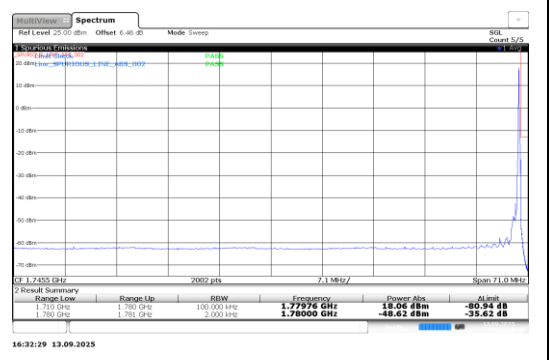
Band66-0.18-QPSK-132670-1@0-15kHz-PASS
