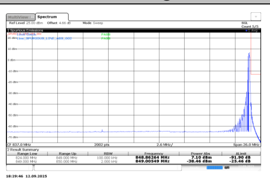
Band5-0.18-BPSK-20648-12@0-15kHz-PASS
