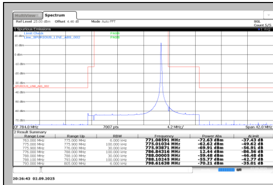
Band13-0.18-QPSK-23279-1@0-15kHz-PASS
