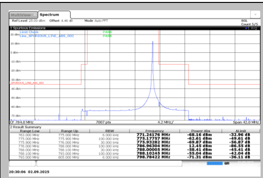
Band13-0.18-QPSK-23279-1@11-15kHz-PASS
