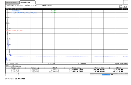
Band66-0.18-BPSK-131974-12@0-15kHz-PASS
