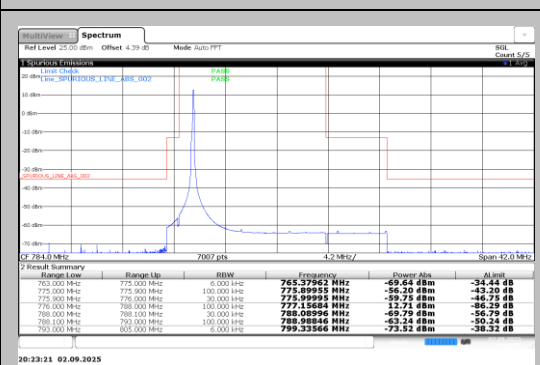
Band13-0.18-QPSK-23181-1@11-15kHz-PASS
