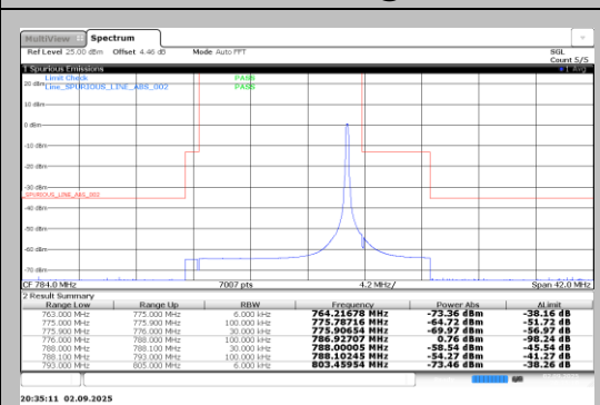
Band13-0.18-BPSK-23279-12@0-15kHz-PASS
