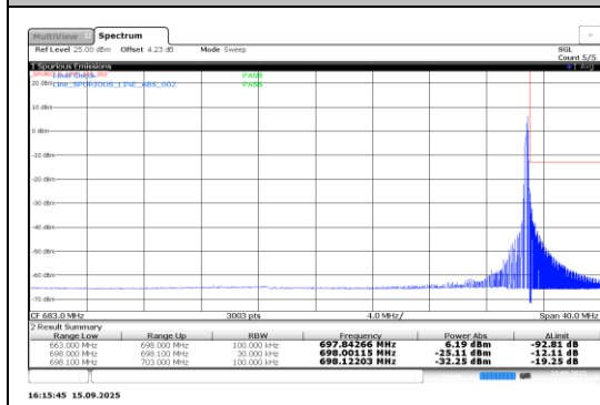
Band71-0.18-BPSK-133470-12@0-15kHz-PASS
