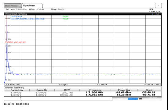
Band66-0.18-BPSK-131974-1@11-15kHz-PASS
