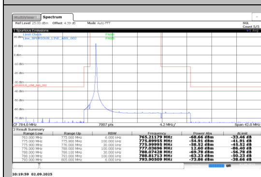
Band13-0.18-QPSK-23181-1@0-15kHz-PASS
