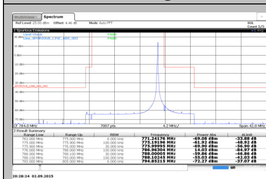
Band13-0.18-BPSK-23279-1@11-15kHz-PASS
