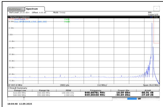
Band5-0.18-QPSK-20648-1@0-15kHz-PASS
