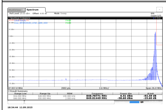
Band5-0.18-QPSK-20648-12@0-15kHz-PASS
