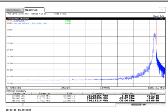
Band12-0.18-BPSK-23178-1@0-15kHz-PASS
