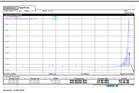
Band5-0.18-QPSK-20648-1@11-15kHz-PASS
