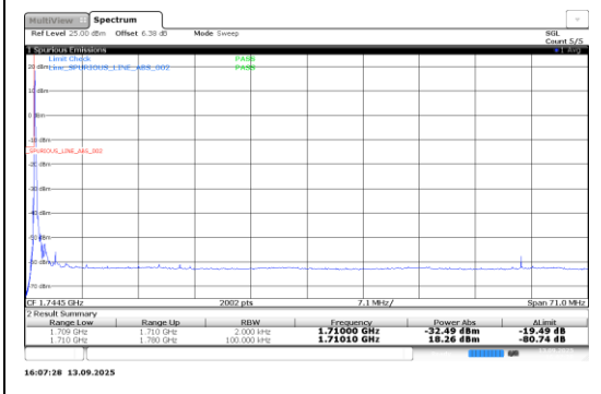
Band66-0.18-BPSK-131974-1@0-15kHz-PASS
