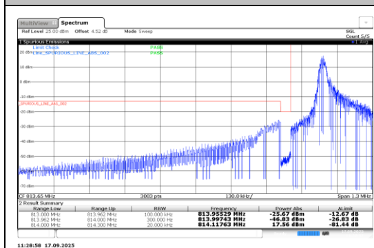
Band26-0.18-QPSK-26692-1@0-15kHz-PASS
