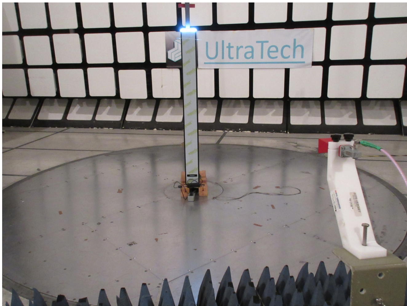
Radiated Emissions at 3 m, 18 – 25 GHz
