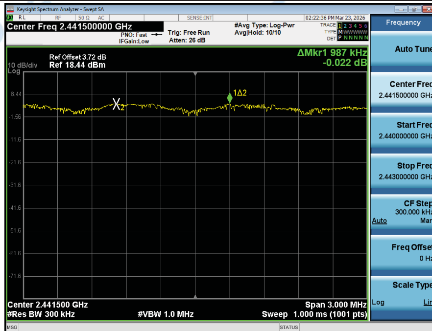
Carrier_Frequencies_Separation_(Hopping)_NVNT_ANT1_2-DH5_Hopping
