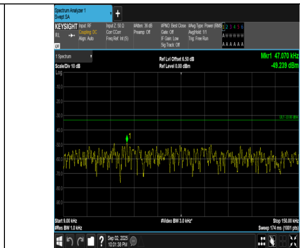
Band5-3MHz-16QAM-20635-1RB#0-0.009~0.15-PASS
