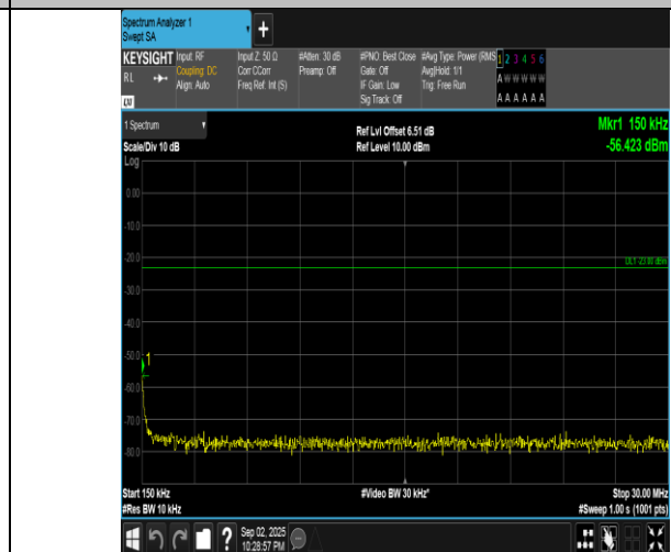
Band5-5MHz-QPSK-20425-25RB#0-0.15~30-PASS
