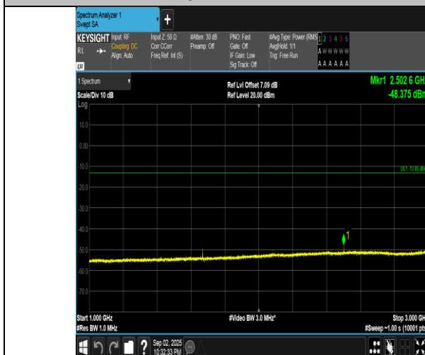
Band5-5MHz-16QAM-20525-1RB#0-1000~3000-PASS
