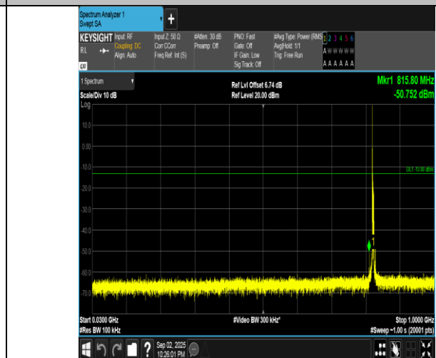
Band5-5MHz-16QAM-20425-1RB#0-30~1000-PASS
