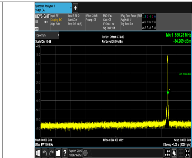
Band5-3MHz-16QAM-20635-15RB#0-30~1000-PASS
