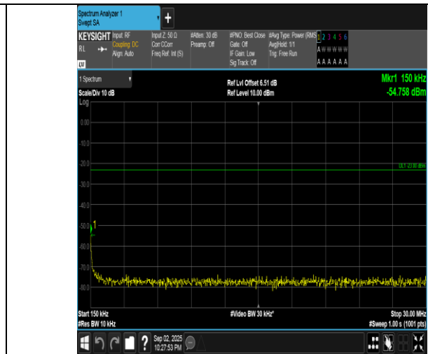
Band5-5MHz-16QAM-20425-1RB#24-0.15~30-PASS
