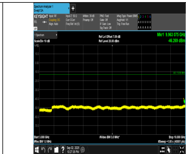
Band5-5MHz-QPSK-20425-1RB#24-3000~10000-PASS
