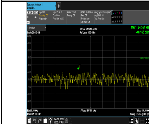
Band5-5MHz-QPSK-20525-1RB#0-0.009-0.15-PASS
