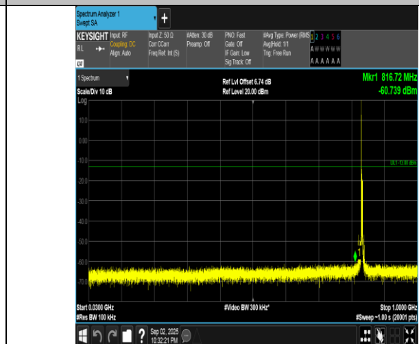
Band5-5MHz-16QAM-20525-1RB#0-30~1000-PASS
