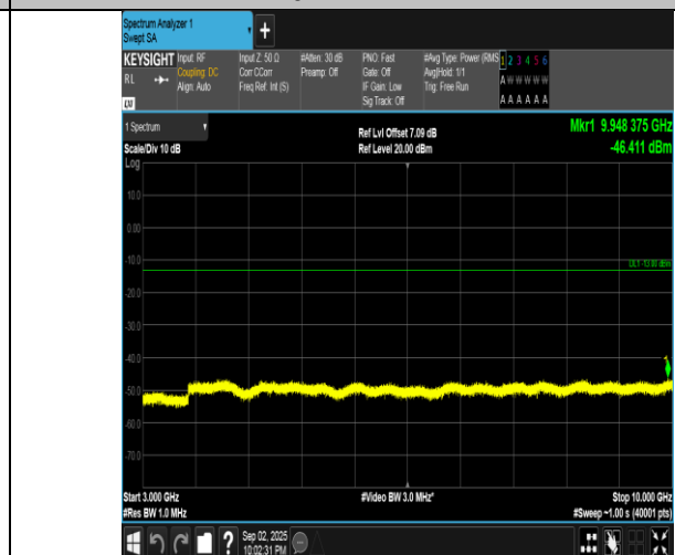
Band5-3MHz-16QAM-20635-1RB#0-3000~10000-PASS
