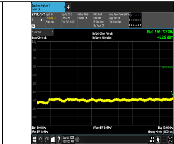
Band5-3MHz-QPSK-20635-1RB#14-3000~10000-PASS
