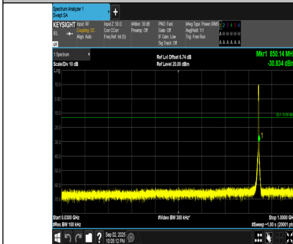
Band5-3MHz-QPSK-20635-15RB#0-30~1000-PASS
