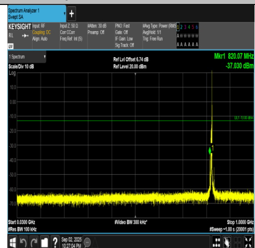
Band5-5MHz-QPSK-20425-1RB#24-30~1000-PASS
