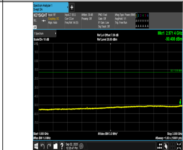
Band5-5MHz-QPSK-20525-25RB#0-1000~3000-PASS
