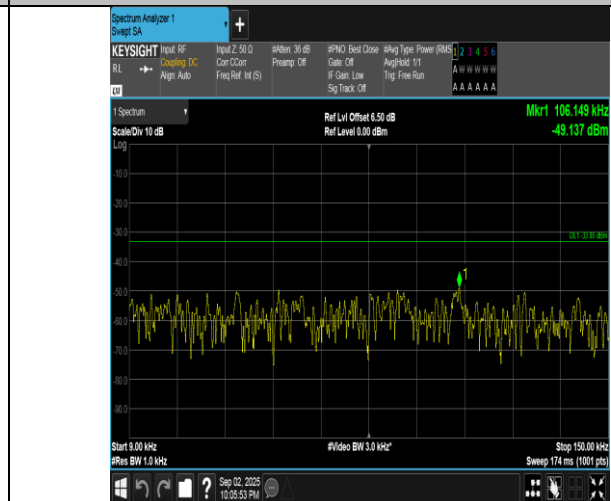
Band5-3MHz-16QAM-20635-15RB#0-0.009~0.15-PASS
