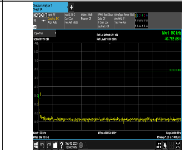
Band5-3MHz-QPSK-20635-15RB#0-0.15~30-PASS
