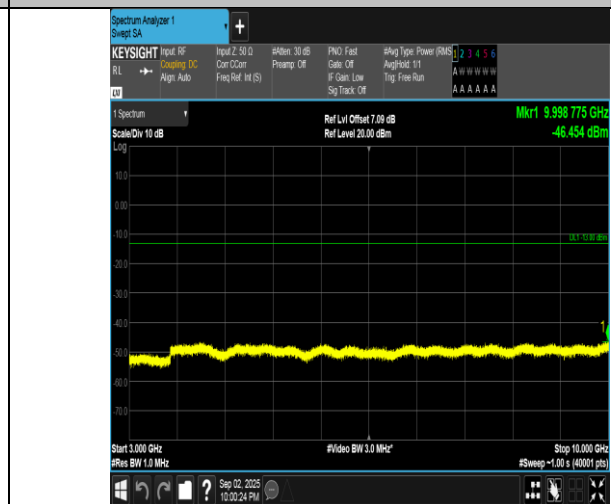
Band5-3MHz-16QAM-20525-15RB#0-3000-10000-PASS
