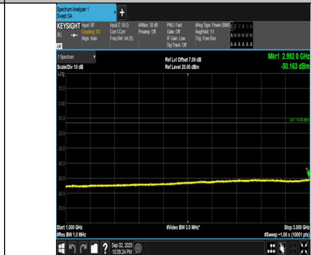
Band5-3MHz-QPSK-20635-15RB#0-1000~3000-PASS
