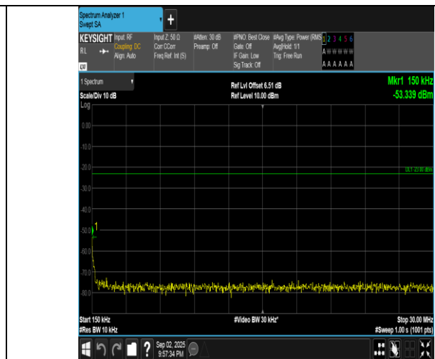
Band5-3MHz-16QAM-20525-1RB#14-0.15~30-PASS
