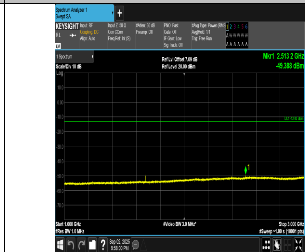
Band5-3MHz-16QAM-20525-1RB#14-1000~3000-PASS
