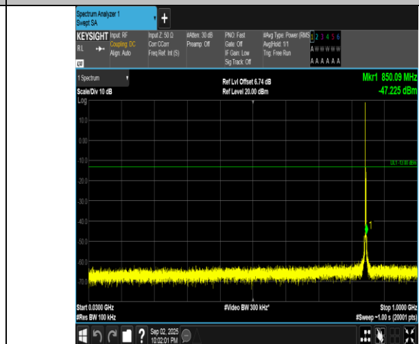
Band5-3MHz-16QAM-20635-1RB#0-30~1000-PASS
