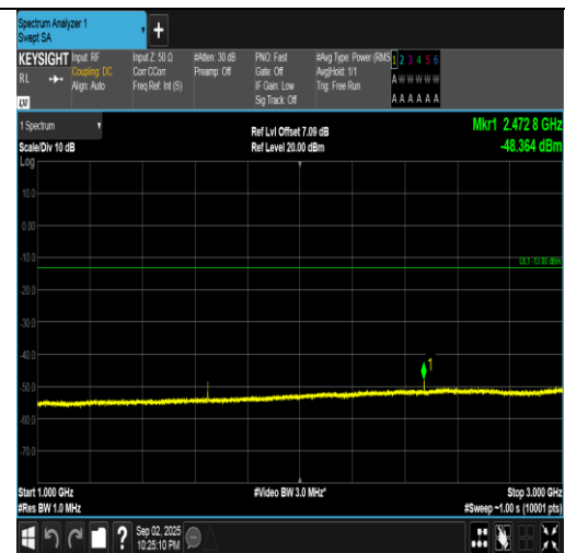
Band5-5MHz-QPSK-20425-1RB#0-1000~3000-PASS
