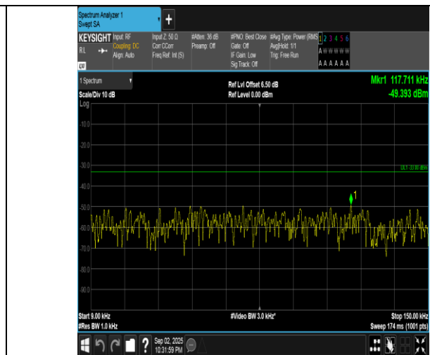
Band5-5MHz-16QAM-20525-1RB#0-0.009~0.15-PASS
