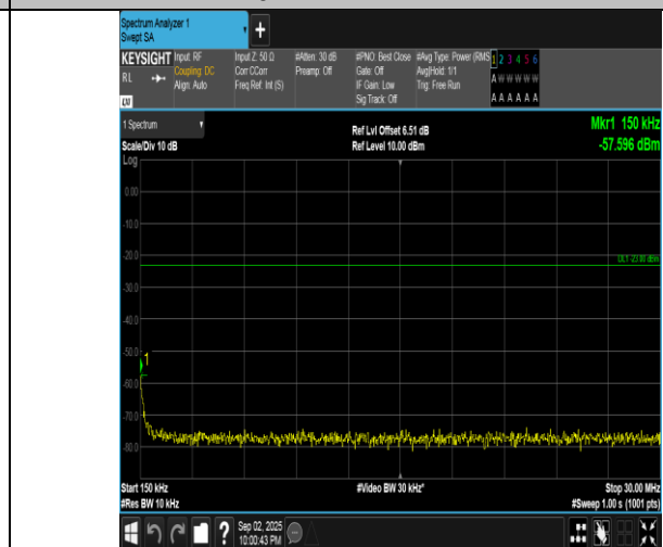
Band5-3MHz-QPSK-20635-1RB#0-0.15-30-PASS
