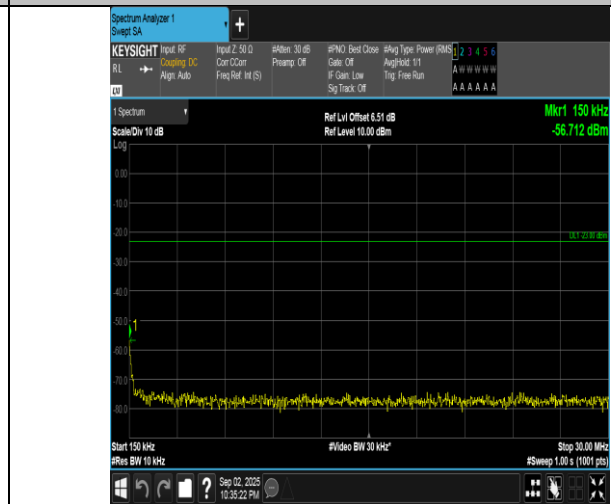
Band5-5MHz-QPSK-20525-25RB#0-0.15~30-PASS
