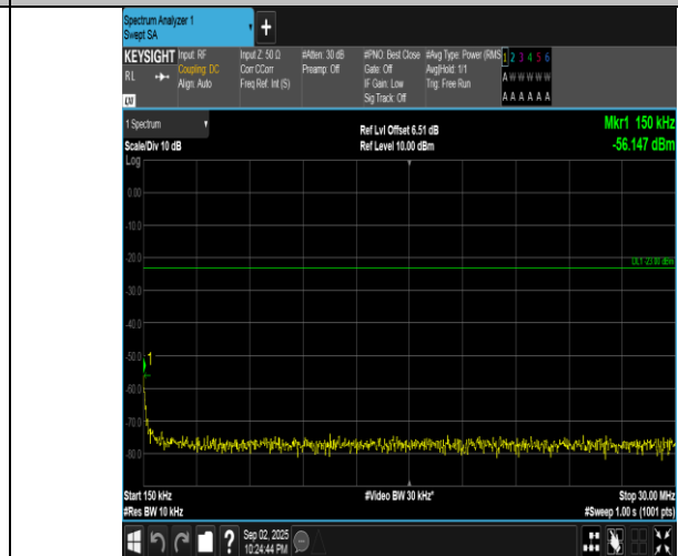
Band5-5MHz-QPSK-20425-1RB#0-0.15~30-PASS
