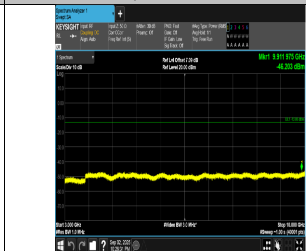
Band5-5MHz-16QAM-20425-1RB#0-3000~10000-PASS
