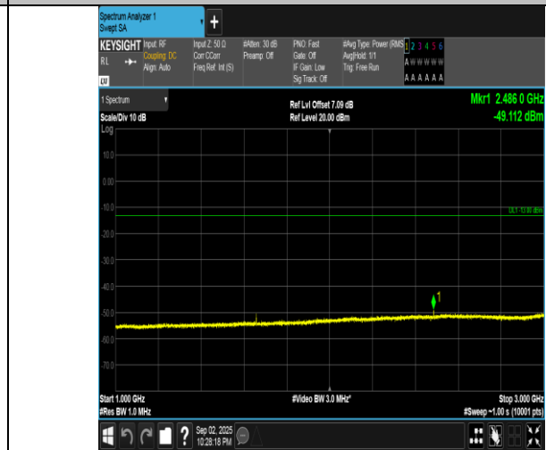
Band5-5MHz-16QAM-20425-1RB#24-1000~3000-PASS
