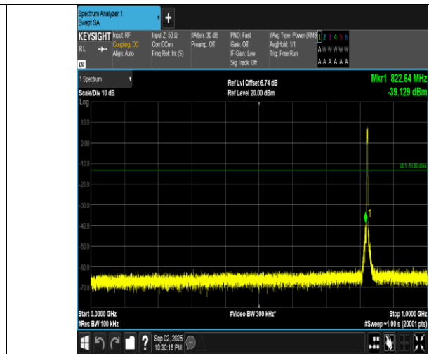
Band5-5MHz-16QAM-20425-25RB#0-30-1000-PASS
