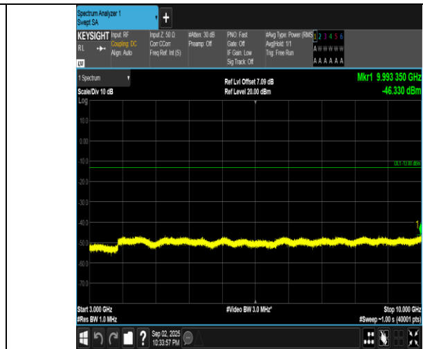
Band5-5MHz-QPSK-20525-1RB#24-3000~10000-PASS
