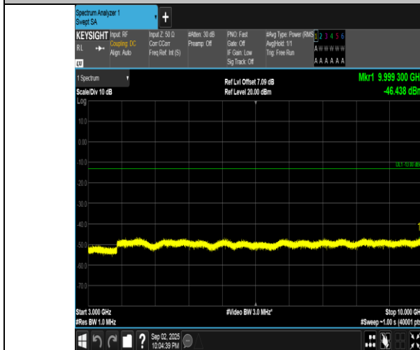
Band5-3MHz-16QAM-20635-1RB#14-3000~10000-PASS
