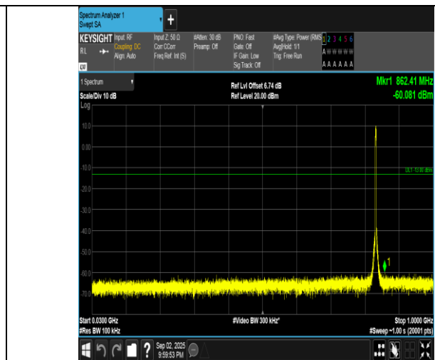
Band5-3MHz-16QAM-20525-15RB#0-30-1000-PASS
