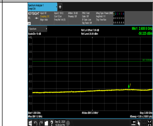
Band5-5MHz-QPSK-20425-25RB#0-1000~3000-PASS
