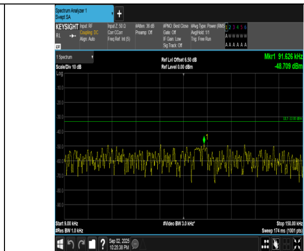
Band5-5MHz-16QAM-20425-1RB#0-0.009~0.15-PASS
