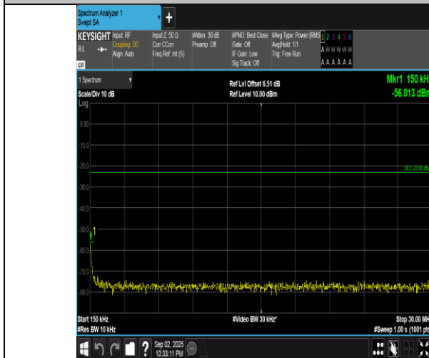
Band5-5MHz-QPSK-20525-1RB#24-0.15~30-PASS
