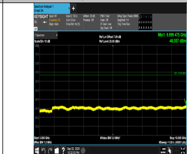
Band5-5MHz-16QAM-20525-1RB#0-3000~10000-PASS
