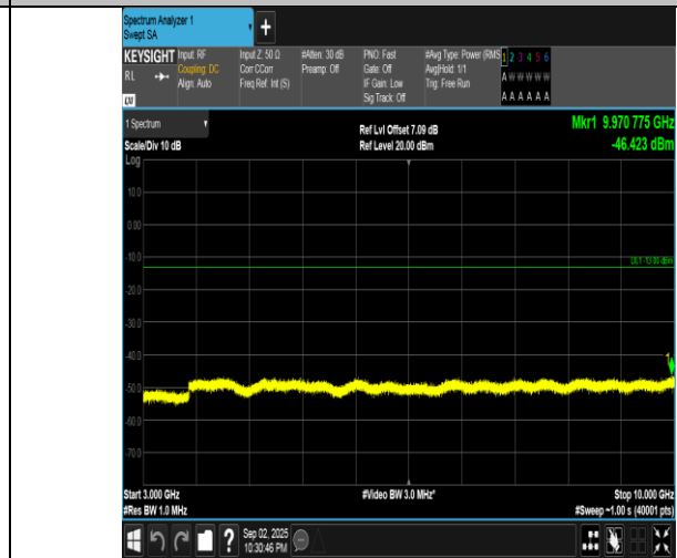
Band5-5MHz-16QAM-20425-25RB#0-3000-10000-PASS
