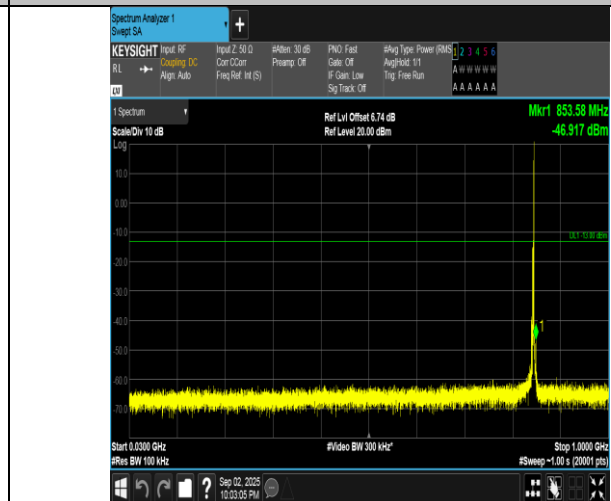
Band5-3MHz-QPSK-20635-1RB#14-30~1000-PASS
