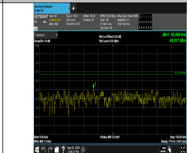
Band5-3MHz-16QAM-20525-15RB#0-0.009~0.15-PASS
