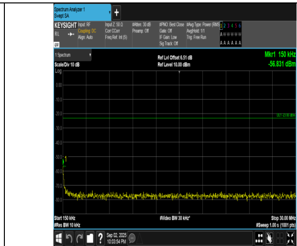
Band5-3MHz-16QAM-20635-1RB#14-0.15~30-PASS
