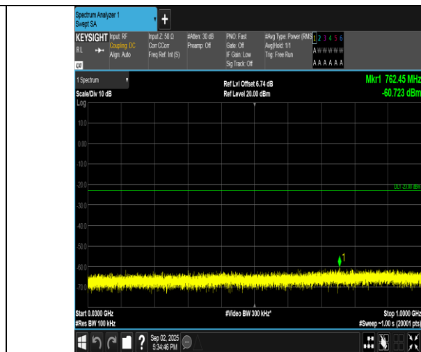
Band4-3MHz-QPSK-20385-1RB#14-30~1000-PASS
