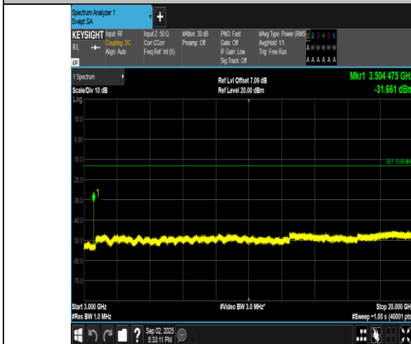
Band4-3MHz-QPSK-20385-1RB#0-3000~20000-PASS
