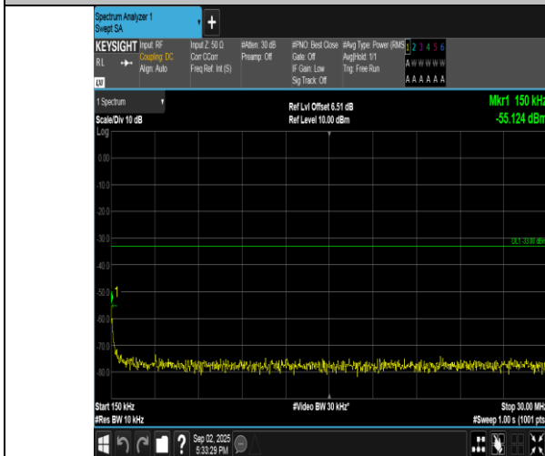
Band4-3MHz-16QAM-20385-1RB#0-0.15~30-PASS
