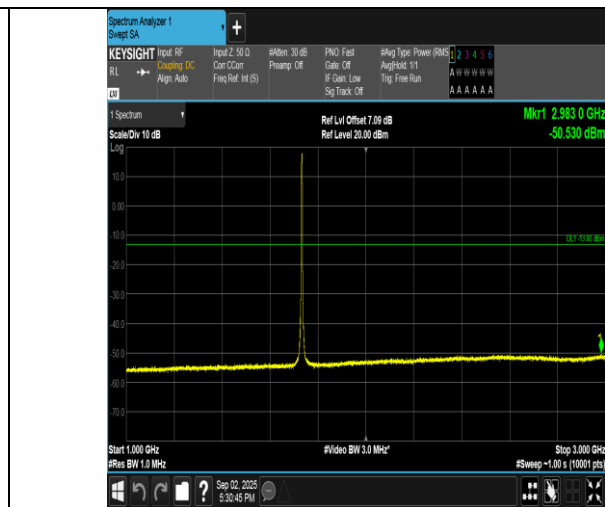
Band4-3MHz-QPSK-20175-15RB#0-1000~3000-PASS
