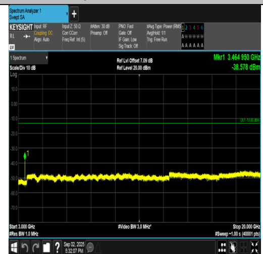
Band4-3MHz-16QAM-20175-15RB#0-3000~20000-PASS
