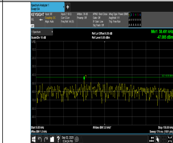
Band4-3MHz-QPSK-20385-1RB#14-0.009~0.15-PASS
