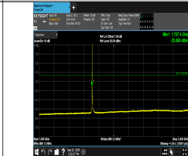
Band4-3MHz-16QAM-19965-1RB#14-1000~3000-PASS
