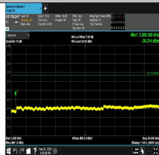
Band4-1.4MHz-16QAM-20393-6RB#0-3000~20000-PASS
