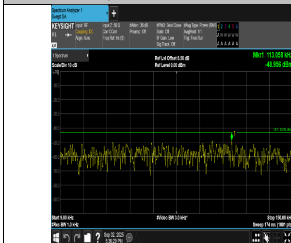
Band4-3MHz-QPSK-20385-15RB#0-0.009~0.15-PASS
