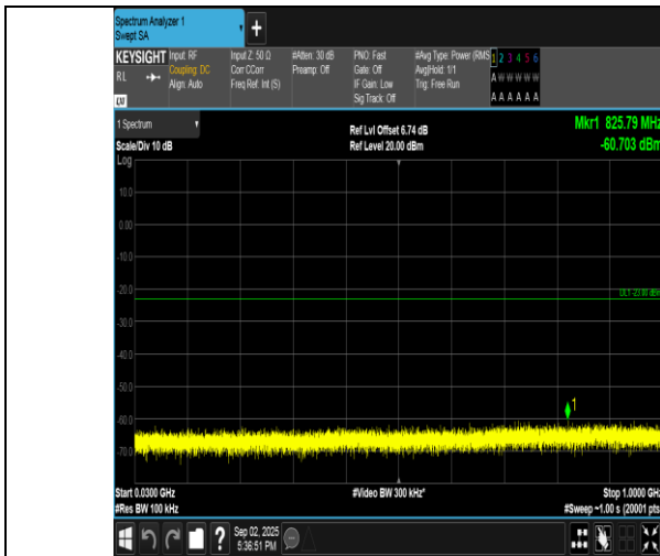
Band4-3MHz-QPSK-20385-15RB#0-30~1000-PASS
