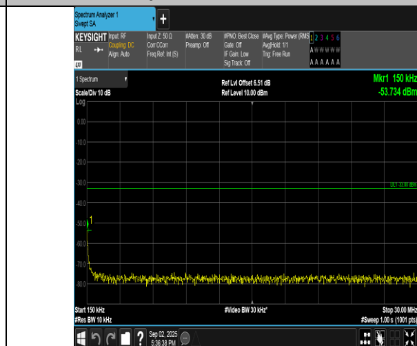
Band4-3MHz-QPSK-20385-15RB#0-0.15~30-PASS
