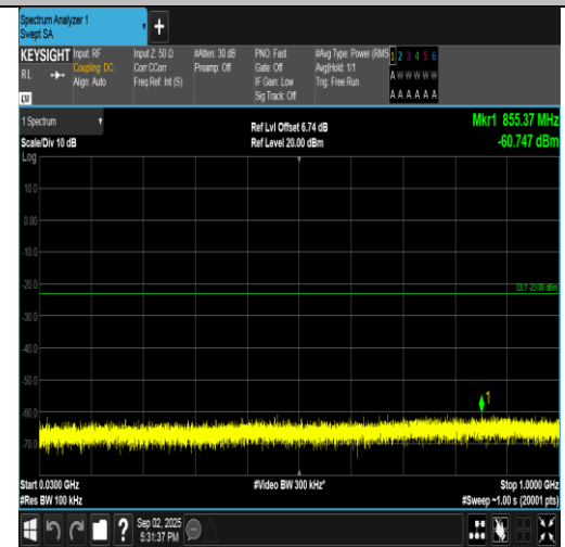
Band4-3MHz-16QAM-20175-15RB#0-30~1000-PASS
