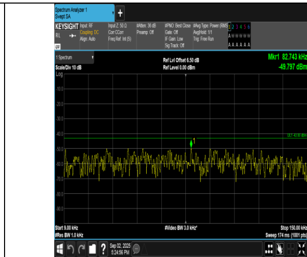
Band4-3MHz-16QAM-19965-15RB#0-0.009~0.15-PASS
