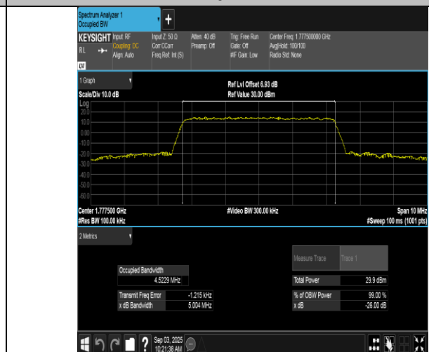
Band66-5MHz-16QAM-132647-25RB#0-PASS
