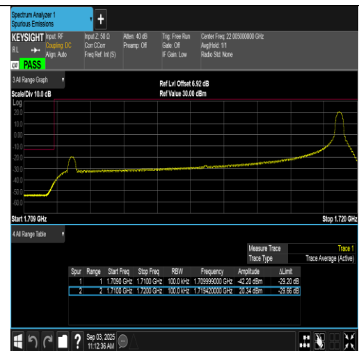
Band66-10MHz-QPSK-132022-1RB#49-PASS
