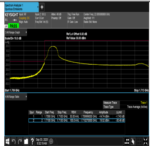
Band66-3MHz-16QAM-131987-1RB#0-PASS
