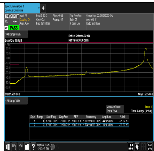
Band66-15MHz-QPSK-132047-1RB#74-PASS
