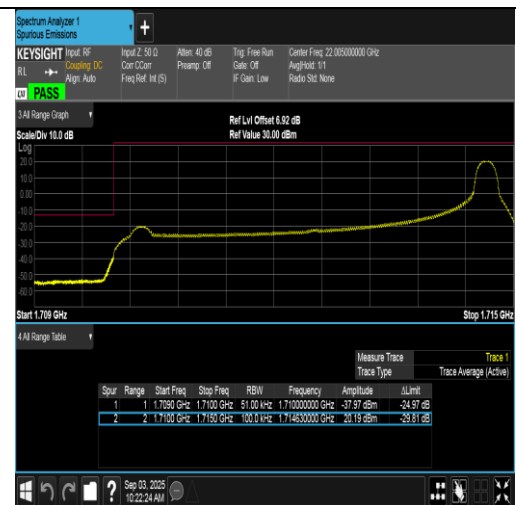
Band66-5MHz-QPSK-131997-1RB#24-PASS
