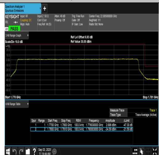
Band66-10MHz-16QAM-132622-50RB#0-PASS
