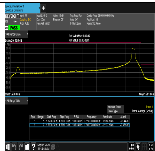
Band66-10MHz-QPSK-132622-1RB#49-PASS
