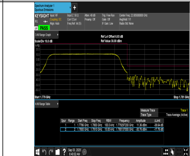
Band66-1.4MHz-16QAM-132665-6RB#0-PASS
