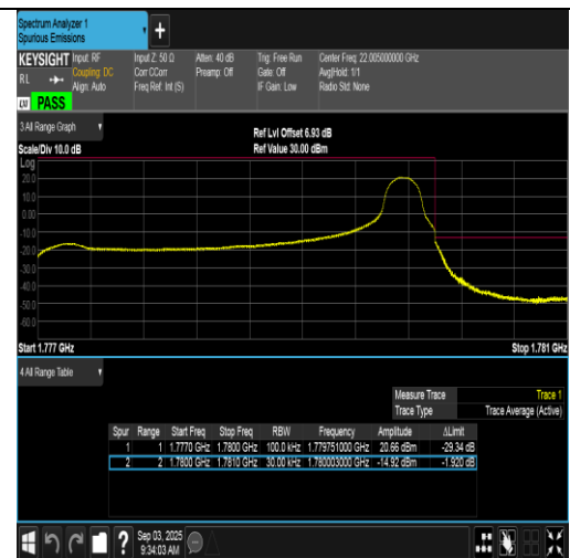
Band66-3MHz-QPSK-132657-1RB#14-PASS
