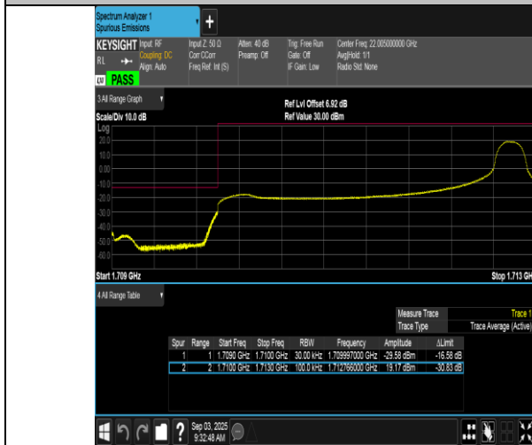
Band66-3MHz-16QAM-131987-1RB#14-PASS
