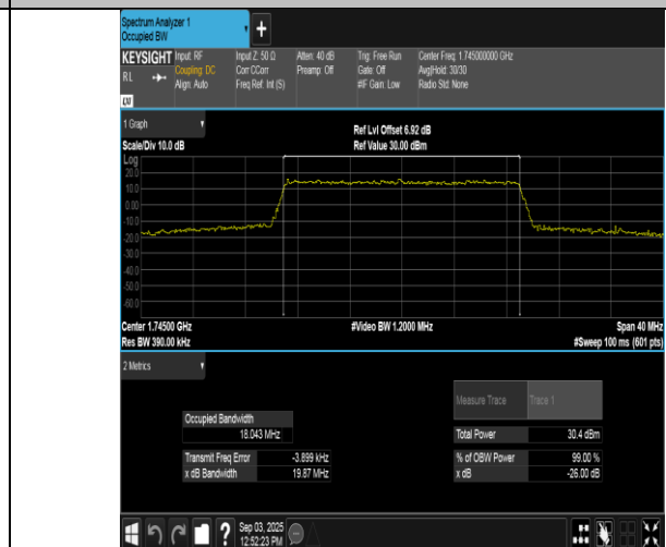
Band66-20MHz-16QAM-132322-100RB#0-PASS
