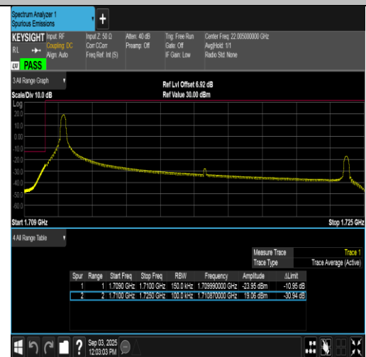
Band66-15MHz-16QAM-132047-1RB#0-PASS
