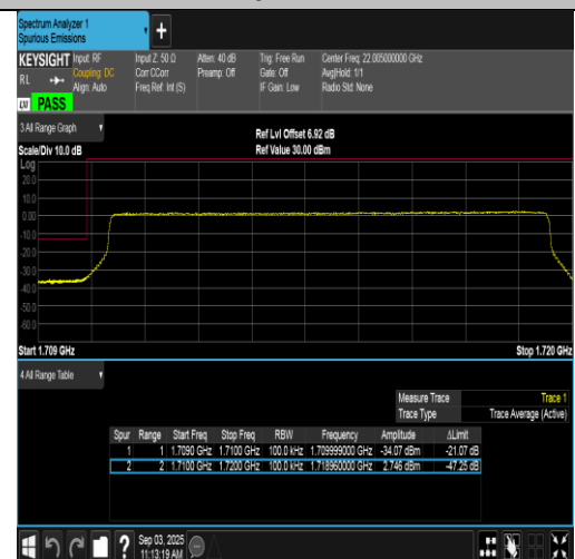
Band66-10MHz-16QAM-132022-50RB#0-PASS
