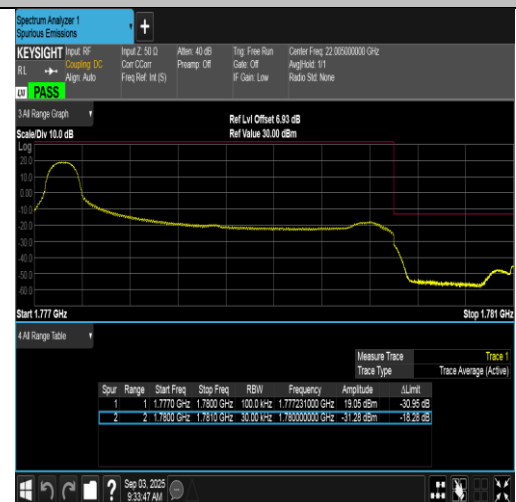
Band66-3MHz-16QAM-132657-1RB#0-PASS
