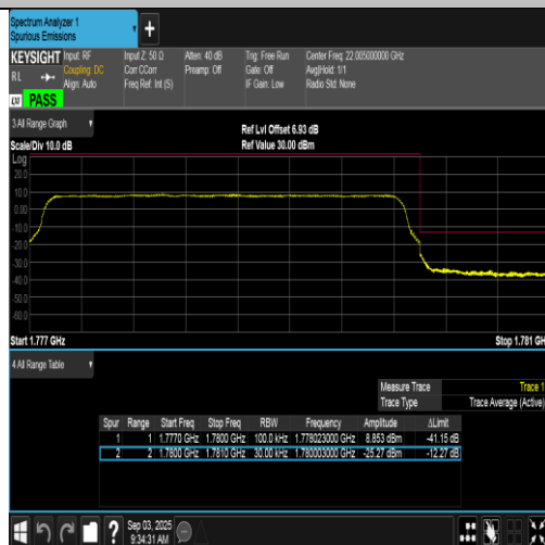
Band66-3MHz-QPSK-132657-15RB#0-PASS
