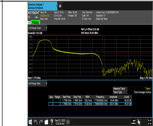
Band66-1.4MHz-16QAM-132665-1RB#0-PASS
