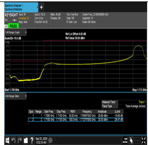
Band66-3MHz-QPSK-131987-1RB#14-PASS
