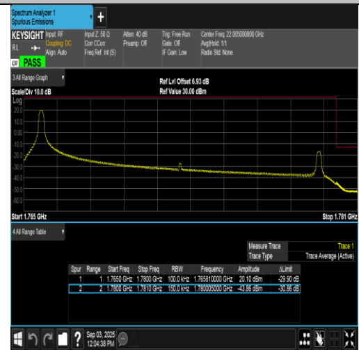
Band66-15MHz-16QAM-132597-1RB#0-PASS
