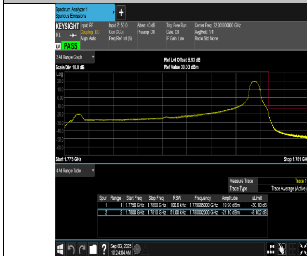
Band66-5MHz-16QAM-132647-1RB#24-PASS
