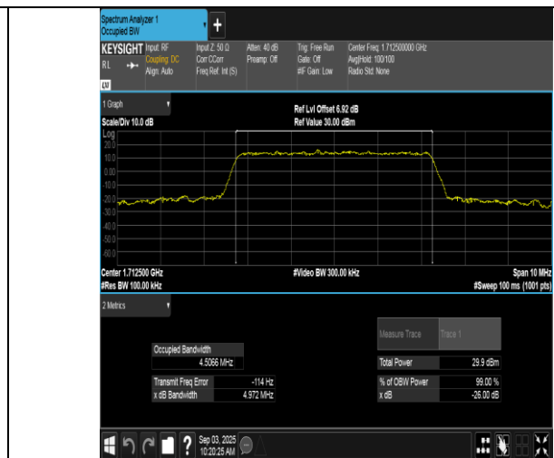
Band66-5MHz-16QAM-131997-25RB#0-PASS
