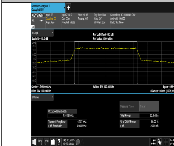
Band66-5MHz-QPSK-132322-25RB#0-PASS
