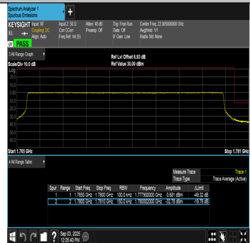
Band66-15MHz-16QAM-132597-75RB#0-PASS
