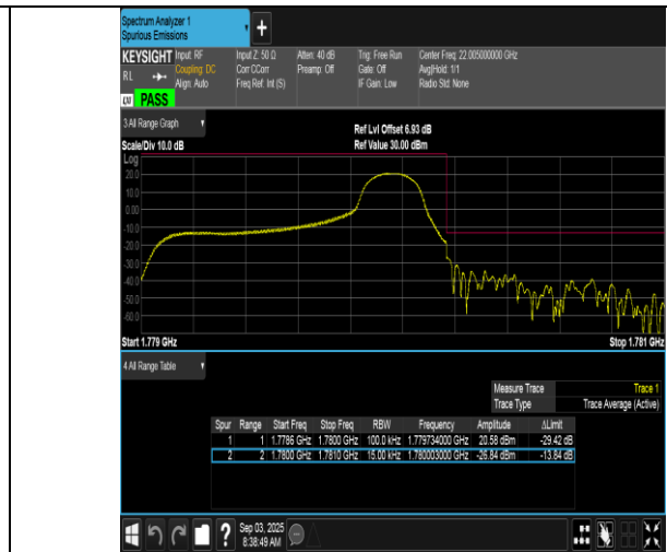
Band66-1.4MHz-QPSK-132665-1RB#5-PASS
