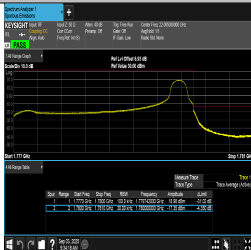
Band66-3MHz-16QAM-132657-1RB#14-PASS
