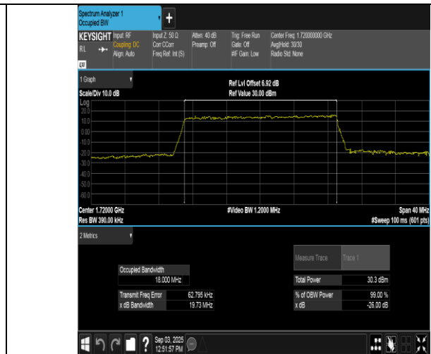
Band66-20MHz-16QAM-132072-100RB#0-PASS
