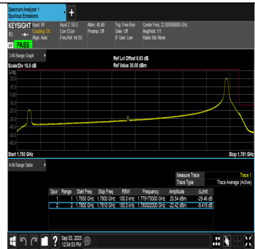
Band66-15MHz-QPSK-132597-1RB#74-PASS
