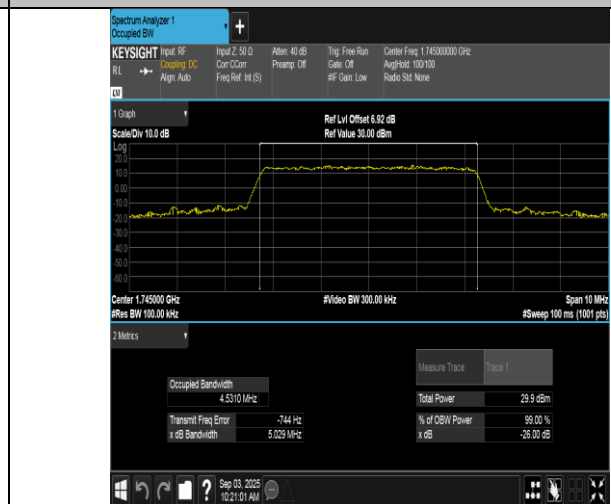
Band66-5MHz-16QAM-132322-25RB#0-PASS
