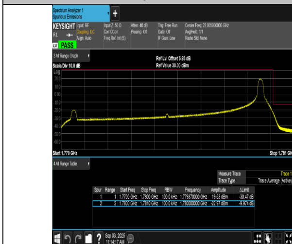
Band66-10MHz-16QAM-132622-1RB#49-PASS
