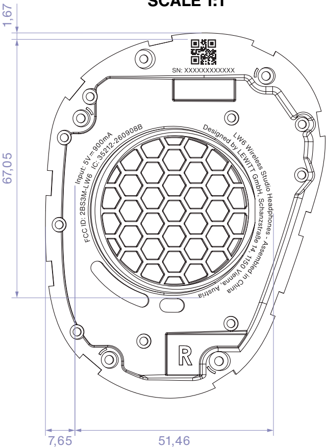
Dimensions in mm SCALE 1:1
