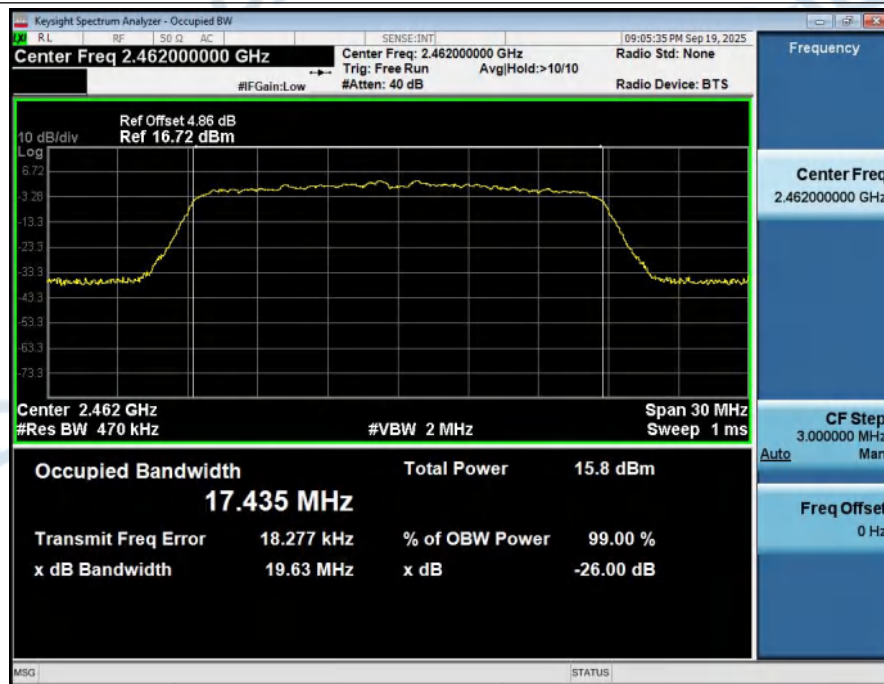
99%_Occupied_Bandwidth_NVNT_ANT2_802_11n(HT20)_2462
