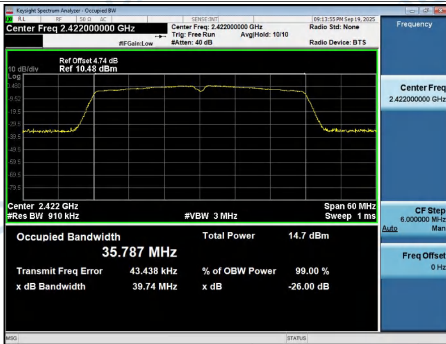
99%_Occupied_Bandwidth_NVNT_ANT2_802_11n(HT40)_2422
