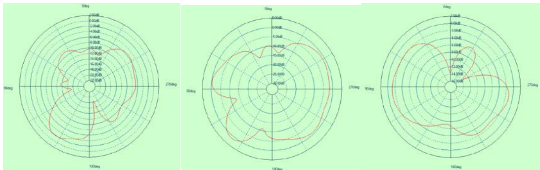
2550MHz_2.5dBi (Phi0/Phi90/Theta90)
