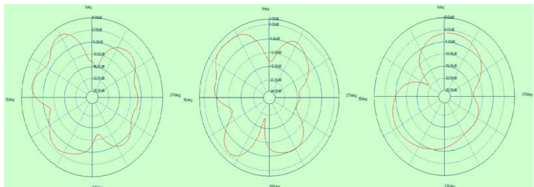
1730MHz_ 2.2dBi (Phi0/Phi90/Theta90)
