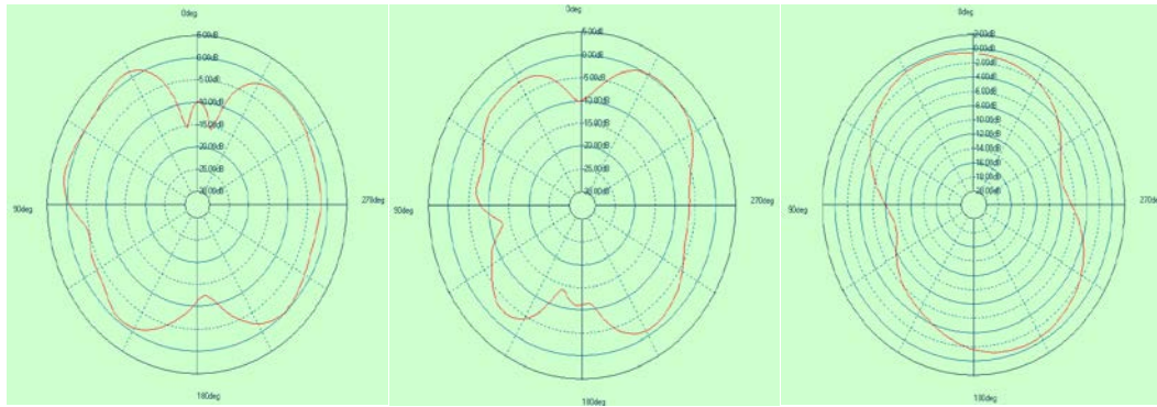
2550MHz_2.5dBi (Phi0/Phi90/Theta90)
