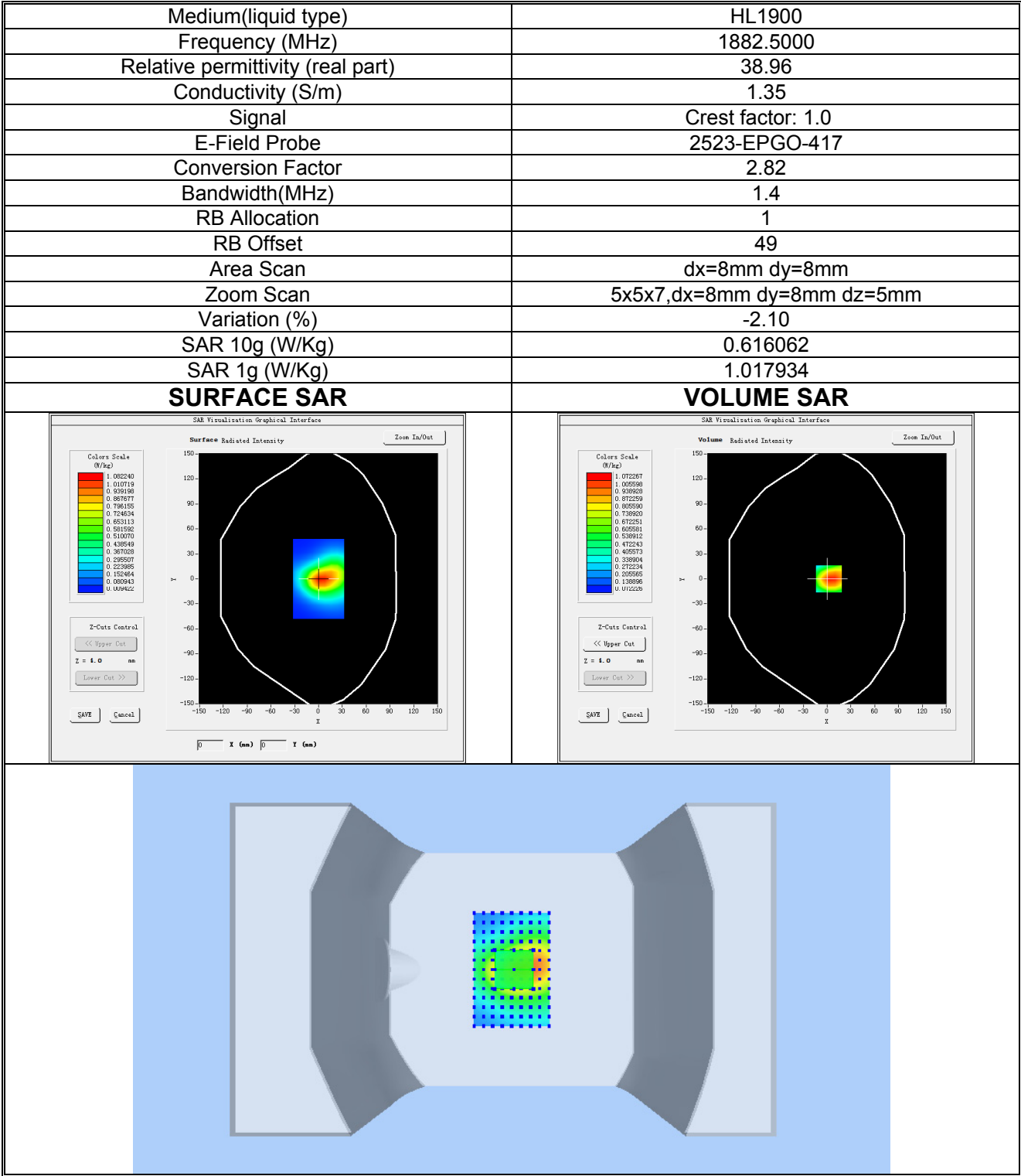
Plot 10: LTE BAND 25, Middle channel (Body-worn, Right Edge) Product Description: ONE Test Date: 2025-10-28
