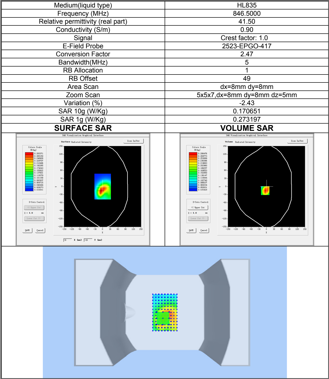
Plot 4: LTE BAND 5, High channel (Body-worn, Front Side) Product Description: ONE Test Date: 2025-10-23
