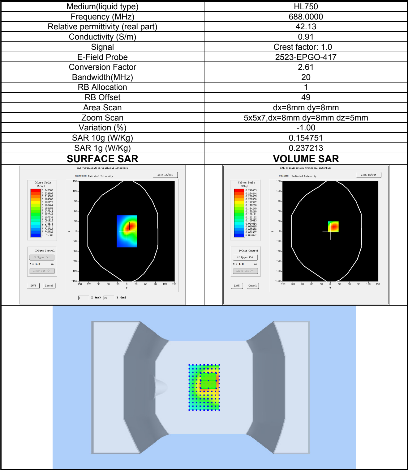
Plot 15: LTE BAND 71, High channel (Body-worn, Front Side) Product Description: ONE Test Date: 2025-10-24
