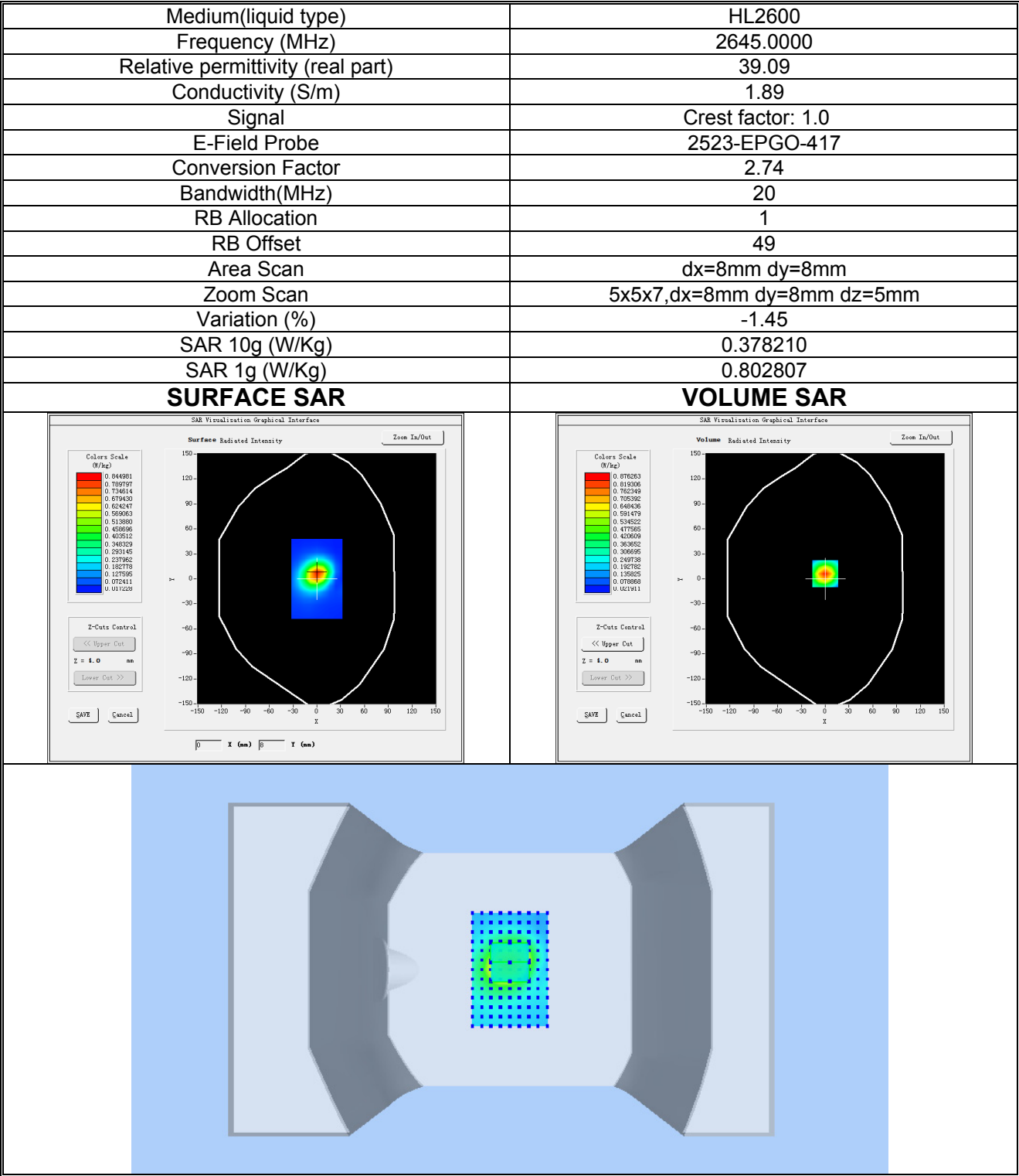
Plot 13: LTE BAND 41, High channel (Body-worn, Right Edge) Product Description: ONE Test Date: 2025-10-20
