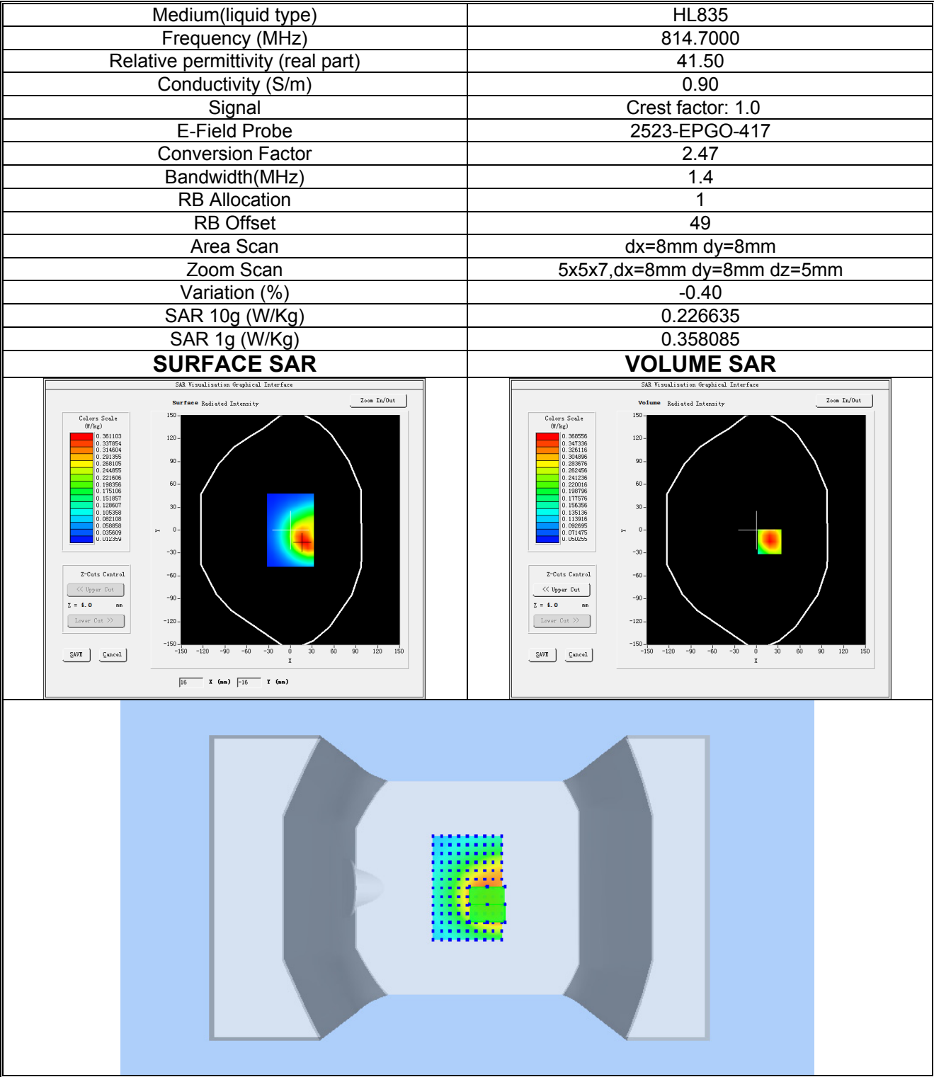
Plot 11: LTE BAND 26(Part 90), Low channel (Body-worn, Front Side) Product Description: ONE Test Date: 2025-10-23
