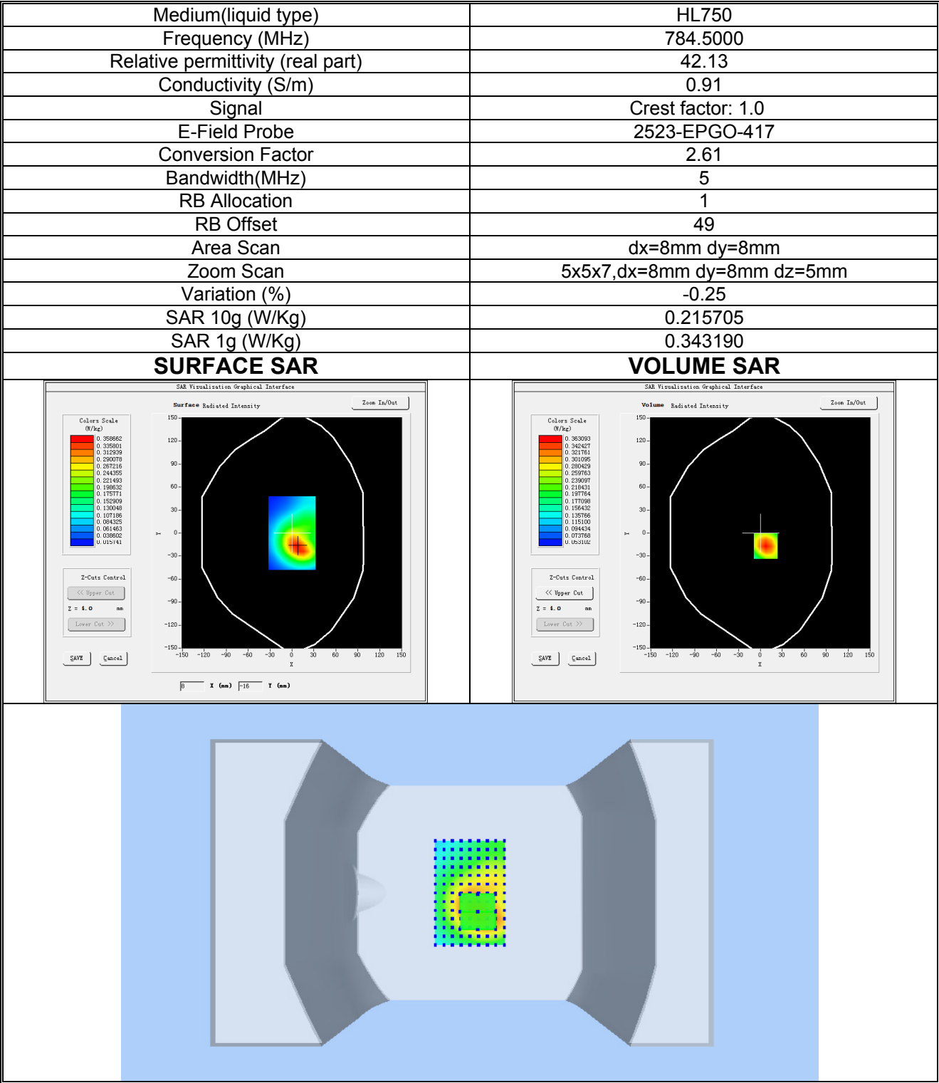
Plot 7: LTE BAND 13, High channel (Body-worn, Front Side) Product Description: ONE Test Date: 2025-10-24
