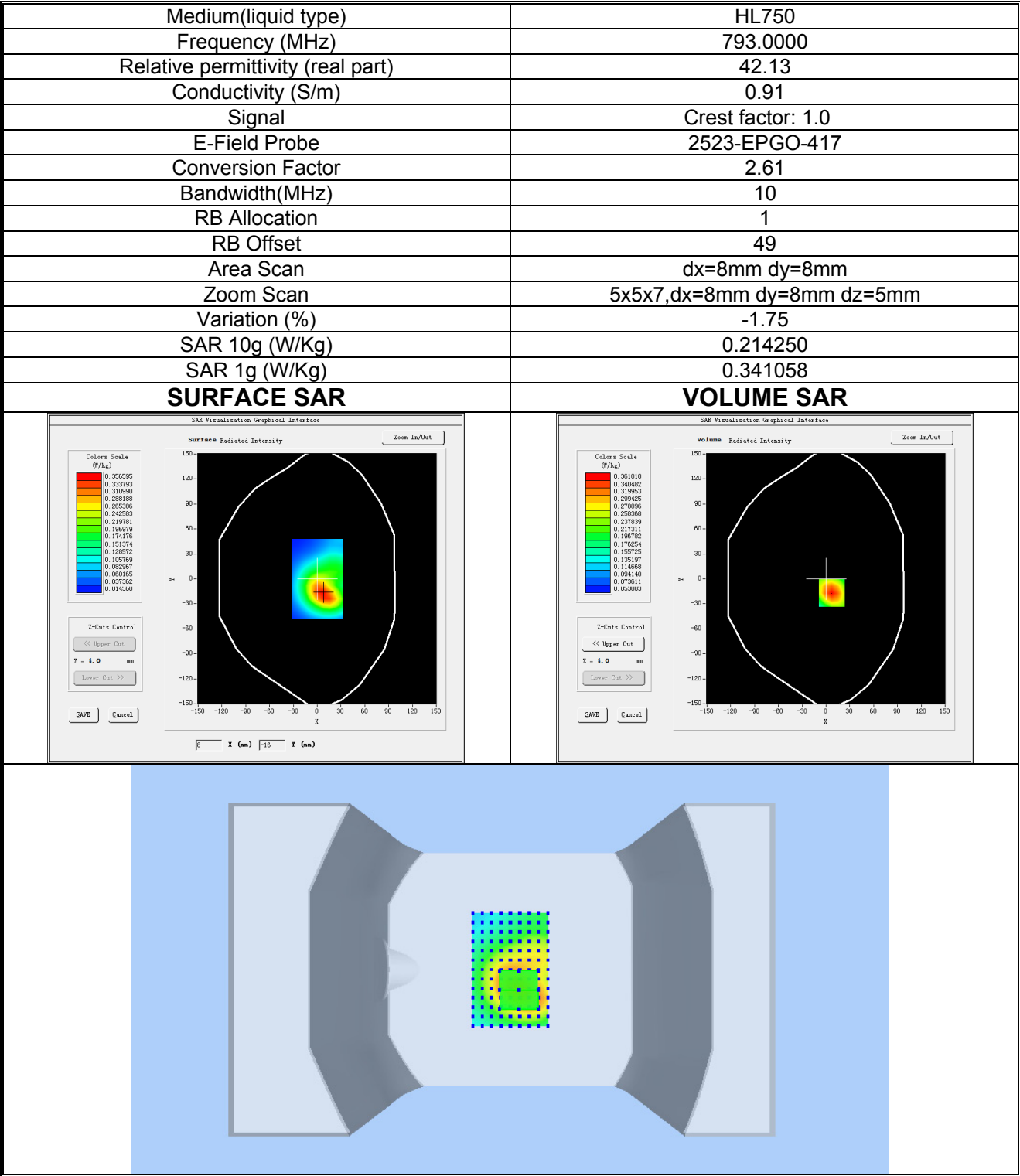
Plot 8: LTE BAND 14, Low channel (Body-worn, Front Side) Product Description: ONE Test Date: 2025-10-24
