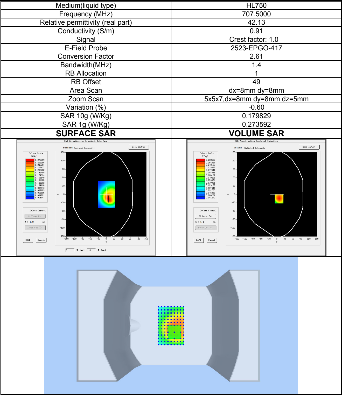
Plot 6: LTE BAND 12, Middle channel (Body-worn, Front Side) Product Description: ONE Test Date: 2025-10-24
