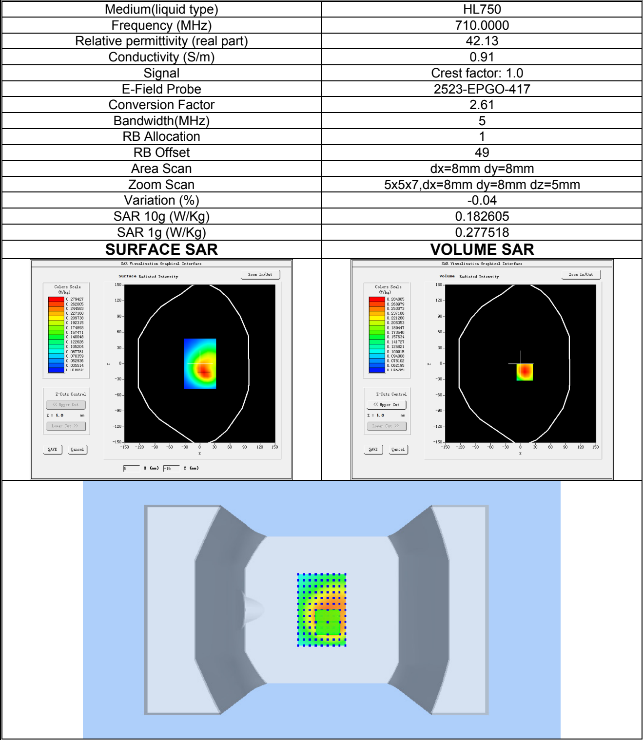
Plot 9: LTE BAND 17, Middle channel (Body-worn, Front Side) Product Description: ONE Test Date: 2025-10-24
