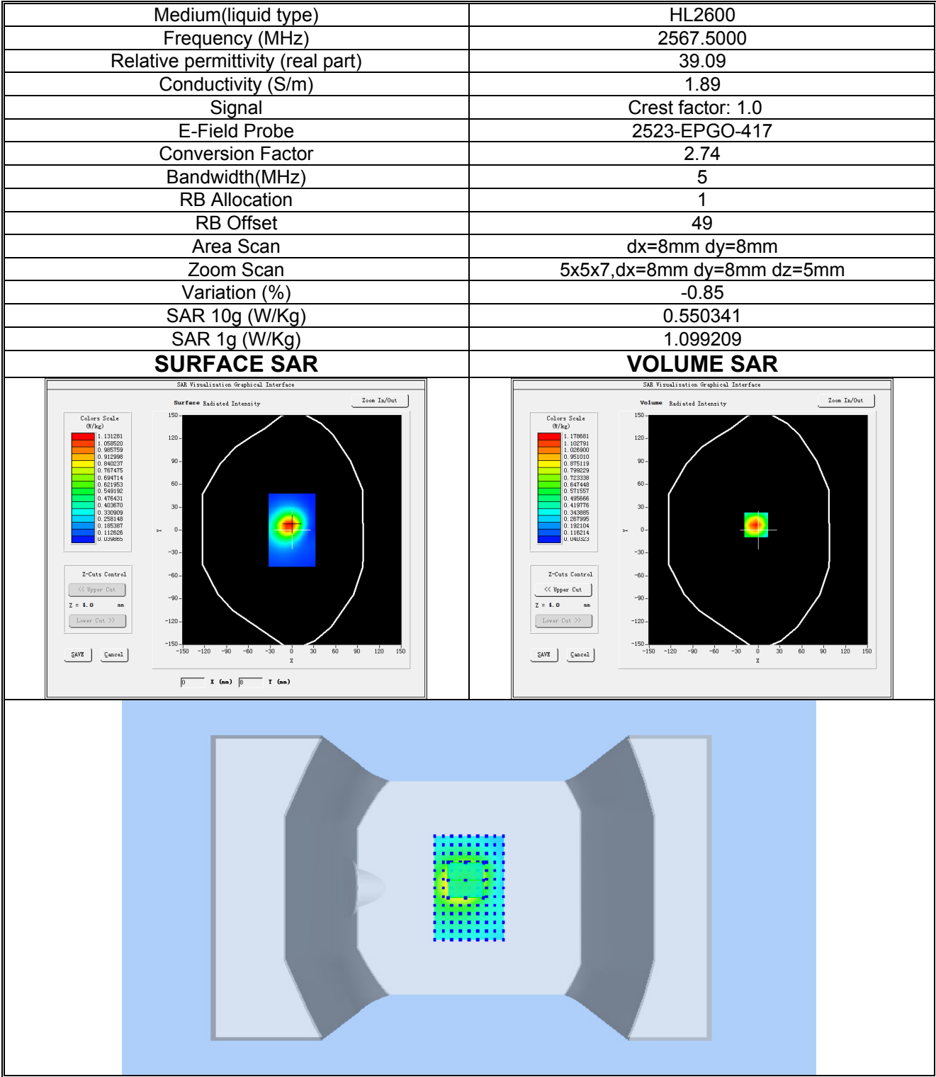
Plot 5: LTE BAND 7, High channel (Body-worn, Right Edge) Product Description: ONE Test Date: 2025-10-20
