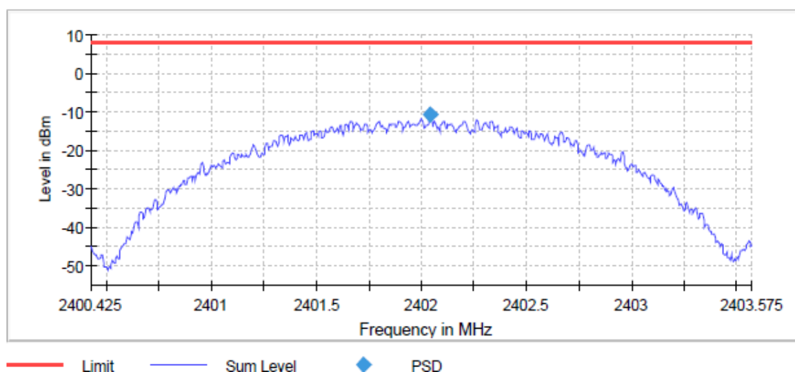
Peak Power Spectral Density
