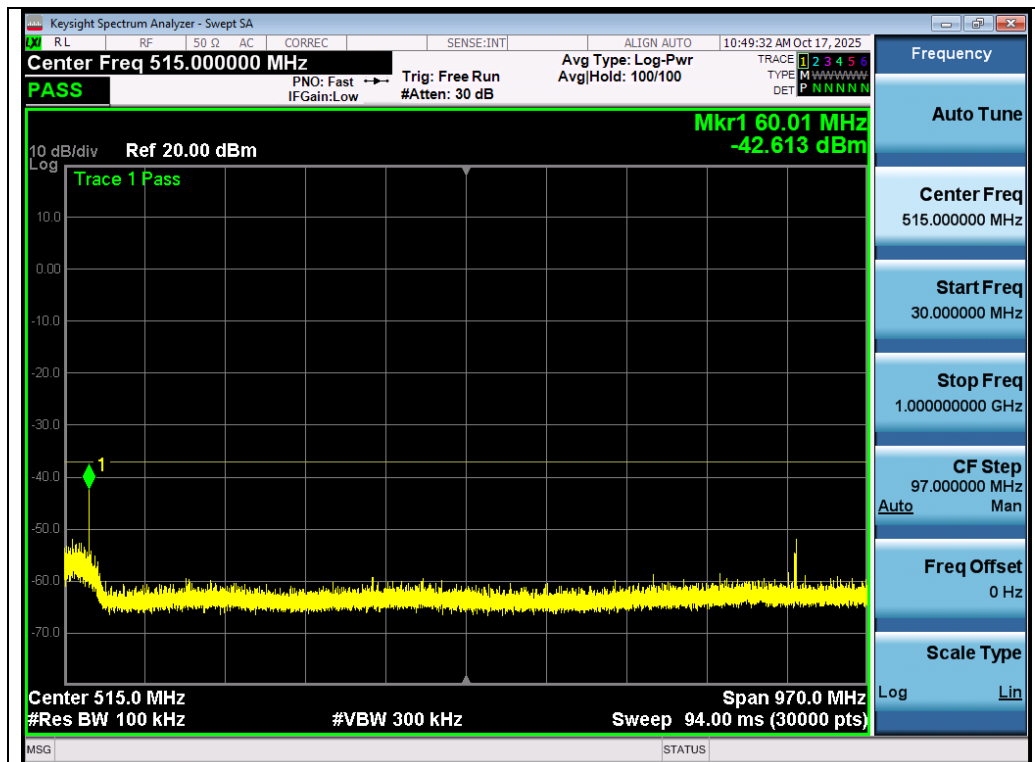
Test_Graph_802.11ac80_ANT2_5610_MCS0_Frequency Band 1
