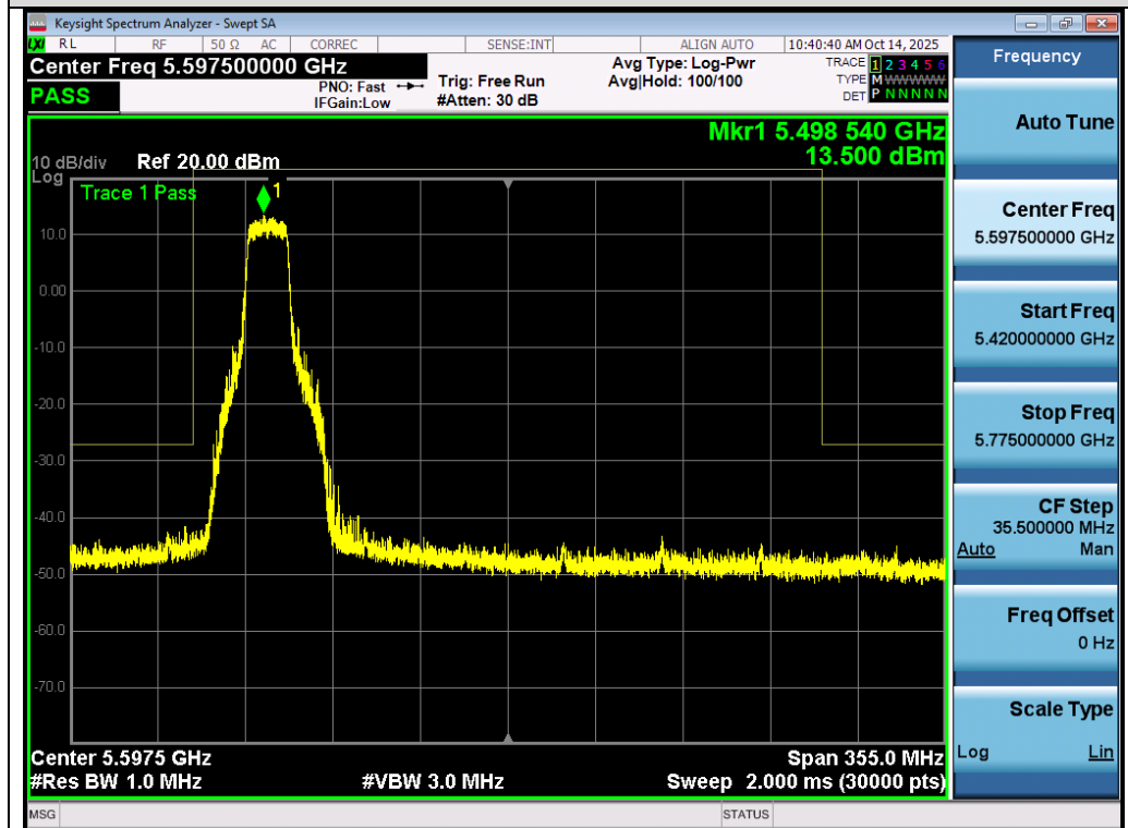
Test_Graph_802.11a_ANT3_5500_6Mbps_Frequency Band 3
