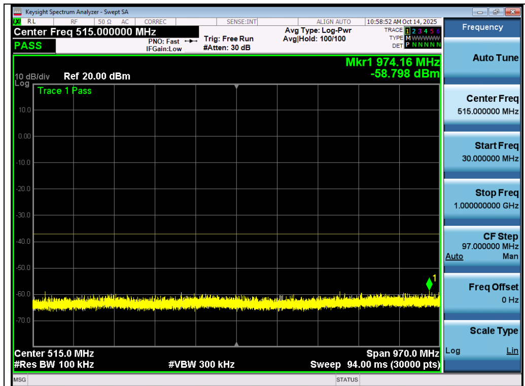
Test_Graph_802.11ac80_ANT3_5530_MCS0_Frequency Band 1
