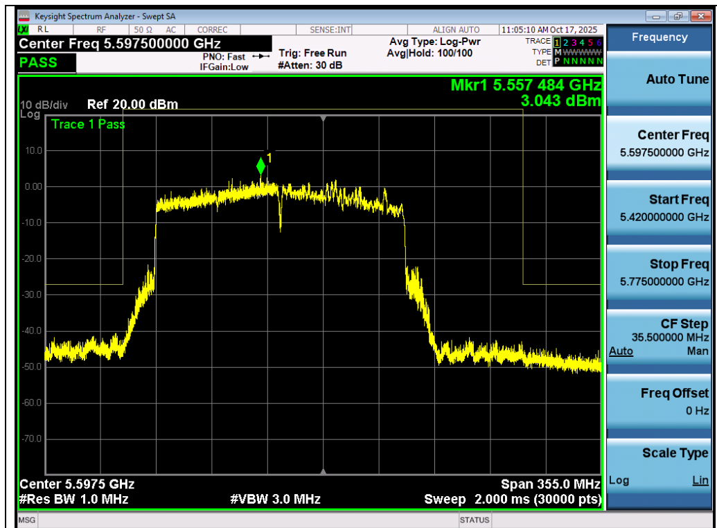
Test_Graph_802.11ax160_ANT 2_5570_MCS0_Frequency Band 3
