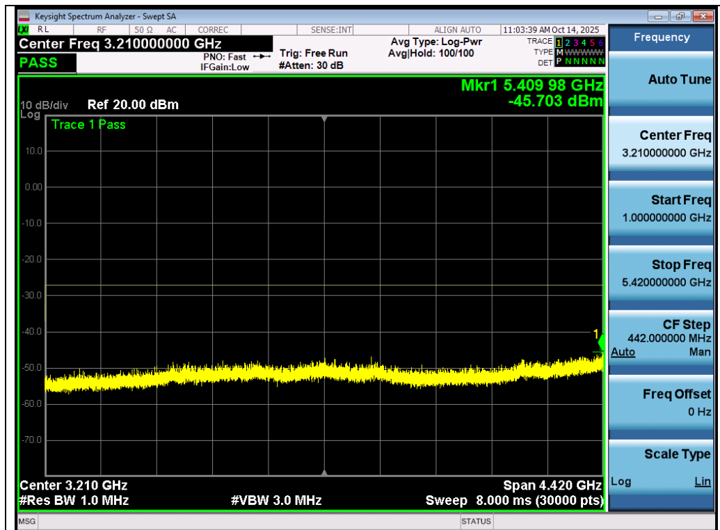
Test_Graph_802.11ac80_ANT3_5610_MCS0_Frequency Band 2
