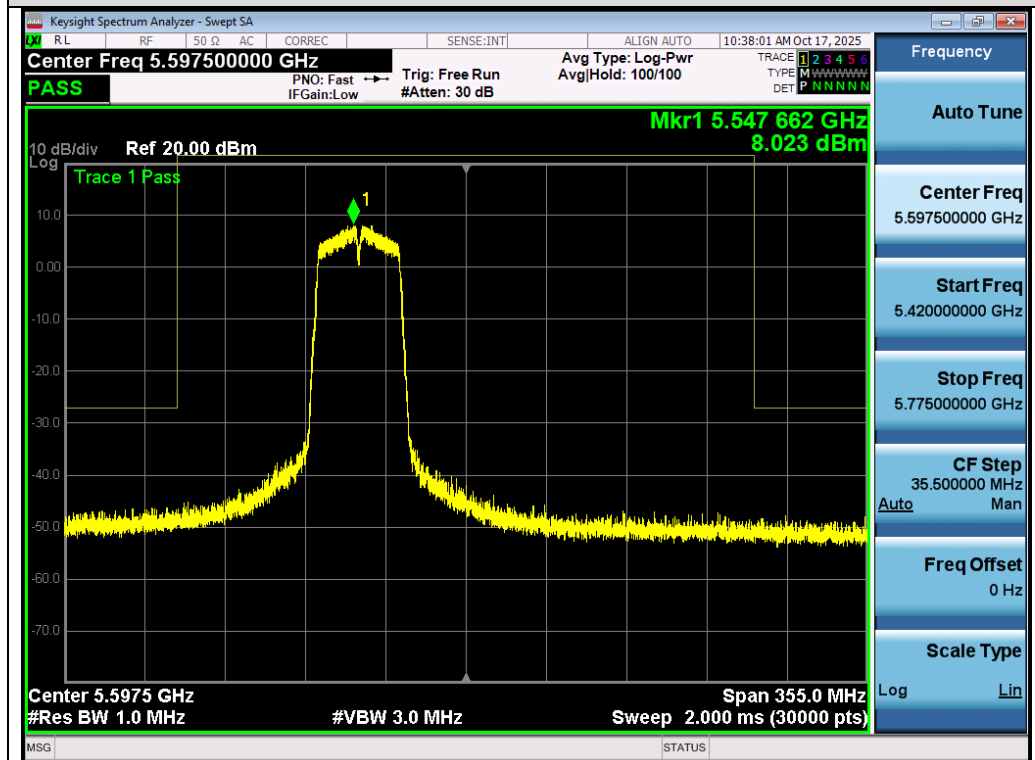
Test_Graph_802.11n40_ANT2_5550_MCS0_Frequency Band 3
