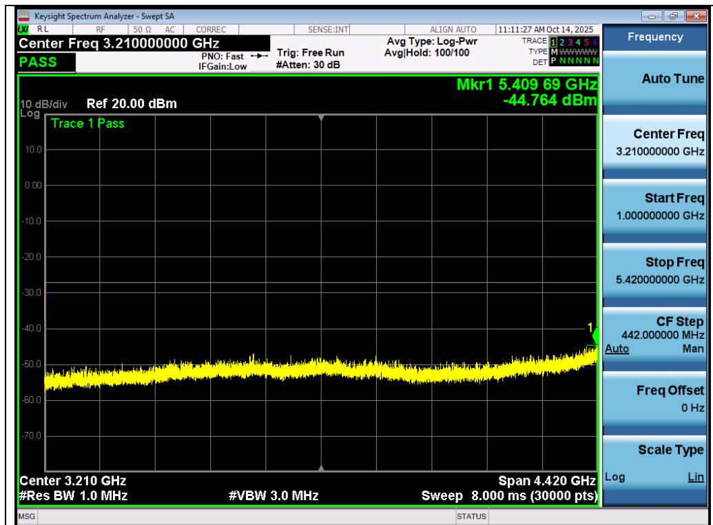
Test_Graph_802.11ax80_ANT3_5530_MCS0_Frequency Band 2
