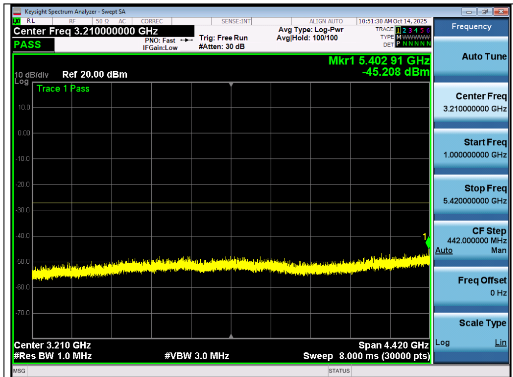
Test_Graph_802.11n40_ANT3_5670_MCS0_Frequency Band 2
