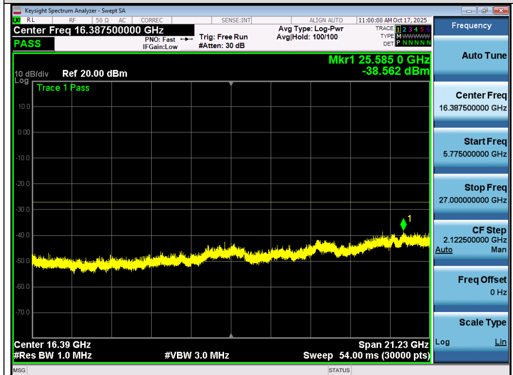
Test_Graph_802.11ax80_ANT2_5530_MCS0_Frequency Band 4
