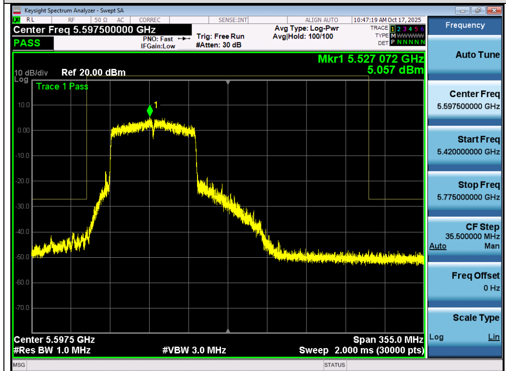
Test_Graph_802.11ac80_ANT2_5530_MCS0_Frequency Band 3
