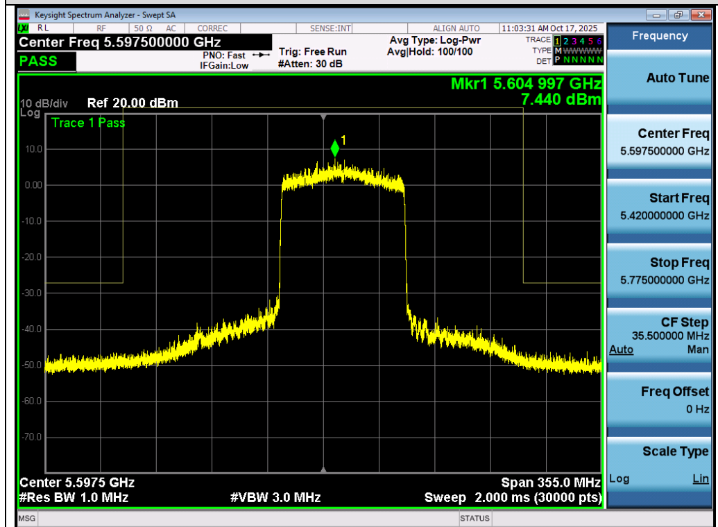
Test_Graph_802.11ax80_ANT2_5610_MCS0_Frequency Band 3
