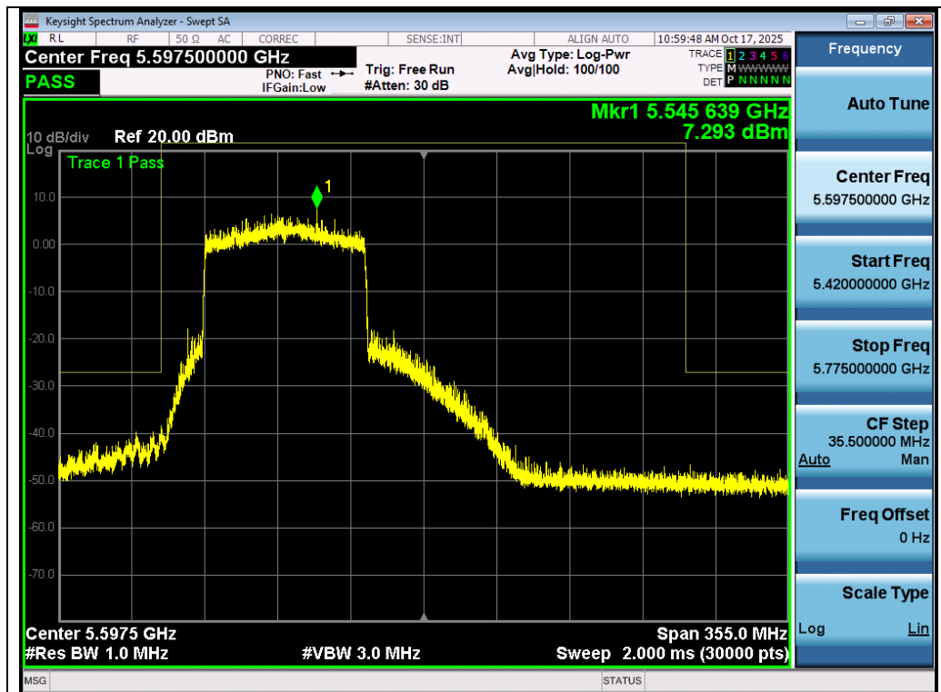
Test_Graph_802.11ax80_ANT2_5530_MCS0_Frequency Band 3
