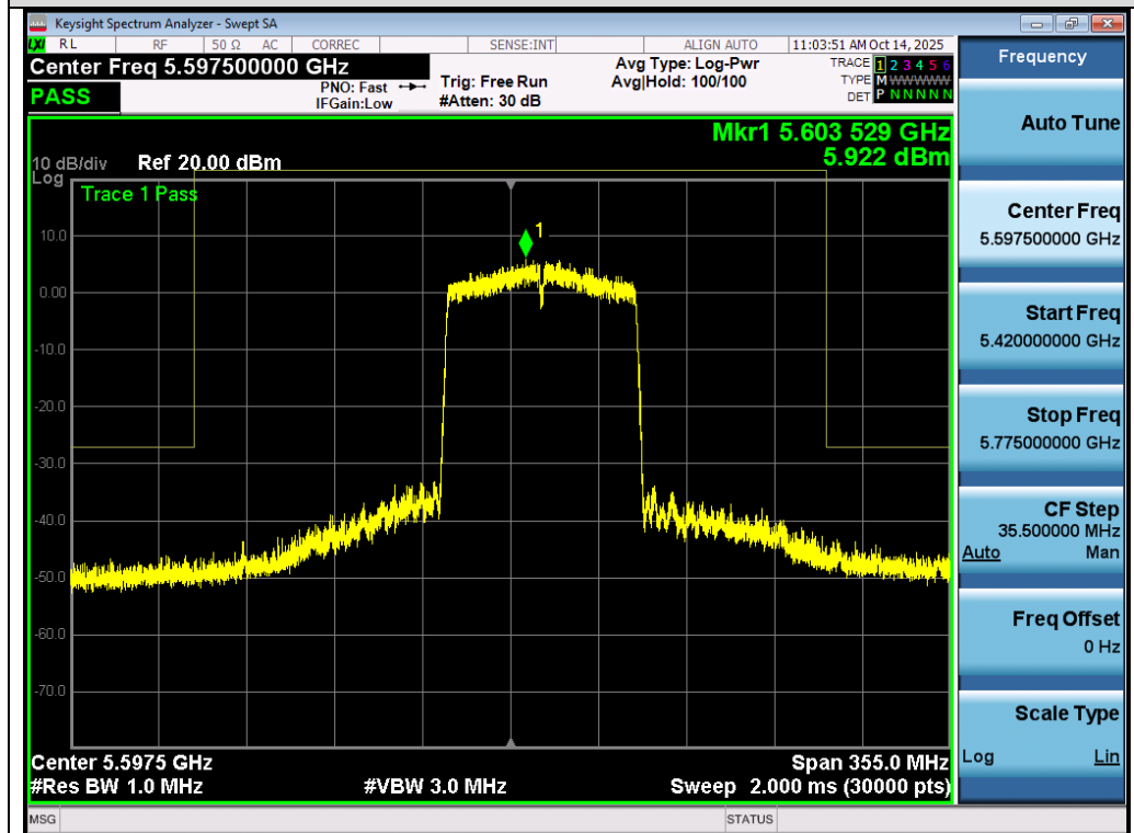
Test_Graph_802.11ac80_ANT3_5610_MCS0_Frequency Band 3
