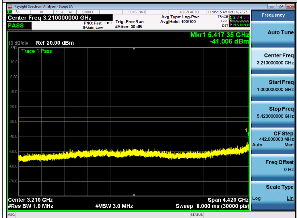
Test_Graph_802.11ac160_ANT 3_5570_MCS0_Frequency Band 2
