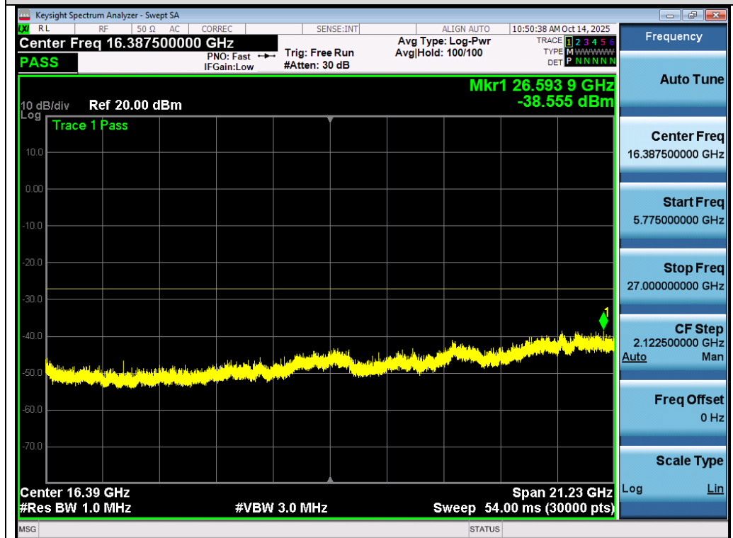
Test_Graph_802.11n40_ANT3_5550_MCS0_Frequency Band 4
