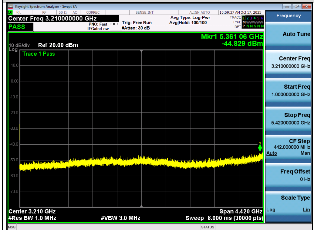
Test_Graph_802.11ax80_ANT2_5530_MCS0_Frequency Band 2
