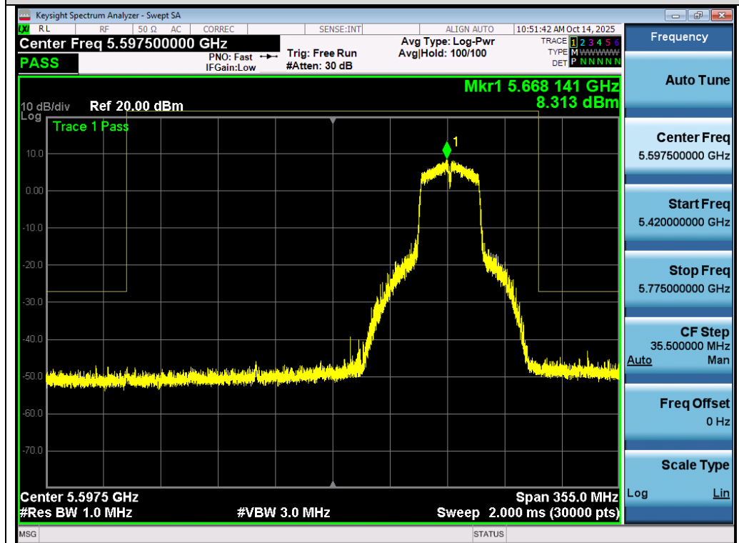
Test_Graph_802.11n40_ANT3_5670_MCS0_Frequency Band 3
