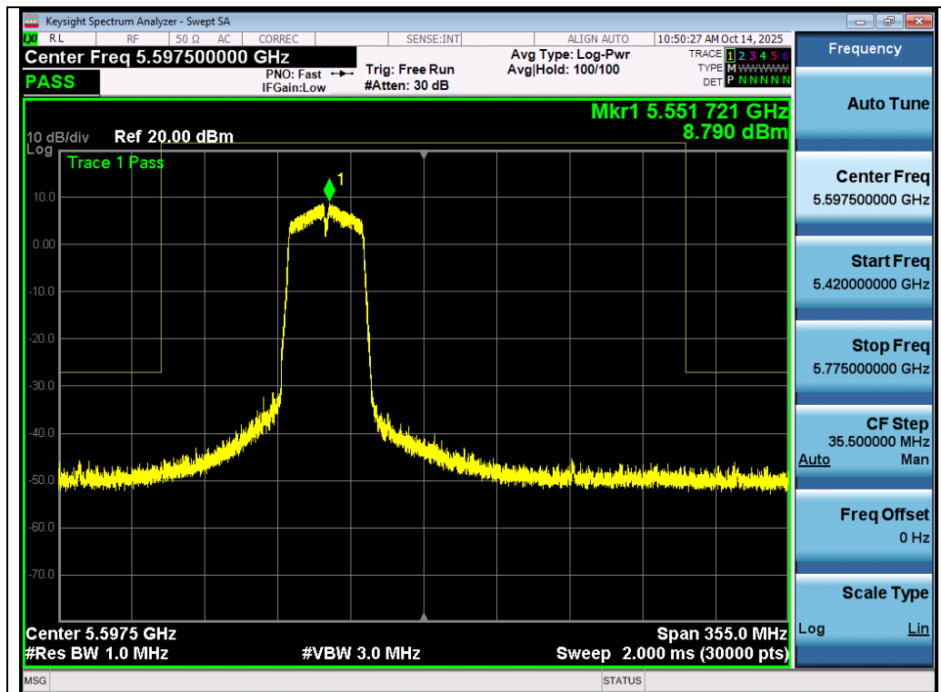
Test_Graph_802.11n40_ANT3_5550_MCS0_Frequency Band 3
