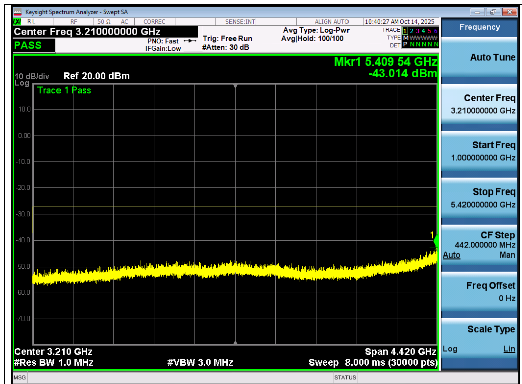
Test_Graph_802.11a_ANT3_5500_6Mbps_Frequency Band 2
