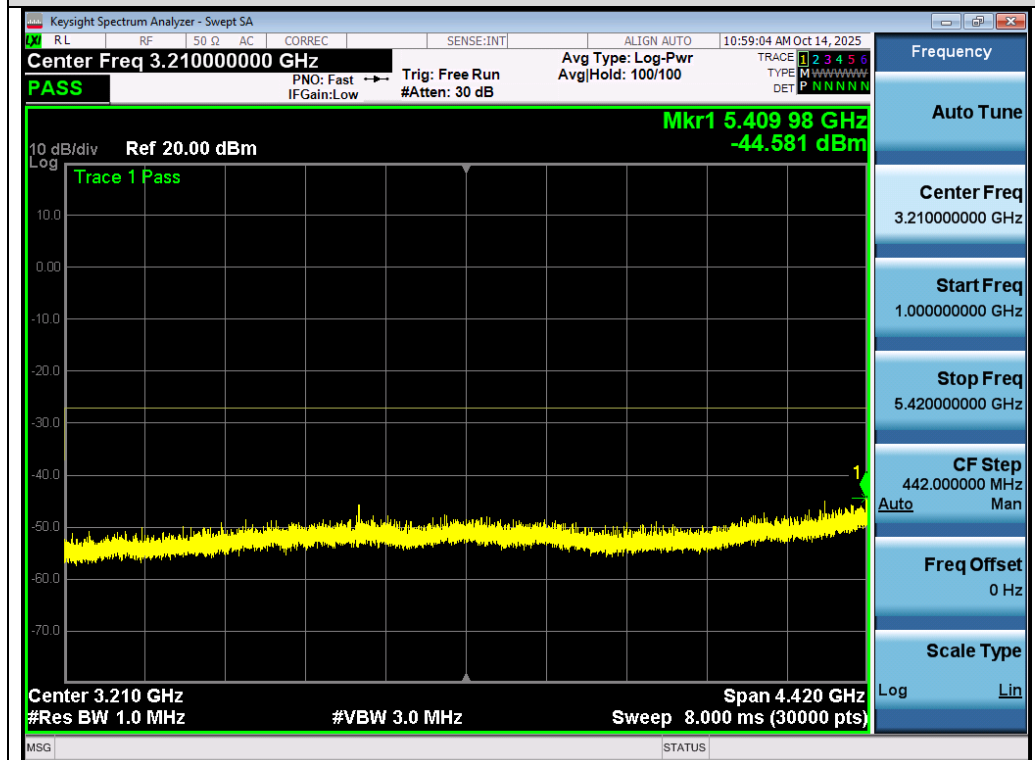
Test_Graph_802.11ac80_ANT3_5530_MCS0_Frequency Band 2
