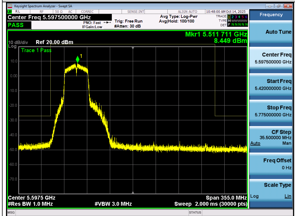
Test_Graph_802.11n40_ANT3_5510_MCS0_Frequency Band 3
