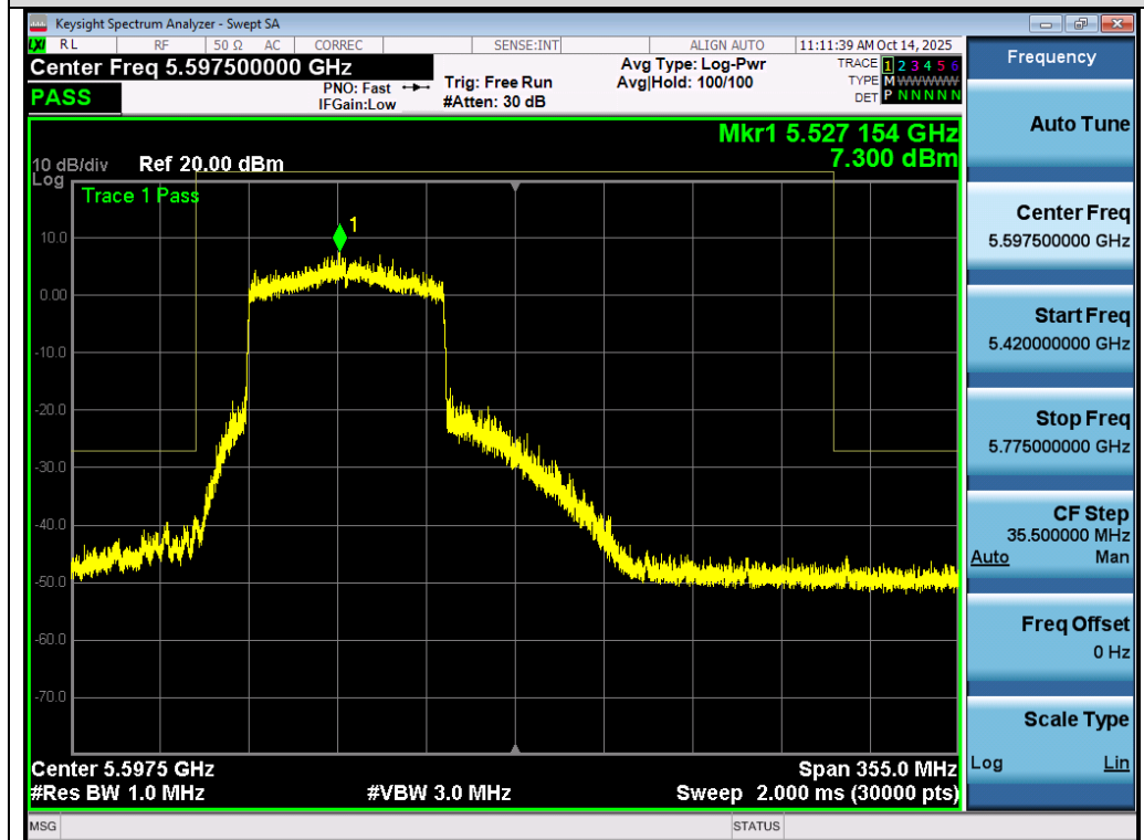
Test_Graph_802.11ax80_ANT3_5530_MCS0_Frequency Band 3
