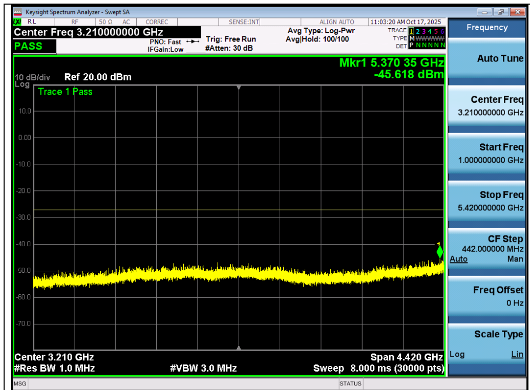
Test_Graph_802.11ax80_ANT2_5610_MCS0_Frequency Band 2
