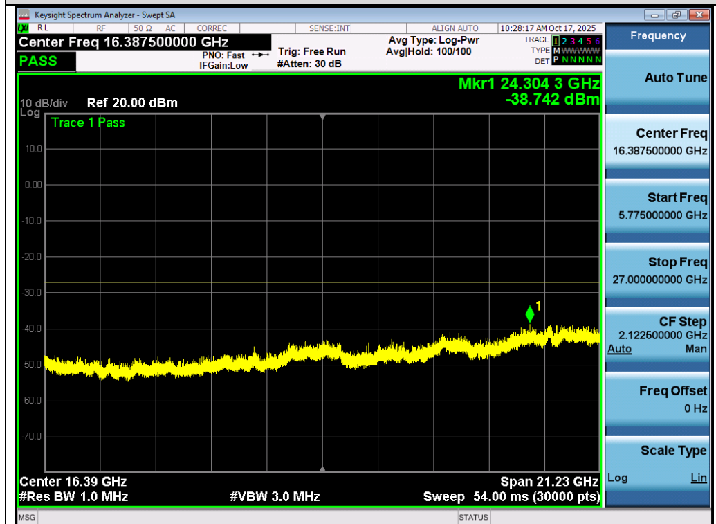
Test_Graph_802.11a_ANT2_5500_6Mbps_Frequency Band 4
