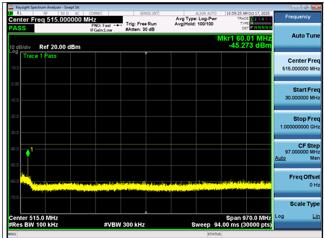
Test_Graph_802.11ax80_ANT2_5530_MCS0_Frequency Band 1
