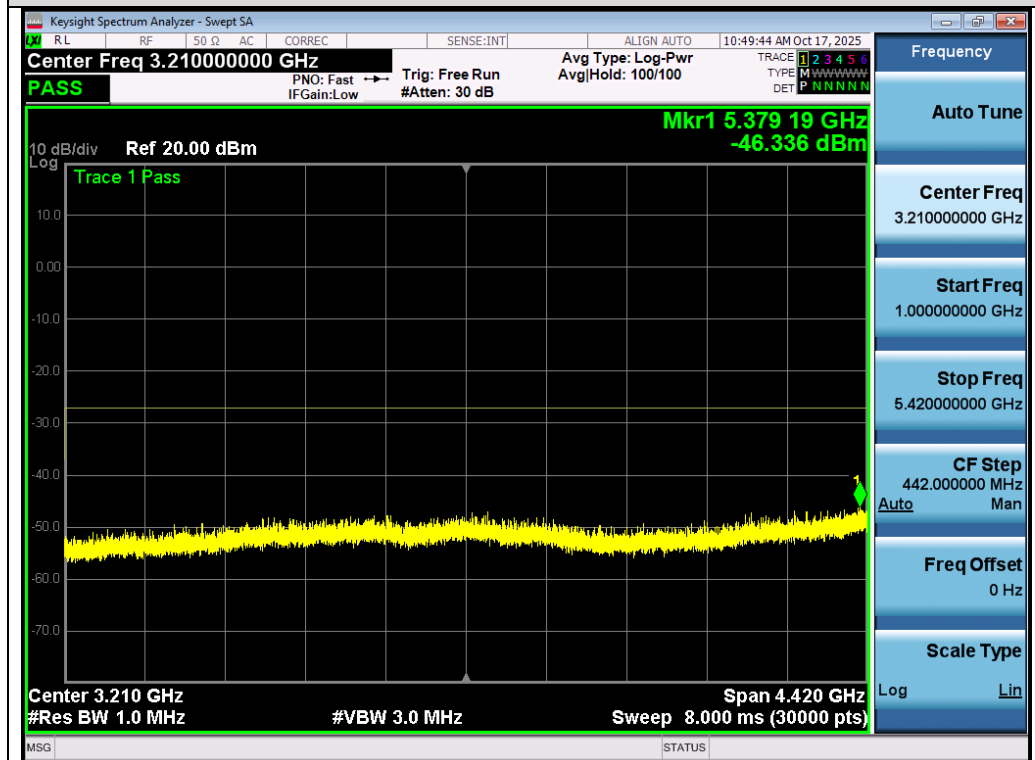
Test_Graph_802.11ac80_ANT2_5610_MCS0_Frequency Band 2
