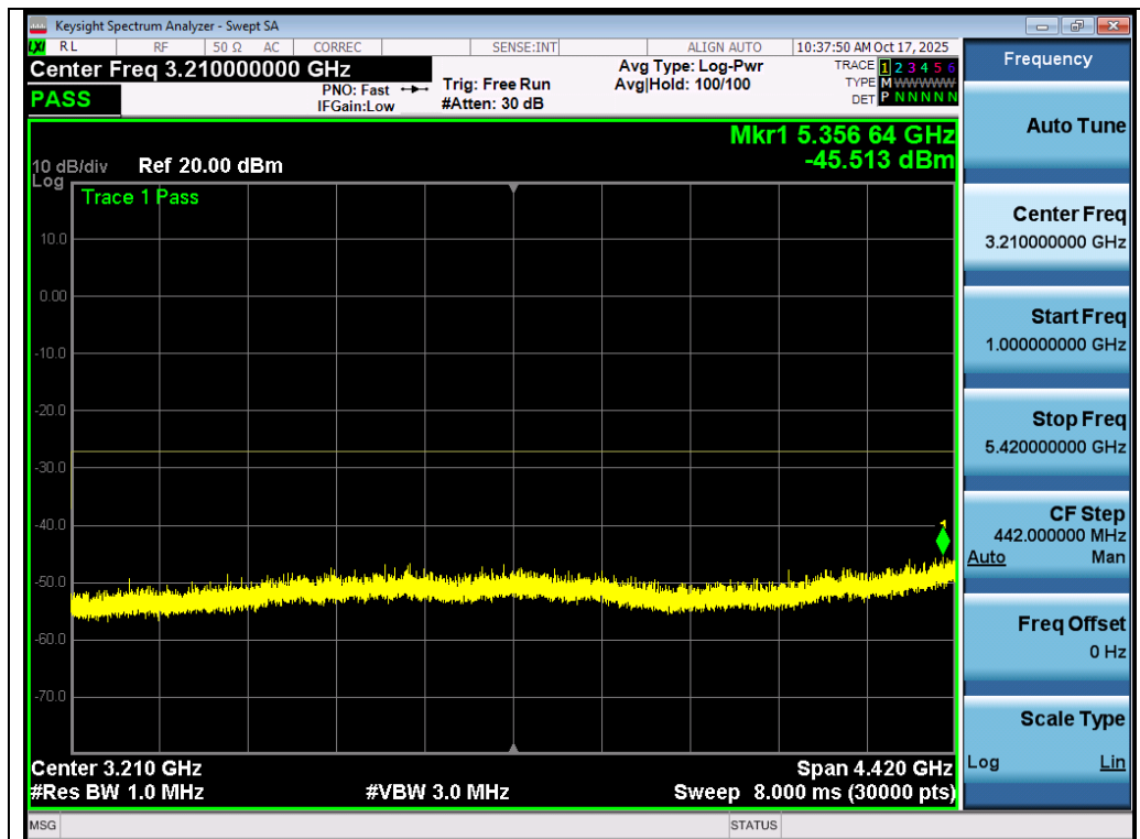
Test_Graph_802.11n40_ANT2_5550_MCS0_Frequency Band 2
