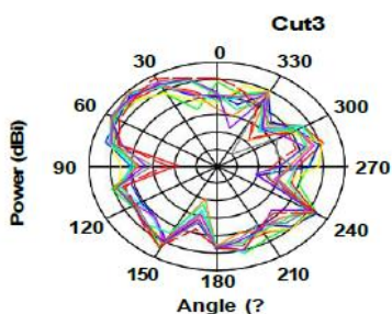
Horizontally Polarized YZ plane
