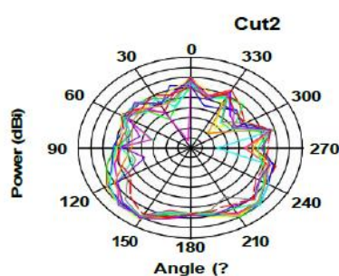
Horizontally Polarized XZ plane
