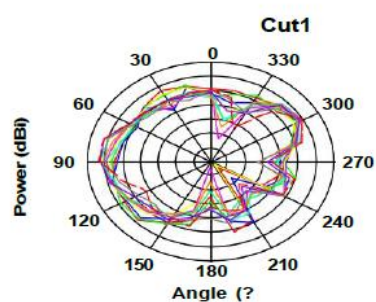
Vertical Polarization XY plane
