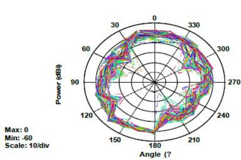
Vertical Polarization XZ plane
