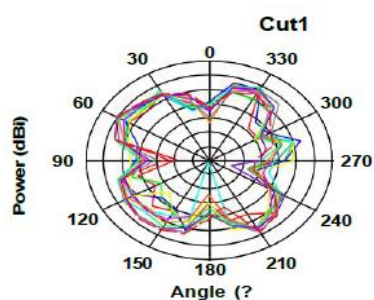
Horizontally Polarized XY plane
