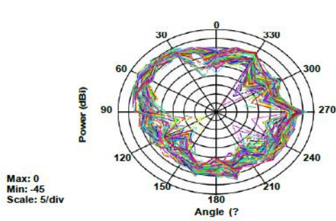
Vertical Polarization XY plane
