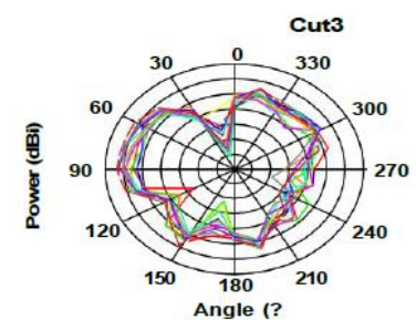
Vertical Polarization YZ plane
