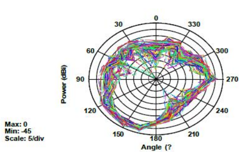
Vertical Polarization YZ plane
