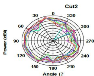
Vertical Polarization XZ plane
