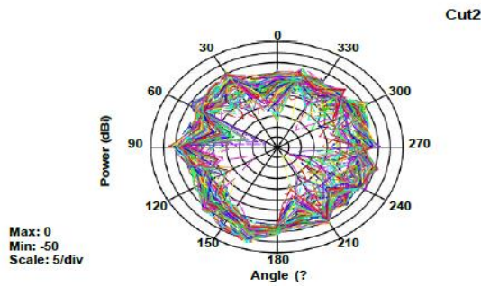
Horizontally Polarized XZ plane
