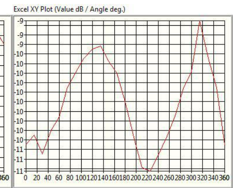
2.45GHz@Theta 0.0 Total
