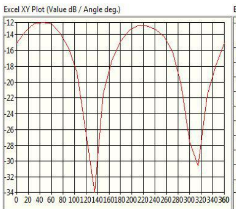
2.485GHz@Theta 0.0 Horizontal
