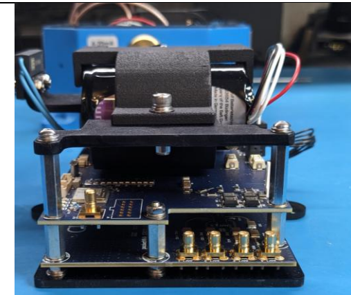
Electronics stack and battery side 4
