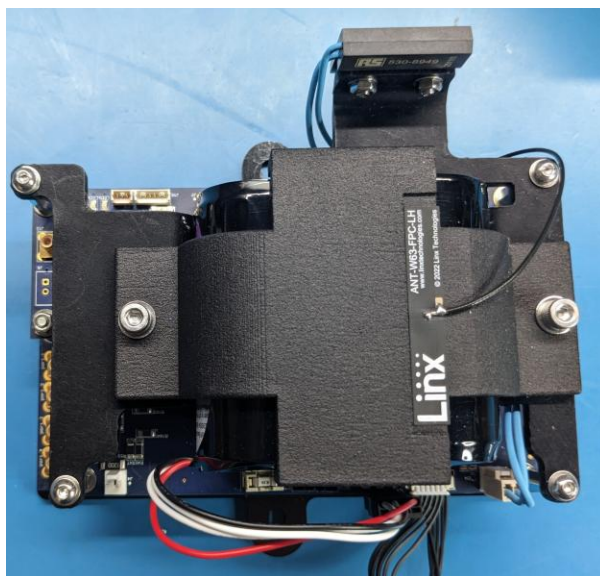
Electronics stack and battery top view
