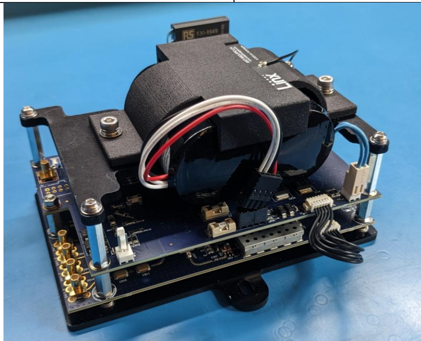
Electronics stack and battery view
