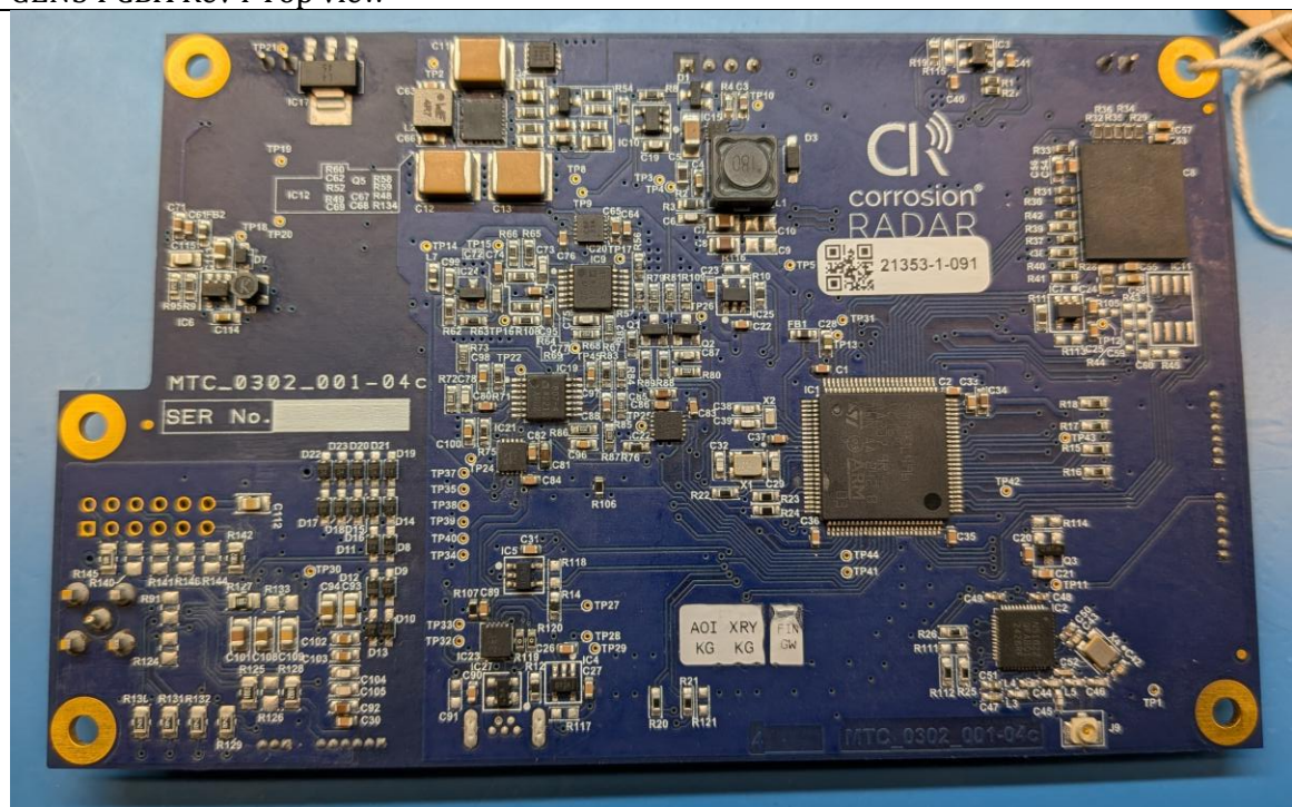
GEN3 PCBA Rev4 Bottom view
