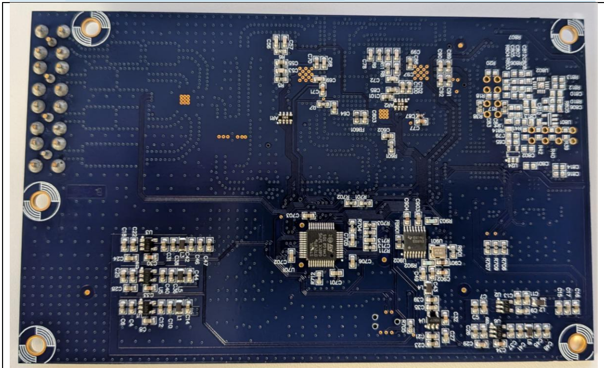
PVNA PCBA Rev3.4.0.12 Bottom view
