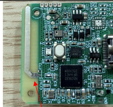
PCB Antenna
