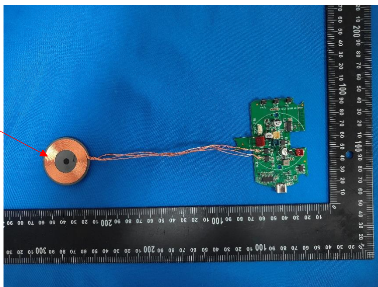
Loop Antenna
