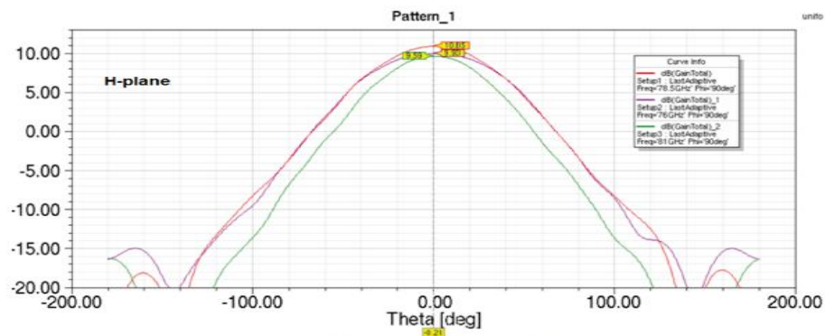
Figure 11. Antenna Pattern in H-Plane
