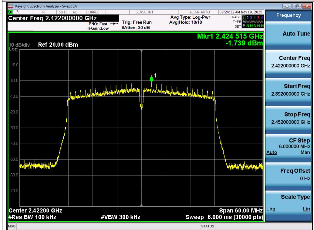
Test_Graph_802.11n40_Chain A_2422_MCS0_Reference Level
