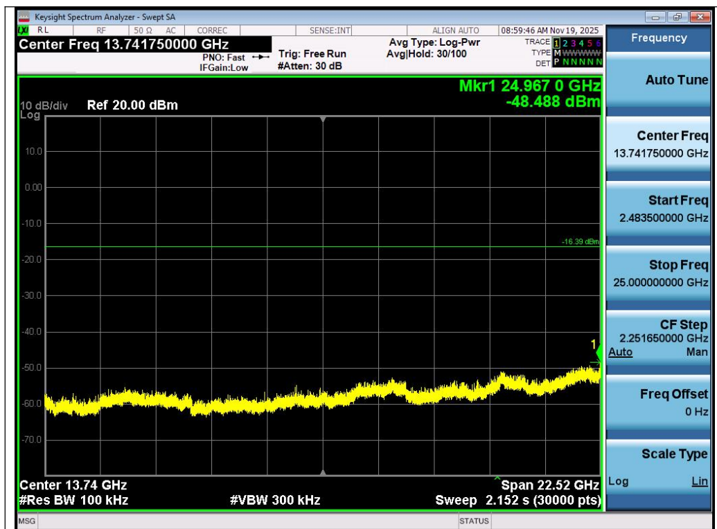
Test_Graph_802.11b_Chain A_2412_1Mbps_Higher Band Emissions
