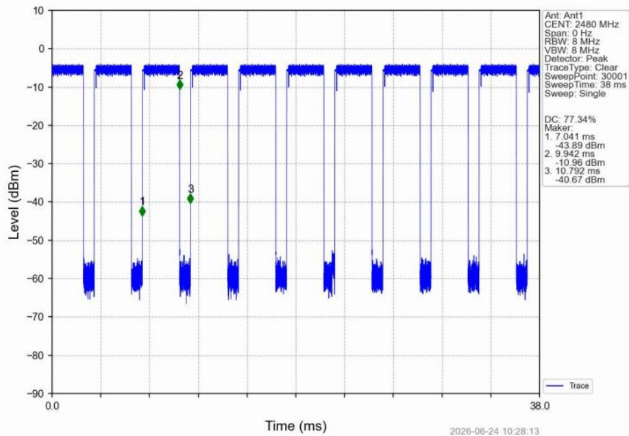
8DPSK_3DH5_HCH_2480MHz_Left_NTNV
