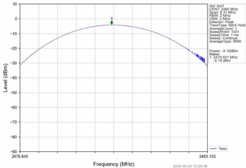
8DPSK_3DH5_HCH_2480MHz_Left_NTNV
