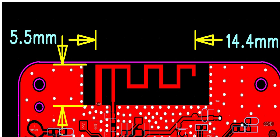
Antenna photo&Length(mm)
