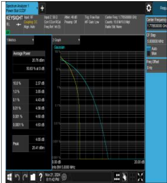
Band66-3MHz-QPSK-132657-1RB#0-PASS
