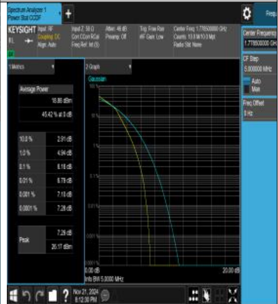
Band66-3MHz-16QAM-132657-15RB#0-PASS
