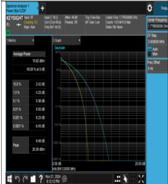
Band66-3MHz-QPSK-132657-15RB#0-PASS
