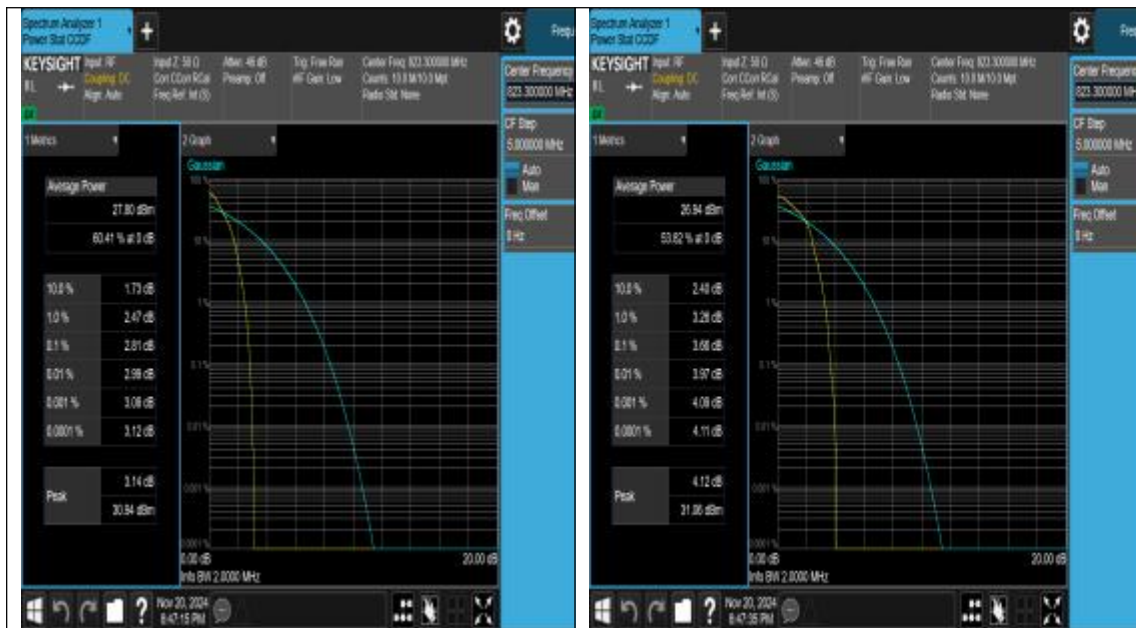
26(814-824)-1.4MHz-QPSK-26783-1RB#0-PASS
