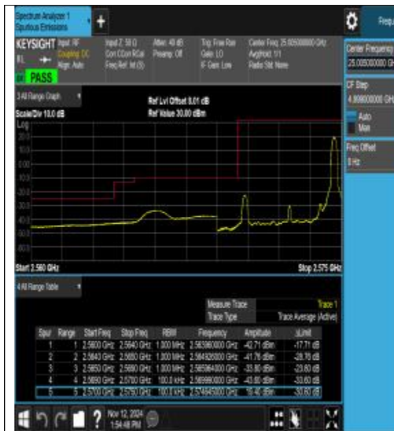
Band38_5MHz_QPSK_37775_1RB#24
