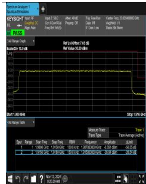
Band25_15MHz_QPSK_26615_75RB#0
