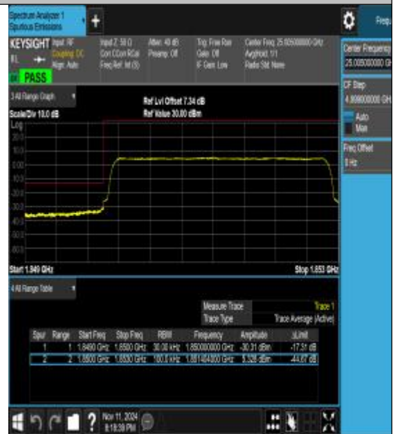
Band25_3MHz_16QAM_26055_15RB#0
