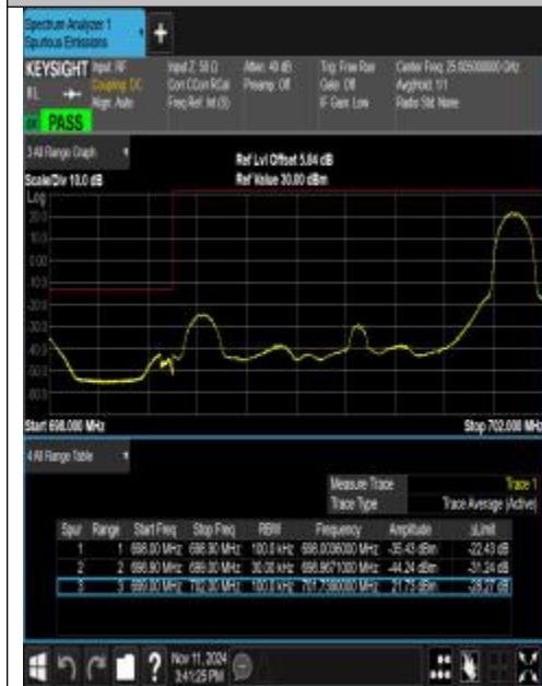
Band12_3MHz_QPSK_23025_1RB#14
