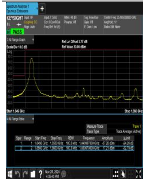
Band25_10MHz_QPSK_26090_1RB#0
