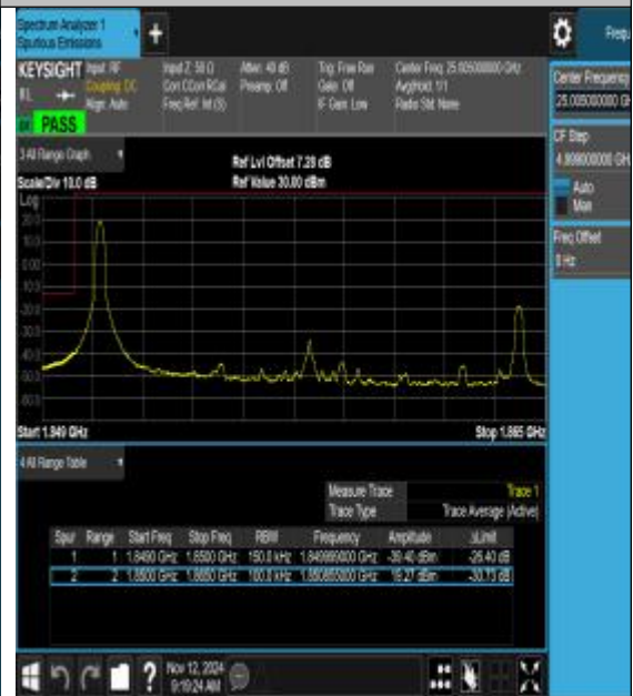
Band25_15MHz_16QAM_26115_1RB#0
