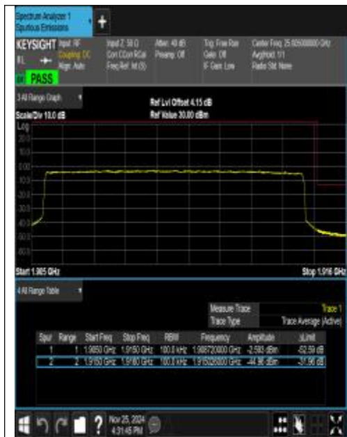
Band25_10MHz_QPSK_26640_50RB#0
