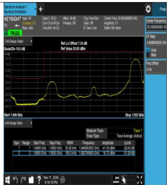
Band25_3MHz_16QAM_26055_1RB#14
