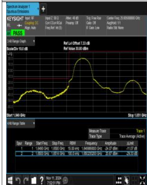
Band25_1.4MHz_QPSK_26047_1RB#0
