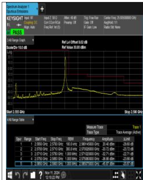
Band7_15MHz_QPSK_21375_1RB#74
