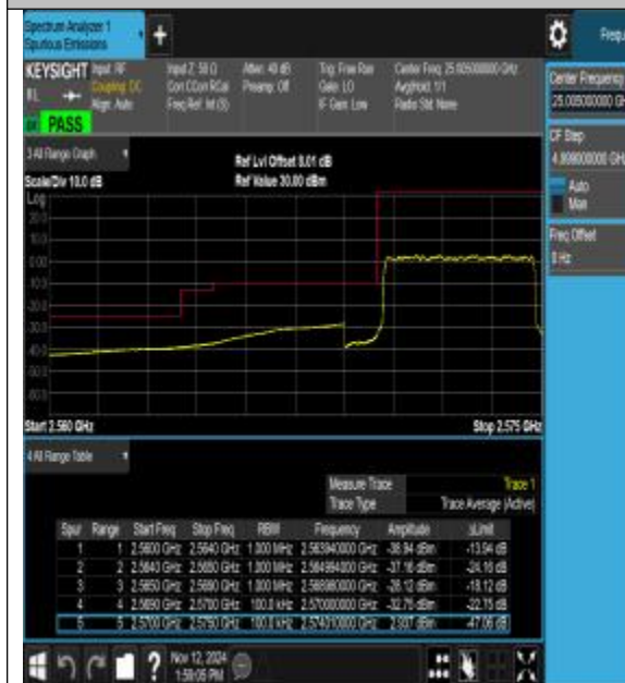
Band38_5MHz_QPSK_37775_25RB#0
