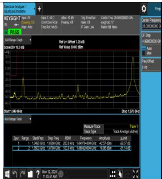
Band25_20MHz_16QAM_26140_1RB#99
