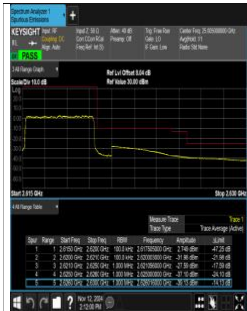
Band38_5MHz_QPSK_38225_25RB#0
