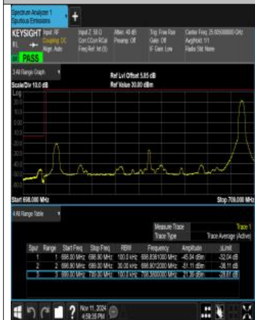
Band12_10MHz_QPSK_23060_1RB#49
