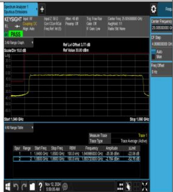
Band25_10MHz_16QAM_26090_50RB#0
