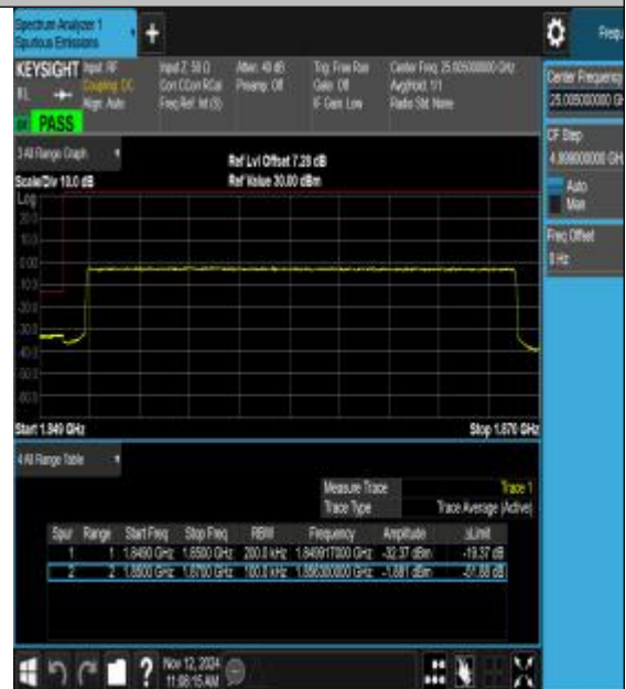
Band25_20MHz_16QAM_26140_100RB#0
