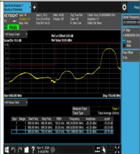
Band12_1.4MHz_16QAM_23017_1RB#5
