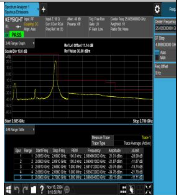
Band41_5MHz_16QAM_41565_1RB#24
