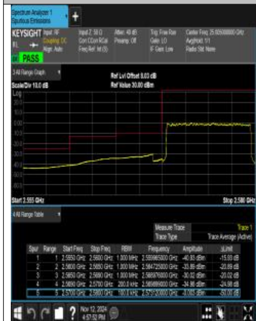
Band38_10MHz_QPSK_37800_1RB#0
