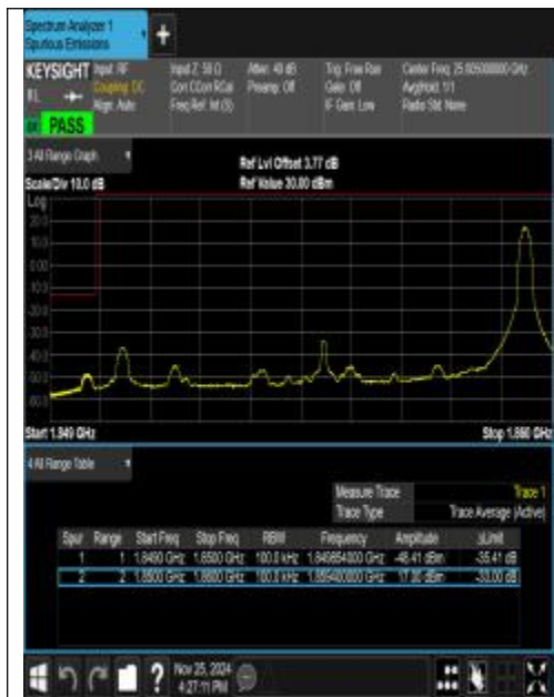
Band25_10MHz_QPSK_26090_1RB#49
