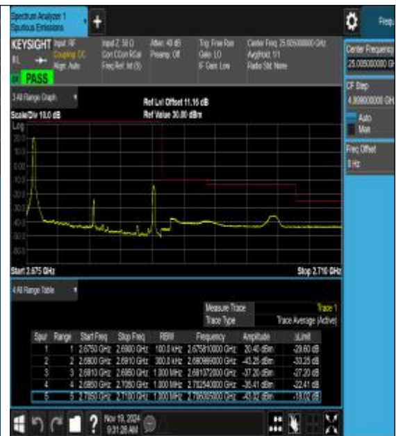
Band41_15MHz_16QAM_41515_1RB#0
