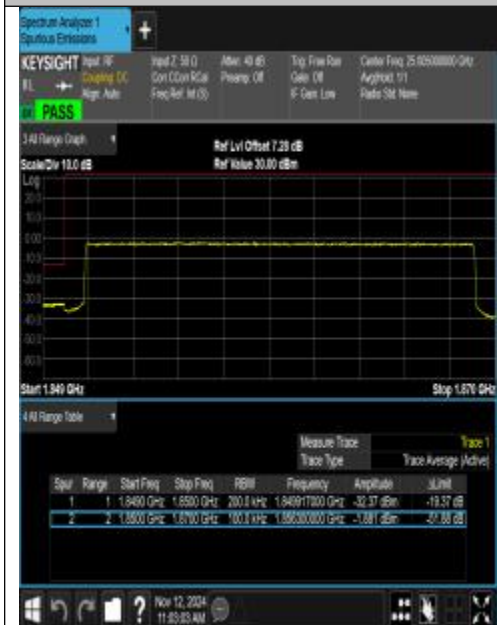
Band25_20MHz_QPSK_26140_100RB#0
