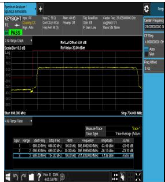
Band12_5MHz_16QAM_23035_25RB#0
