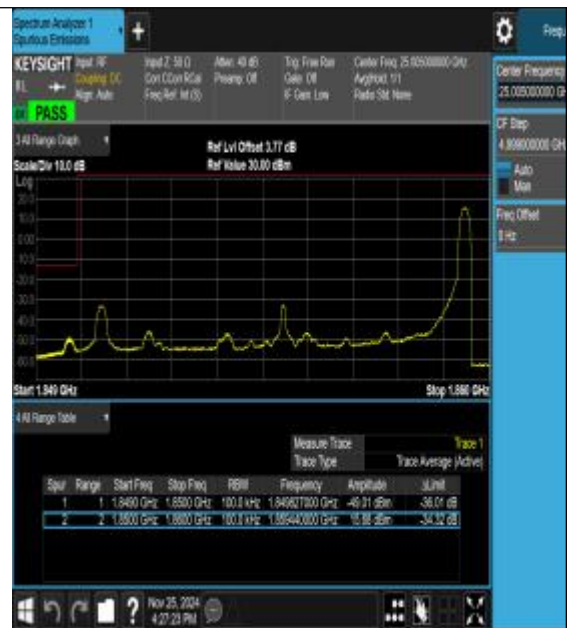
Band25_10MHz_16QAM_26090_1RB#49
