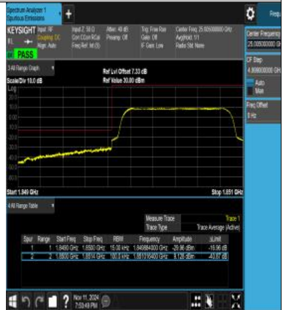
Band25_1.4MHz_16QAM_26047_6RB#0
