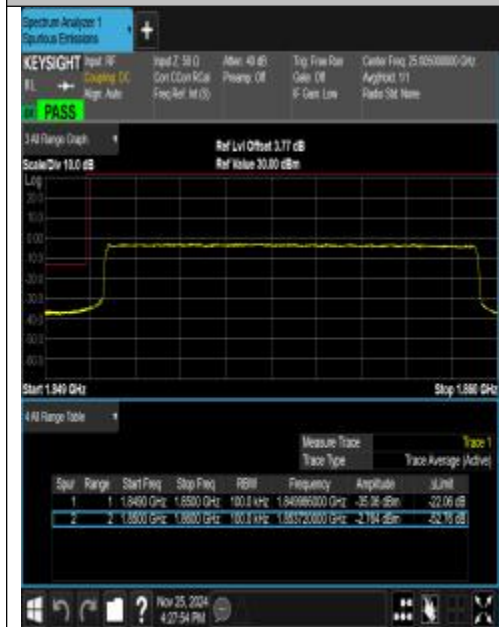
Band25_10MHz_QPSK_26090_50RB#0
