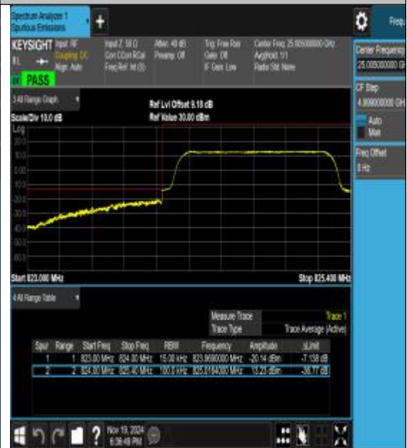
Band26_1.4MHz_16QAM_26797_6RB#0
