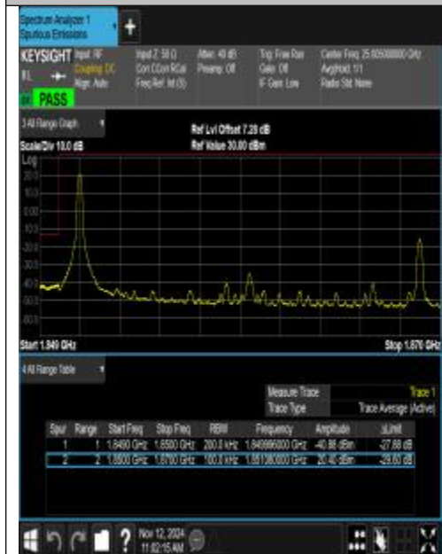
Band25_20MHz_QPSK_26140_1RB#0
