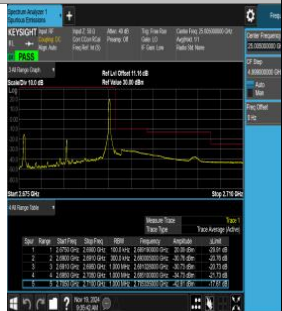
Band41_15MHz_16QAM_41515_1RB#74
