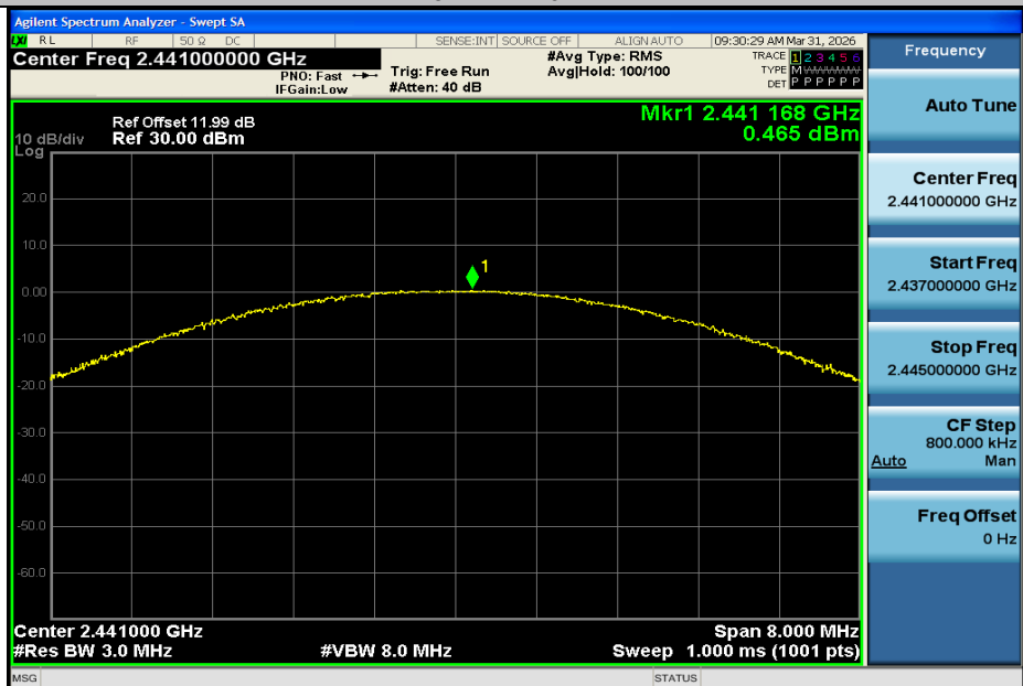
2DH5-Ant1-2441-PASS
