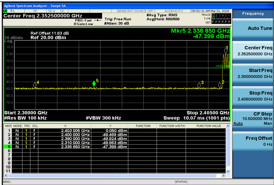
DH5-Ant1-Hop_2402-PASS
