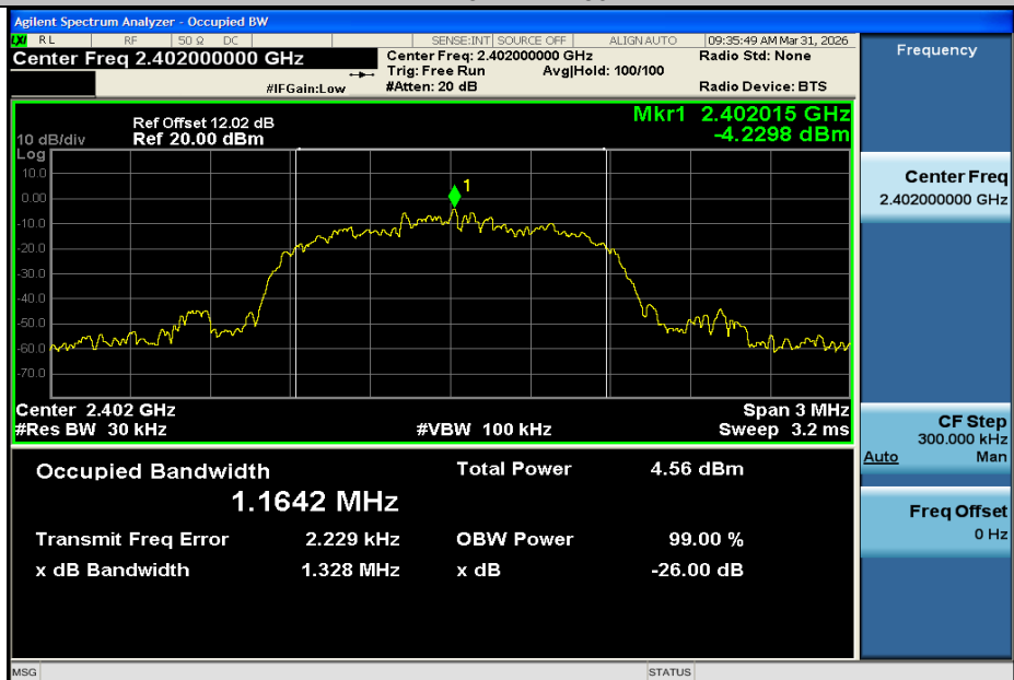
3DH5-Ant1-2402
