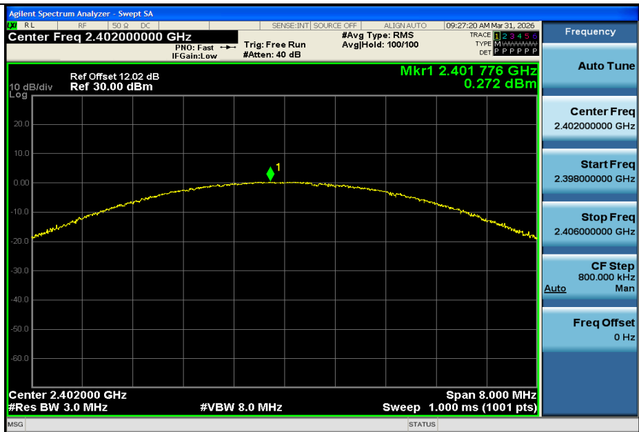
2DH5-Ant1-2402-PASS
