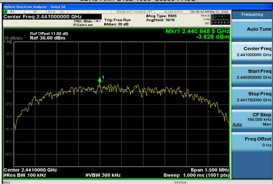
3DH5-Ant1-2441-0~Reference-PASS
