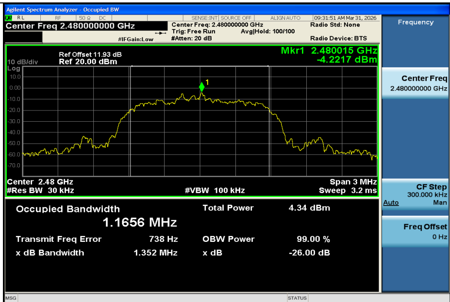
2DH5-Ant1-2480
