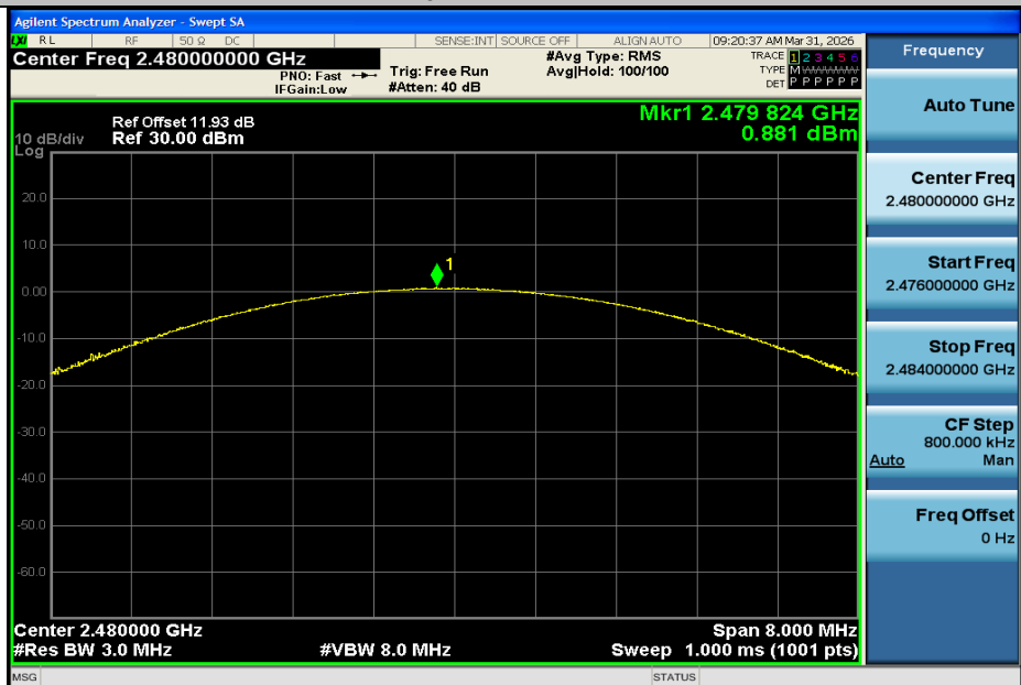
DH5-Ant1-2480-PASS
