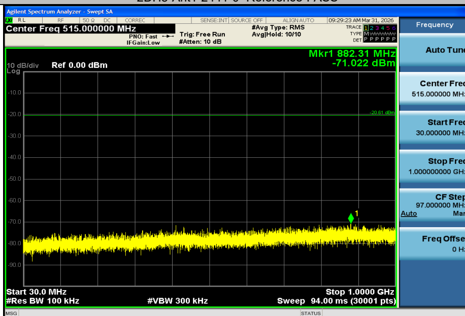
2DH5-Ant1-2441-30~1000-PASS
