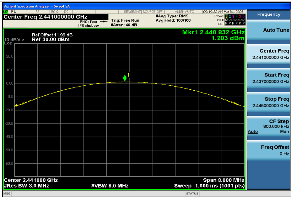
DH5-Ant1-2441-PASS
