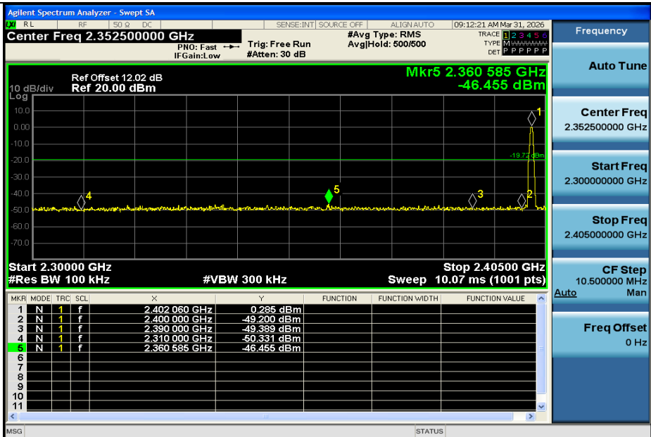
DH5-Ant1-2402-PASS
