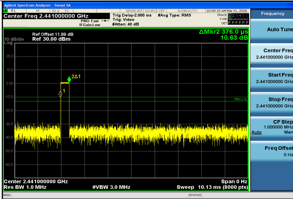
DH1-Ant1-Hop-PASS
