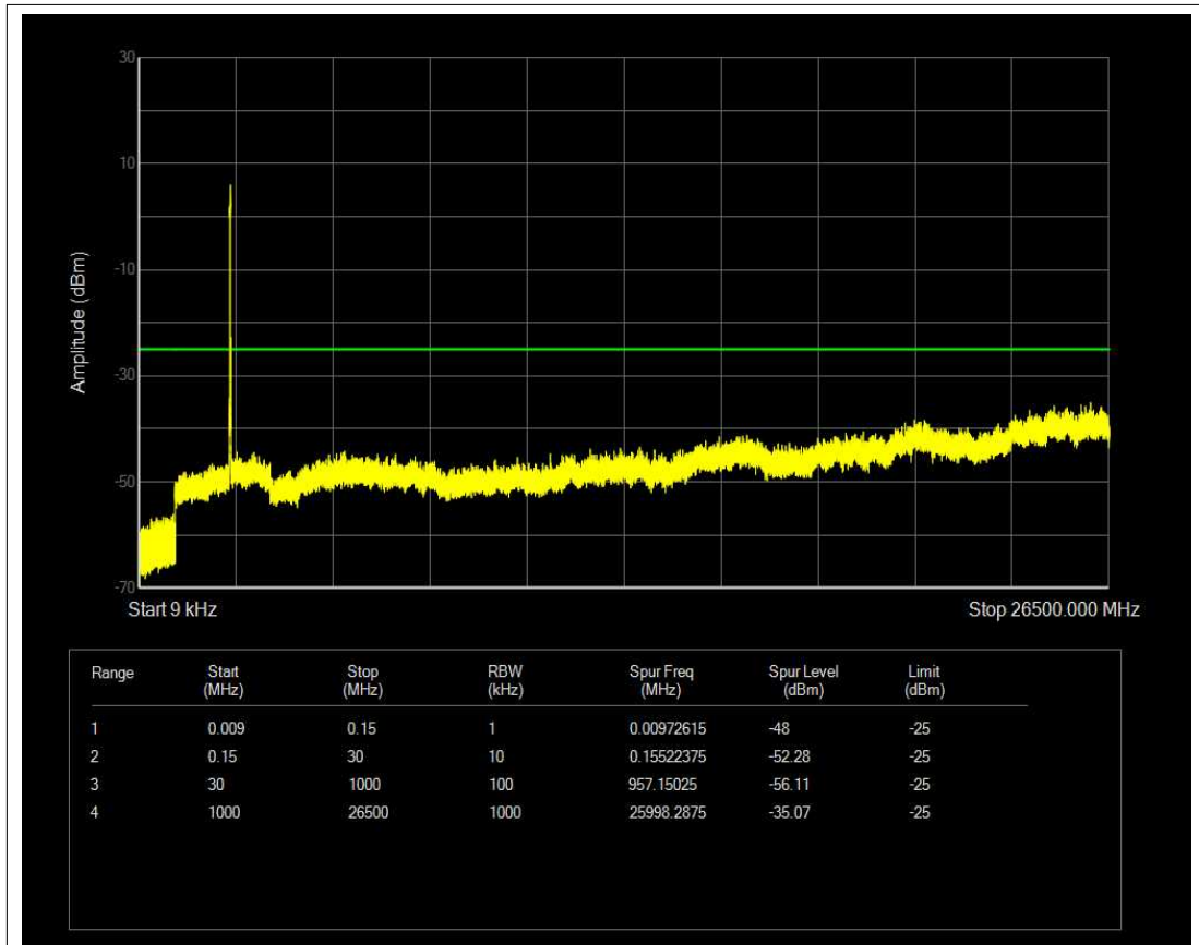
Band41 16QAM BW=20MHz Channel=39750 RB Size=100 Position=#0 NVNT
