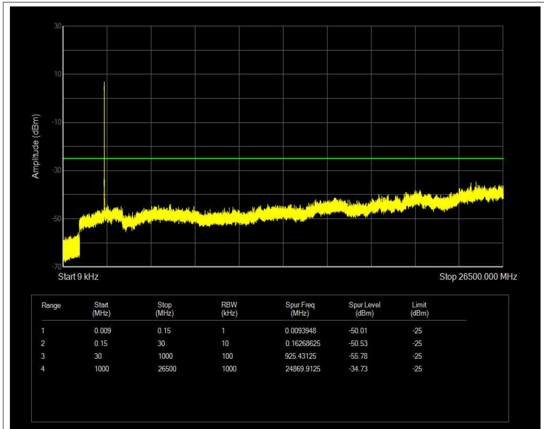
Band41 16QAM BW=10MHz Channel=39700 RB Size=50 Position=#0 NVNT
