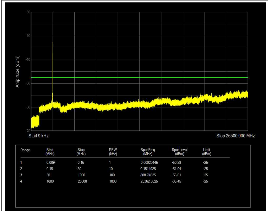
Band41 16QAM BW=20MHz Channel=40620 RB Size=100 Position=#0 NVNT
