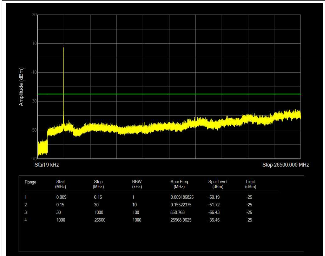
Band41 16QAM BW=10MHz Channel=40620 RB Size=50 Position=#0 NVNT
